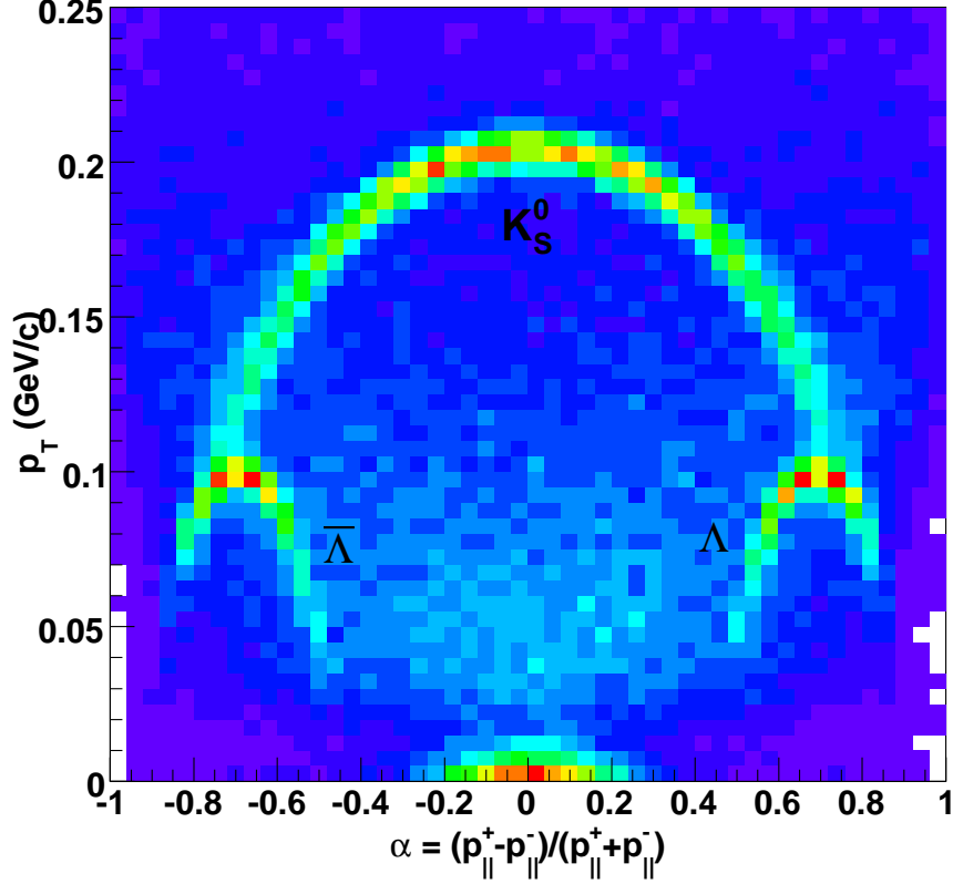
Figure 4.10: Armenteros-Podolanski plot for V0 candidates. p_{\parallel}^+ and p_{\parallel}^- are the momentum components of the positive and negative V0 daughters parallel to the parent V0 momentum direction. p_T is the momentum of each daughter transverse to the parent momentum direction.
