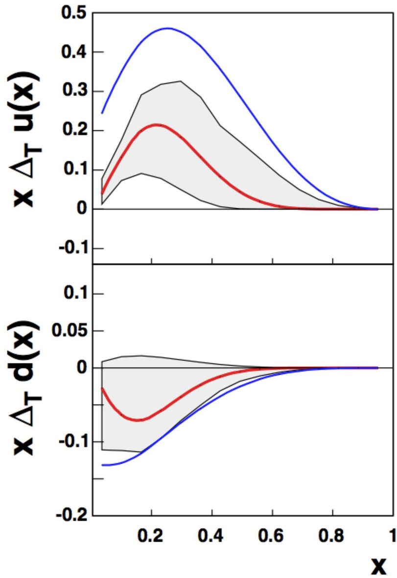
Figure 2.5: Transversity distributions of u and d quarks in the proton extracted from a global fit to data, taken from [88]. The shaded region shows a one-sigma uncertainty around the best-fit distribution. The bold lines outside the shaded region indicate the Soffer bound.
