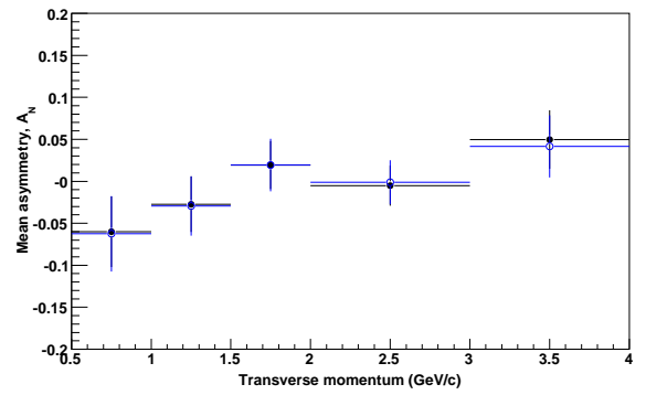
(f) \bar{\Lambda} , forward angles
