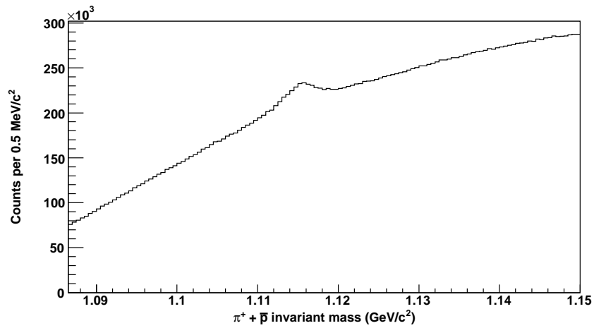
(b) Raw \bar{\Lambda} invariant mass distribution.
