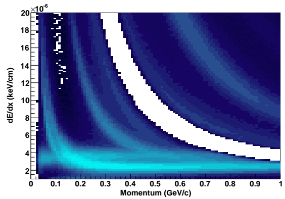
(b) Positive V0 daughters rejected by energy loss selection for protons.
