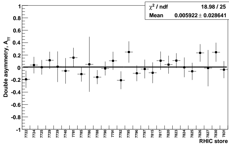
(c) \bar{\Lambda}
