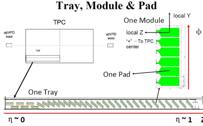
Figure 2.12: TOF geometry for trays, modules and readout pads.
