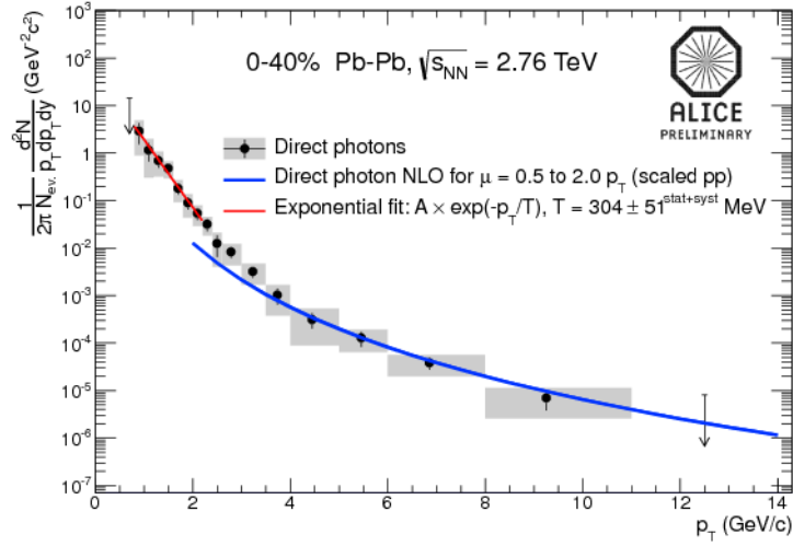
Figure 1.9: Direct photon invariant yield in Pb + Pb collisions at \sqrt{s_{NN}} = 2.76 TeV for 0-40% centrality with NLO pQCD predictions and exponential fit in ALICE. The plots are obtained from [Wil13].
