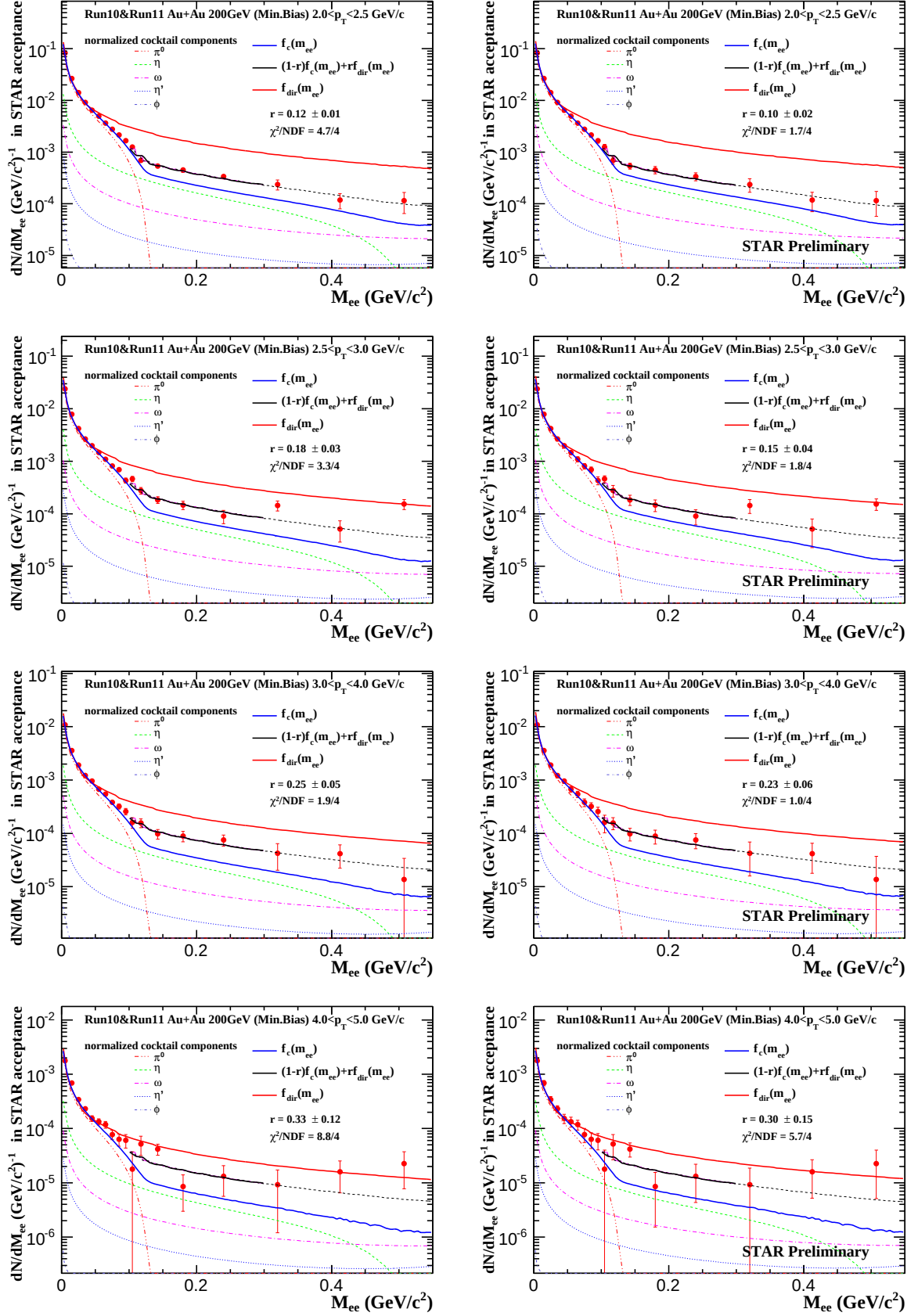
Figure 5.4: The two component function fit on Run10 and Run11 combined Au+Au di-electron continuum in 0.1 < M_{ee} < 0.3 \text{ GeV/c}^2 at 200 GeV. Left panels: w/ statistical errors only. Right panels: w/ errors setting as the quadrature sum of statistical and systematic errors.
