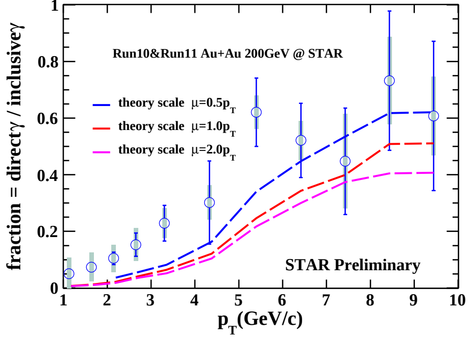
Figure 5.7: The fraction of direct photon compared with the NLO pQCD prediction. The curves represent T_{AA}d\sigma_{\gamma}^{NLO}(p_T)/dN_{\gamma}^{inclusive}(p_T) , showing the scale dependence of the theory [GV93].
