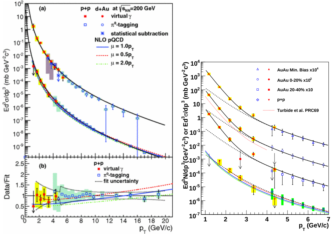
Figure 1.7: The direct photon yields in p+p , d+Au and Au+Au collisions at \sqrt{s(s_{NN})} = 200 \text{ GeV} . Left panel shows the d+Au results compared to p+p results. The figure is obtained from [AAA13]. Right panel shows the Au+Au results. The figure is obtained from [Ada10b].
