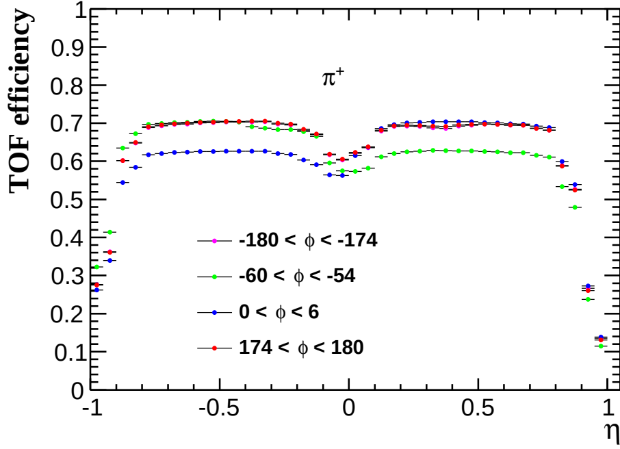
Figure 4.18: \eta and \phi dependence of TOF matching efficiency for Run11 \pi^+
