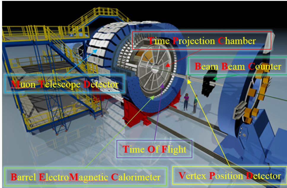
Figure 2.2: Layout of STAR detector.
