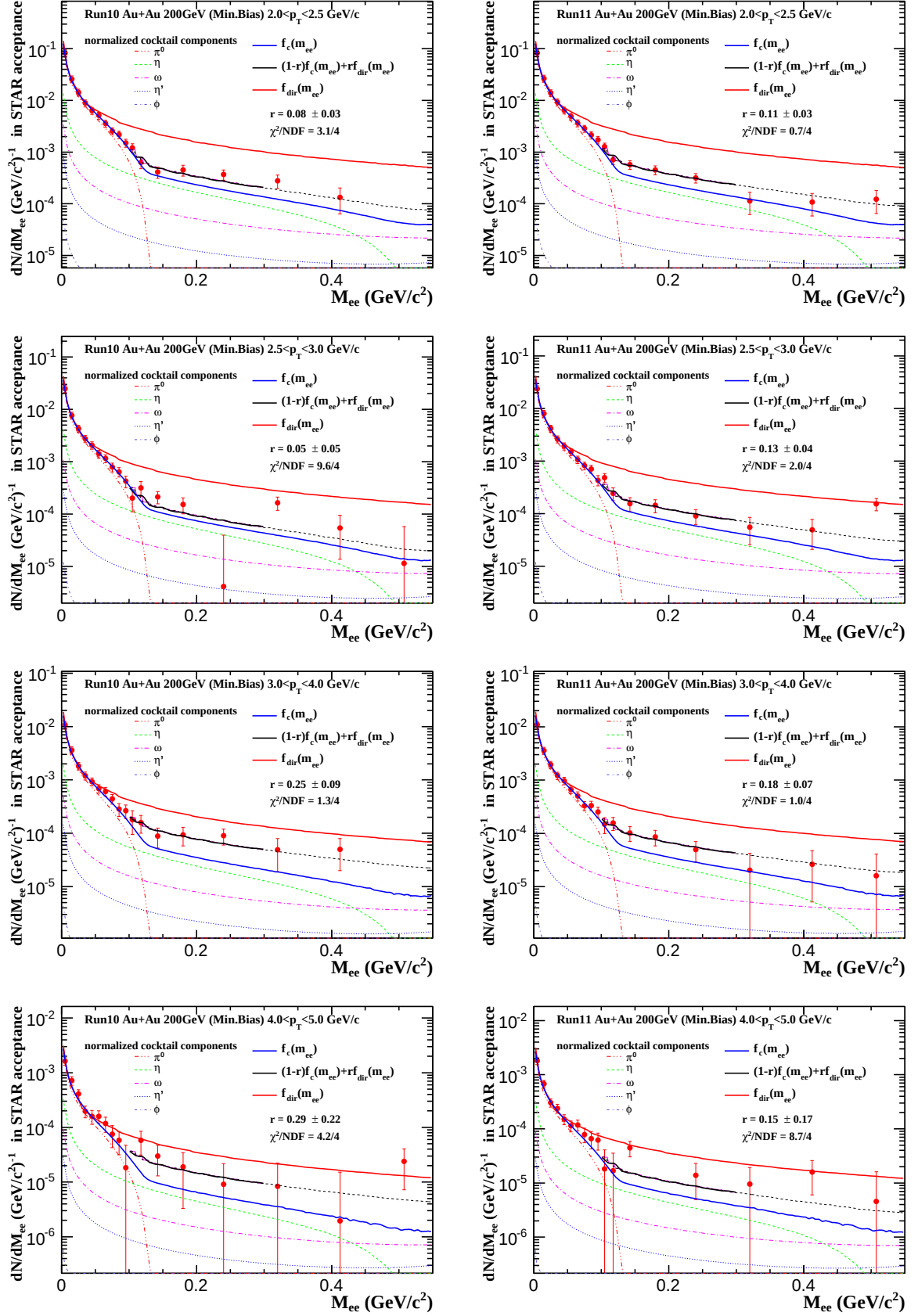
Figure 4.36: The two component function fit on Run10 and Run11 Au+Au di-electron continuum in 0.1 < M_{ee} < 0.3 \text{ GeV}/c^2 at 200GeV.
