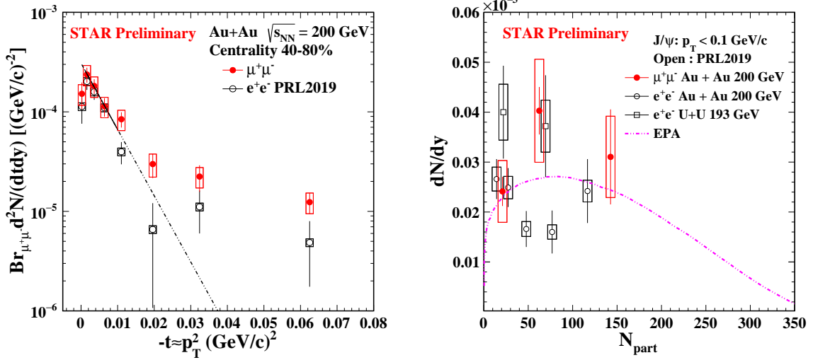
Figure 2: The J/\psi yield as a function of the negative momentum transfer squared -t ( -t \sim p_T^2 ) for the 40%–80% centrality class in Au+Au collisions, in comparison with previous dielectron measurements [7]. The error bars represent the statistical uncertainties, while the boxes represent the systematic uncertainties. The black solid line is an exponential fit to the data points in the range of 0.002–0.015 (\text{GeV}/c)^2 . The dashed black line is an extrapolation of the fit.
