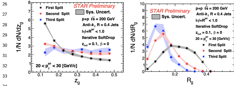
Figure 1 – The momentum fraction, z_g (left), and opening angle between prongs, R_g (right), for first (black), second (red), and third (blue) hard splittings.
