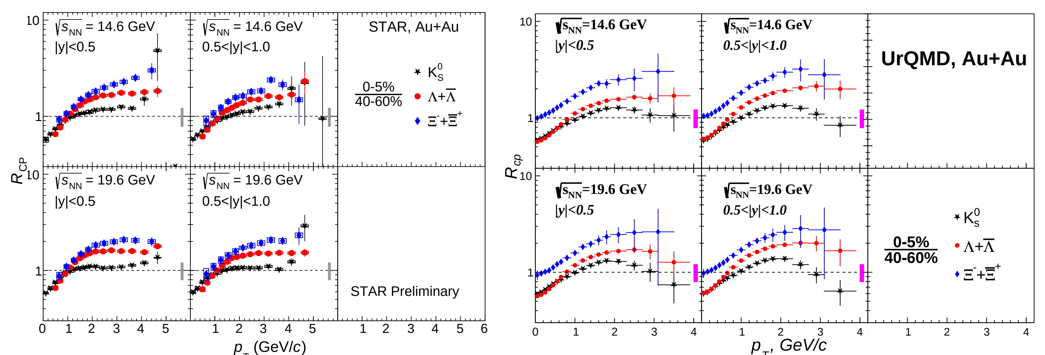
Figure 3: R_{CP} for strange hadrons at \sqrt{s_{NN}} = 14.6 and 19.6 GeV collision energies from STAR BES II (left plot) and UrQMD (right plot).
