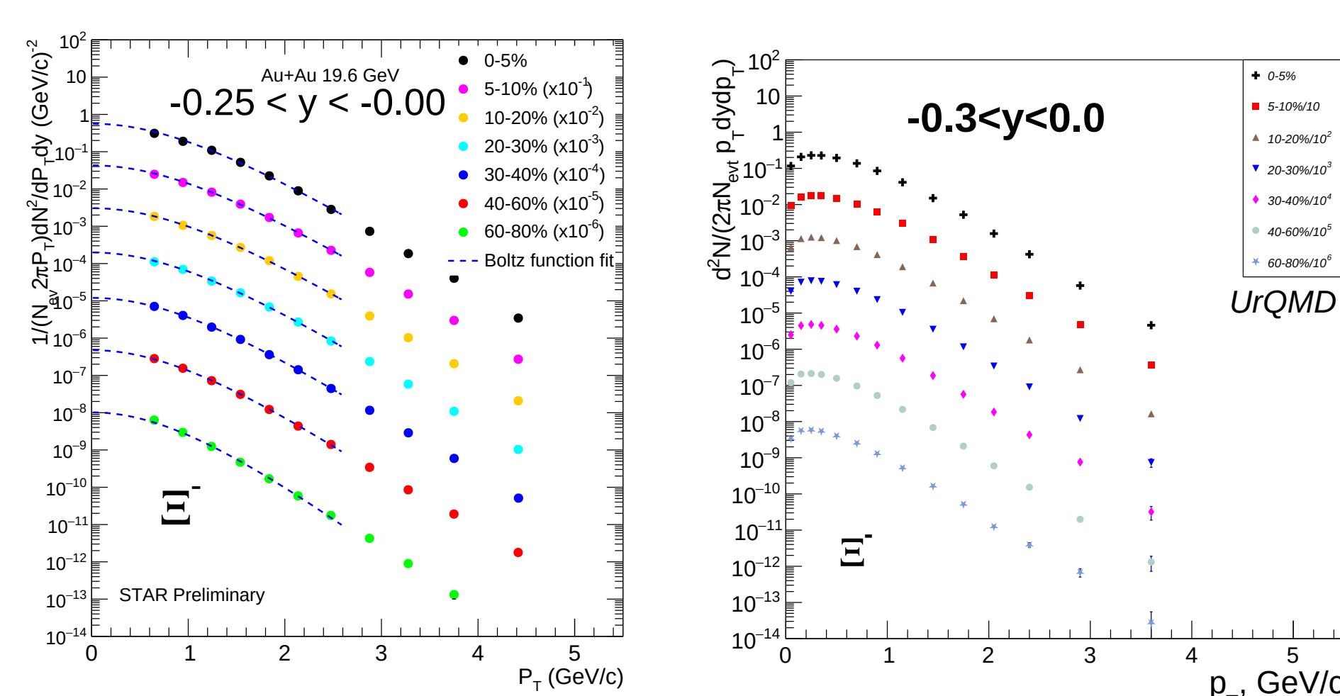
Figure 2: Transverse momentum distribution of \Xi^- for collision energy of 19.6 GeV from STAR BES II (left plot) and UrQMD (right plot). Each spectrum corresponds to a certain centrality class and is multiplied by coefficient from 1 - 10^6 for visibility.
