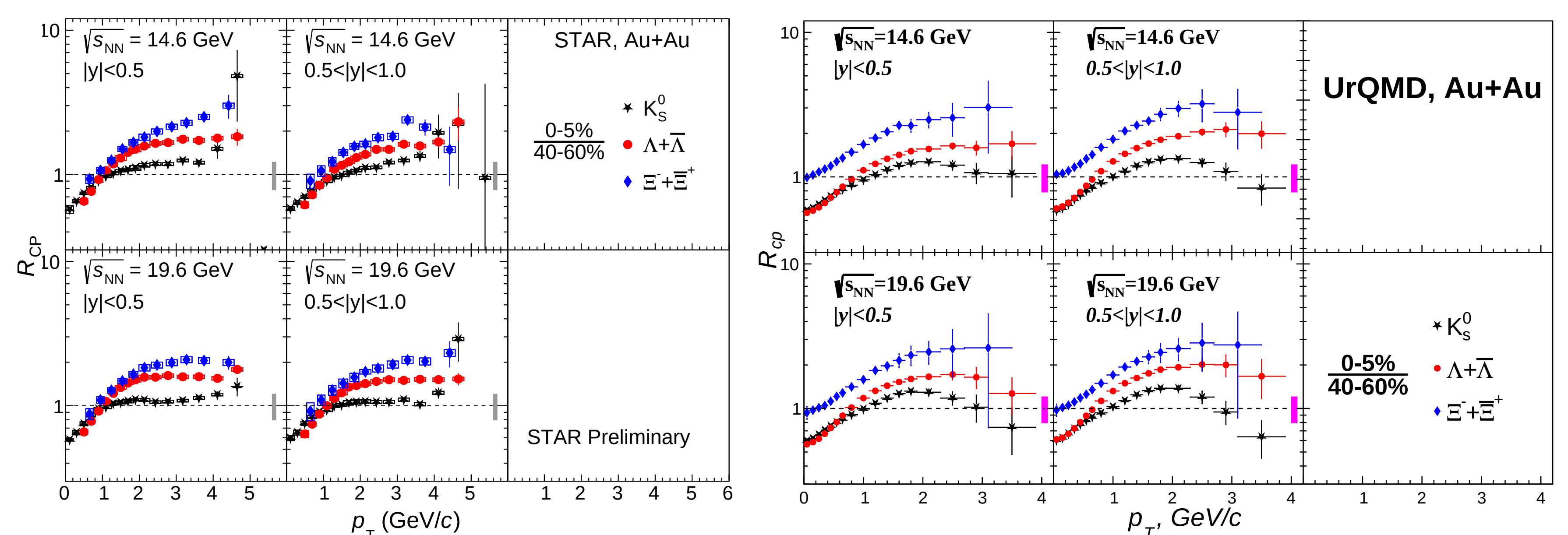
Figure 3: R_{CP} for strange hadrons at \sqrt{s_{NN}} = 14.6 and 19.6 GeV collision energies from STAR BES II (left plot) and UrQMD (right plot).
