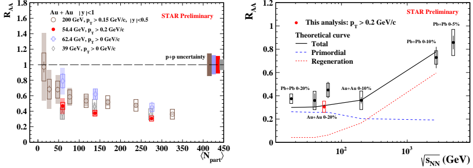
Figure 1: Left panel: The R_{AA} of inclusive J/\psi as a function of \langle N_{part} \rangle in Au+Au collisions at different collision energies at mid-rapidity [5, 6]. The error bars represent the statistical uncertainties. The boxes represent the systematic uncertainties. The shaded bands on the data points indicate the uncertainties from the nuclear overlap function \langle T_{AA} \rangle [15]. The bands around unity indicate the uncertainties from the p+p baselines. Right panel: The R_{AA} of J/\psi as a function of collision energy for central collisions [2–7], in comparison with model calculations [16]. The error bars represent the statistical uncertainties and the boxes represent the systematic uncertainties, including those from p+p baselines and uncertainties from \langle T_{AA} \rangle .
