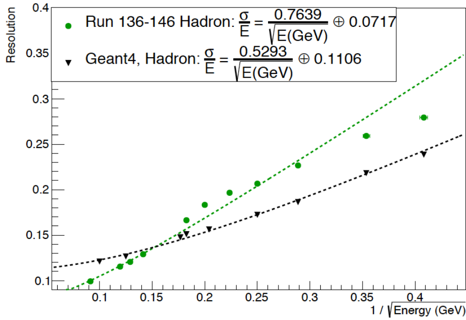
Figure 24. Comparison of experimental and GEANT4 predicted energy resolution
