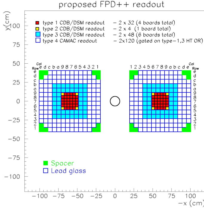
Figure 3.17: Proposed readout electronics for the FPD++.
