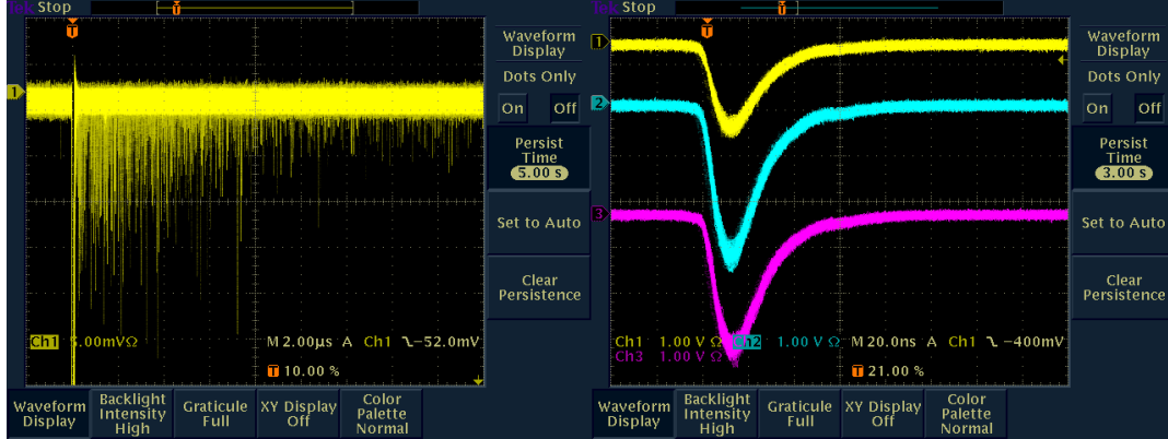
Figure 3.12: XP2202 phototube afterpulse and in-set gain variations. In an average 10 microsecond afterpulse, the afterpulse peak falls to about 1% of the main peak in 2 microseconds. The gain variations on same applied voltages are visible from the right image.
