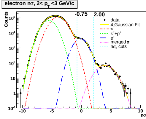
(a) MinBias 2 < p_T < 3 GeV/c
