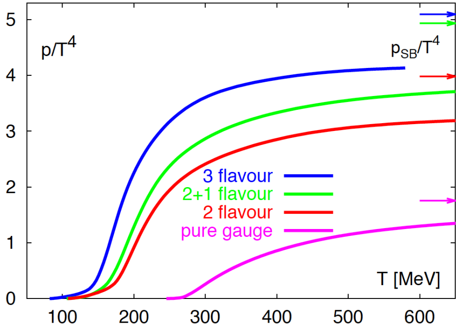
Figure 1.4: A LQCD calculations of pressure as a function of temperature for different treatments of partons. The rapid change in pressure is in response to the change in the active number of degrees of freedom. Figure taken from [10].
