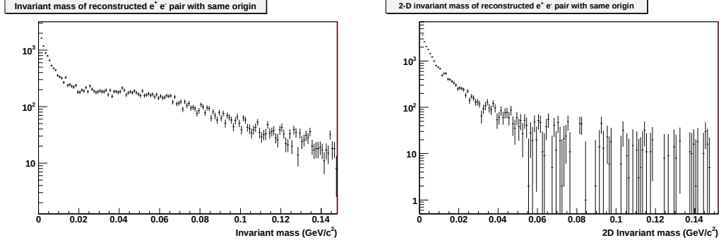
Figure 3.27: Left Plot: The invariant mass of reconstructed e^+ and e^- pairs from the Dalitz decays in simulation. Right Plot: same as the Left Plot, except plotting the 2D invariant mass.
