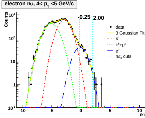
(c) MinBias 4 < p_T < 5 GeV/c
