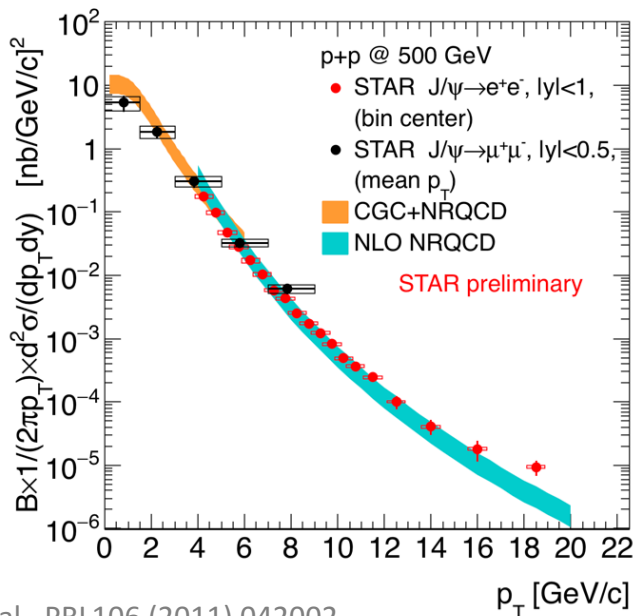
NLO NRQCD: Ma et al., PRL106 (2011) 042002 CGC+NRQCD: Ma, Venugopalan, PRL113 (2014) 192301
