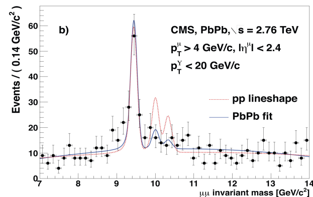
CMS Collaboration, Phys Rev Lett 107 052302, 2011
