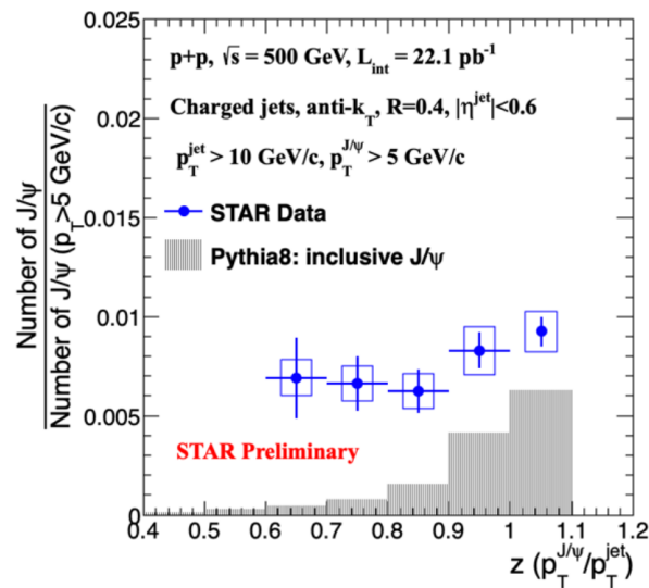
Figure 4. The normalized z distributions for inclusive J/\psi mesons produced within a jet in p + p collisions at \sqrt{s} = 500 GeV compared to prediction from PYTHIA 8. The data are normalized by the J/\psi cross-section at the same collision energy [20].
