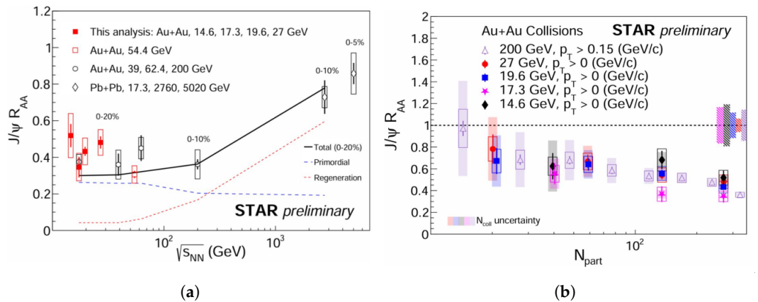
Figure 1. (a) J/\psi R_{AA} as a function of collision energy with data from the STAR experiment \sqrt{s_{NN}} = 14.6 - 200 GeV in Au+Au collisions [7,8], compared with SPS and ALICE measurements [9–11] and model predictions [12,13]. (b) Measurement of the J/\psi R_{AA} as a function of centrality in Au+Au collisions for various collision energies at the STAR experiment.
