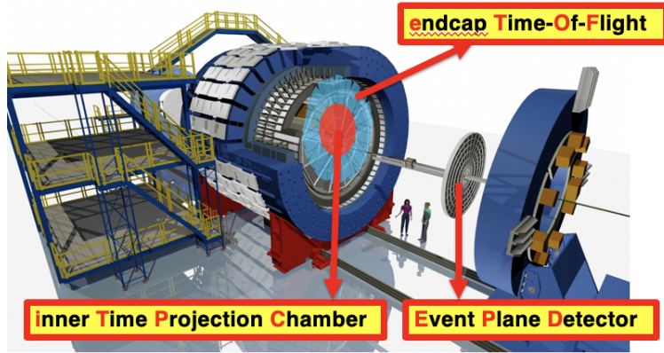
Figure 1. The layout of STAR detector upgrades for RHIC BES-II program.
