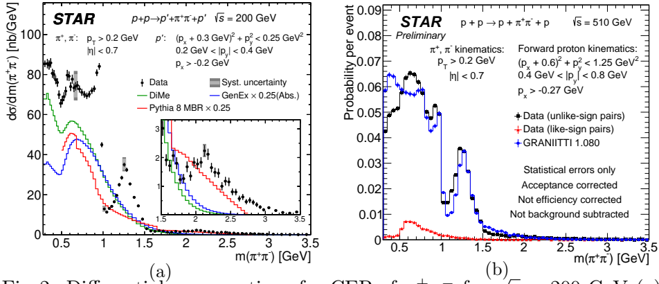
Fig. 2: Differential cross sections for CEP of \pi^+\pi^- for \sqrt{s} = 200 GeV (a) as a function of the invariant mass of the pair, measured in the fiducial region explained on the plots. Data are shown as solid points with error bars representing the statistical uncertainties. The typical systematic uncertainties are shown as grey boxes for only a few data points as they are almost fully correlated between neighbouring bins. Predictions from Monte Carlo models GenEx, DiMe and MBR are shown as histograms. Efficiency uncorrected, preliminary distribution of the invariant mass of the pair for \sqrt{s} = 510 GeV (b) together with distribution for like-sign pairs. Prediction from Monte Carlo model Graniitti is shown as histogram. Both data and MC prediction are normalised to unity.
