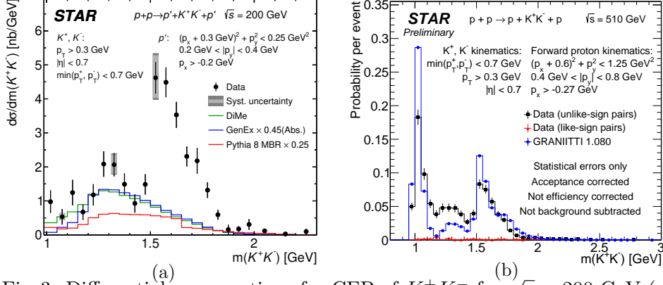
Fig. 3: Differential cross sections for CEP of K^+K^- for \sqrt{s} = 200 GeV (a) as a function of the invariant mass of the pair, measured in the fiducial region explained on the plots. Data are shown as solid points with error bars representing the statistical uncertainties. The typical systematic uncertainties are shown as grey boxes for only a few data points as they are almost fully correlated between neighbouring bins. Predictions from Monte Carlo models GenEx, DiMe and MBR are shown as histograms. Efficiency uncorrected, preliminary distribution of the invariant mass of the pair for \sqrt{s} = 510 GeV (b) together with distribution for like-sign pairs. Prediction from Monte Carlo model Graniitti is shown as histogram. Both data and MC prediction are normalised to unity.
