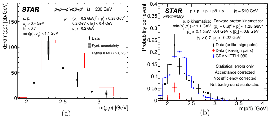
Fig. 4: Differential cross sections for CEP of p\bar{p} for \sqrt{s} = 200 GeV (a) as a function of the invariant mass of the pair, measured in the fiducial region explained on the plots. Data are shown as solid points with error bars representing the statistical uncertainties. The typical systematic uncertainties are shown as grey boxes for only a few data points as they are almost fully correlated between neighbouring bins. Prediction from Monte Carlo model MBR is shown as histogram. Efficiency uncorrected, preliminary distribution of the invariant mass of the pair for \sqrt{s} = 510 GeV (b) together with distribution for like-sign pairs. Prediction from Monte Carlo model Graniitti is shown as histogram. Both data and MC prediction are normalised to unity.
