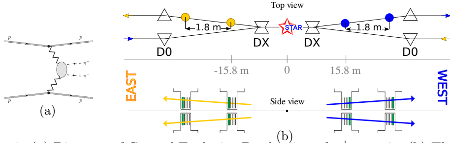
Fig. 1: (a) Diagram of Central Exclusive Production of \pi^+\pi^- pair. (b) The layout of the Roman Pot (RP) system at STAR. Two sets of RPs, were installed between the DX and D0 magnets, at 15.8 m and 17.6 m, on either side of the Interaction Point. Arrows in the bottom part of the Figure demonstrate combinations of RPs forming four branches, in which proton tracks can be reconstructed.
