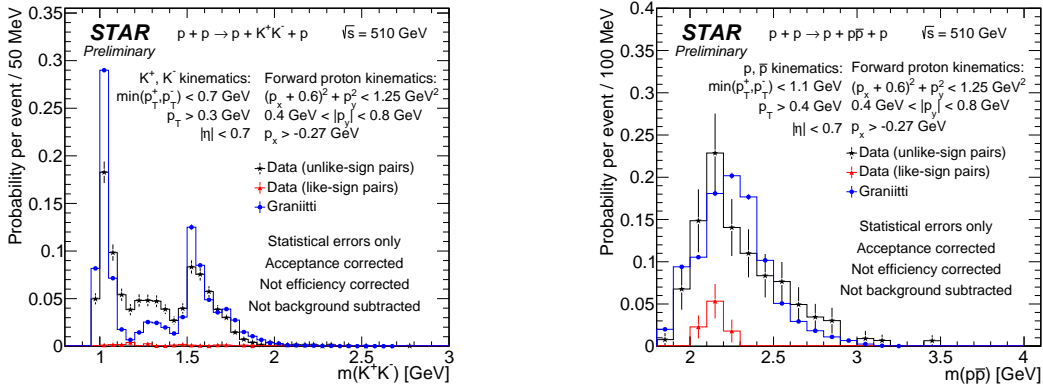
Figure 3: The acceptance corrected invariant mass spectrum of exclusively produced K^+ K^- pairs (left) and p \bar{p} pairs (right). Results are compared with a new tune of GRANIITTI [4]. Error bars represent the statistical uncertainties.
