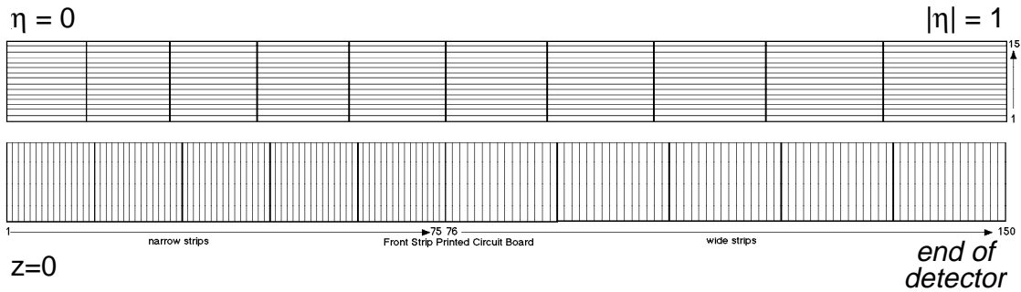
Figure 18: This figure shows the layout of the printed circuit. The top shows the \phi -strips and bottom shows the \eta -strips. Note, the two sizes of strips for the \eta -strips.
