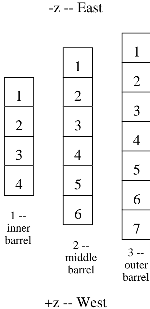
Figure 9: Numbering scheme for the wafers on the SVT ladder.
