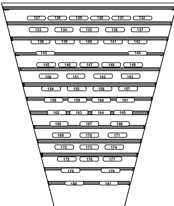
Figure 12: Representation of an inner sector of the TPC. The numbering of the FEE cards is shown.
