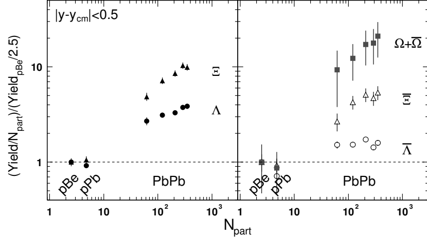
Figure 1.15: Strange particle yields scaled by N_{\text{part}} normalized by p-Be collisions [Fan02].
