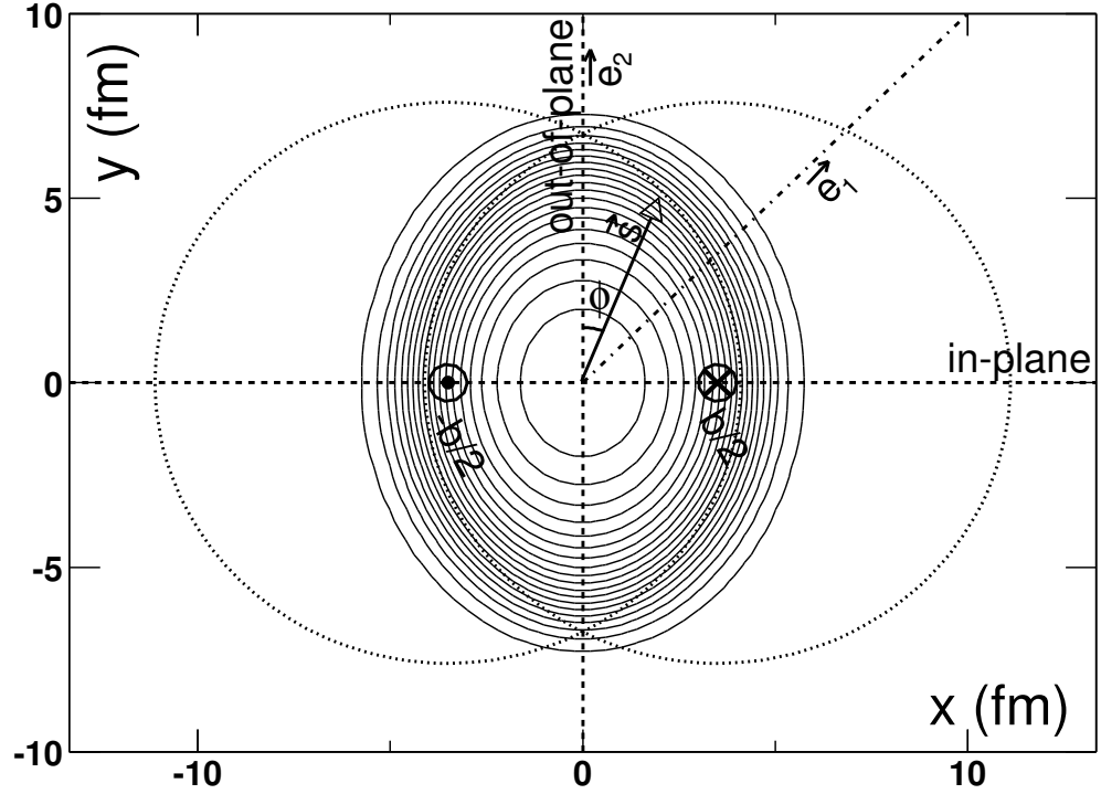
Figure A.1: Coordinate system for the transverse plane in heavy-ion collisions. Contours of the overlap density are also shown. Here \phi is the azimuthal angle with respect to the y -axis. Also shown are generalized coordinates \vec{e}_1 and \vec{e}_2 used to calculate the fourth-harmonic eccentricity where the (y-)e_2 -axis is the only uniquely defined direction in the transverse plane.
