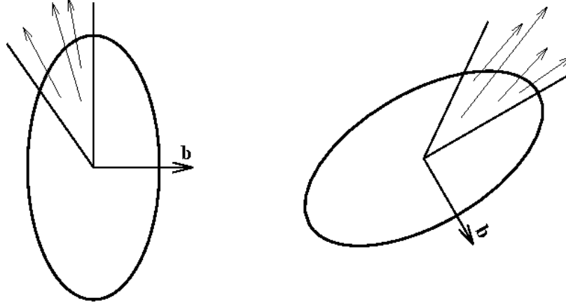
Figure 4.12: Example of two events with different laboratory event plane angles. The arrows represent particles accepted into a \Phi_{rp} correlation function.
