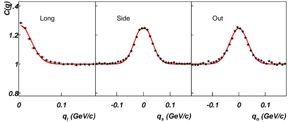
Figure 4.4: Bertsch-Pratt projections for an analysis with no vertex binning but a tighter cut on vertex position. The event vertices vary from -35 < z_{vtx} < 35cm with a cut on rapidity of -1 < y < 1 . Of note is the reduced slope in q_l improving the agreement between the data and the Gaussian fit (red line) when compared to Fig. 4.3.
