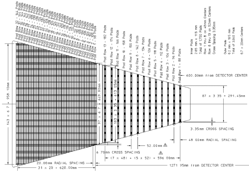
Figure 3.4: The pad layout for a sector of the TPC in STAR.
