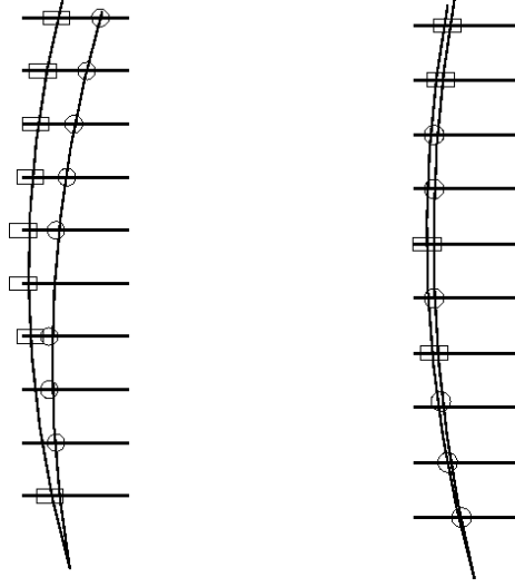
Figure 4.14: Examples of how the topology map is used to identify split tracks. Closed squares and open circles represent separate reconstructed tracks. On the left are two separate tracks while on the right is a likely split track candidate.
