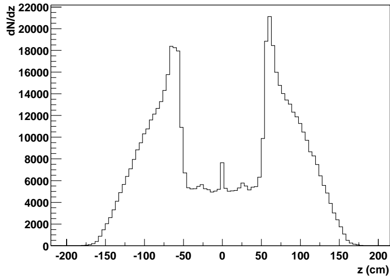
Figure 4.9: “Z” distribution of photon conversion points serving as an indicator of the amount of material between the emission region and the detector [54].
