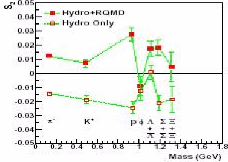
Figure 1.4: The mean spatial anisotropy s'_2 as a function of particle mass with and without the RQMD hadronic after-burner [7].
