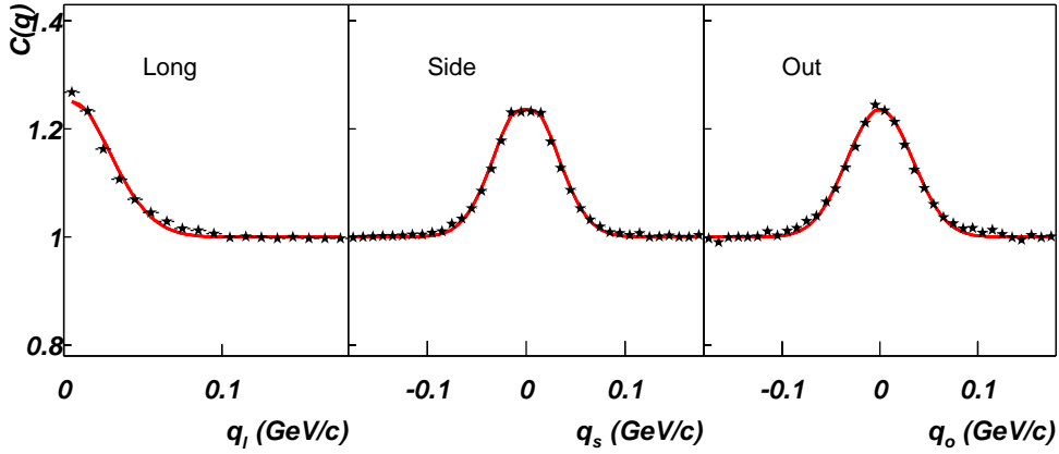
Figure 4.6: Bertsch-Pratt projections for an analysis with 10 cm vertex binning. The event vertices vary from -75 < z_{vtx} < 75\text{cm} with a rapidity cut of -1 < y < 1 . Of note is the reduced slope in q_l improving the agreement between the data and the Gaussian fit (red line) when compared to Fig. 4.3.
