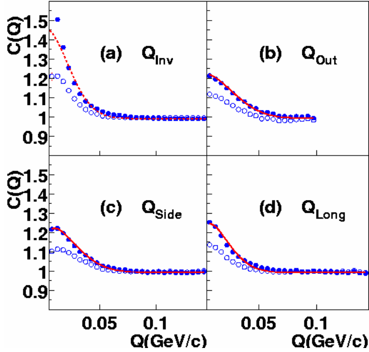
Figure 2.2: 1D ( q_{inv} ) histogram and 1D projections of Pratt–Bertsch parameterization correlation functions for \sqrt{s_{NN}} = 130\text{GeV} Au + Au collisions. Shown are histograms for both uncorrected (open circles) and Coulomb corrected (closed circles) with Gaussian source fits to the corrected data (lines) [23].
