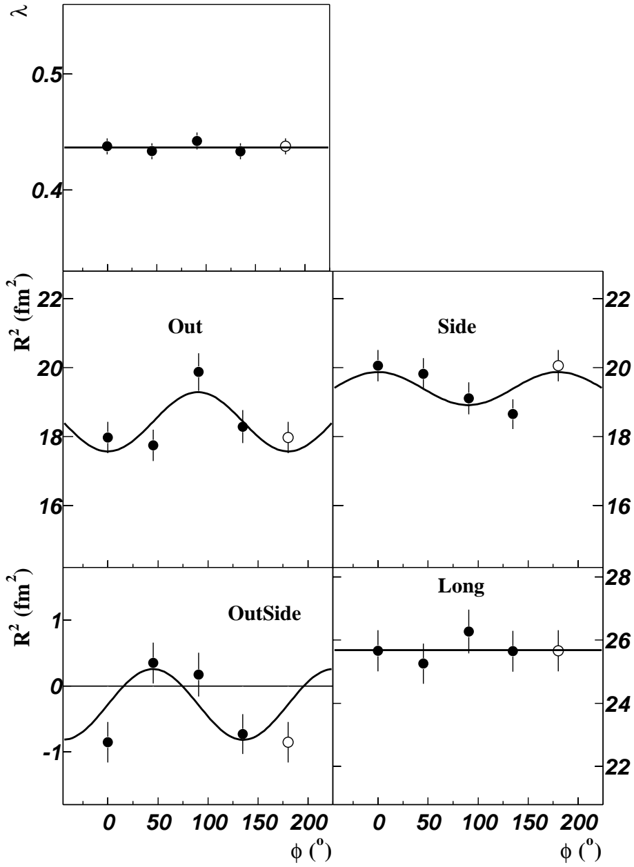
Figure 5.3: \pi^-\pi^- RP HBT parameters with sinusoidal fits to transverse radii and linear fits to \lambda and R_l^2 .
