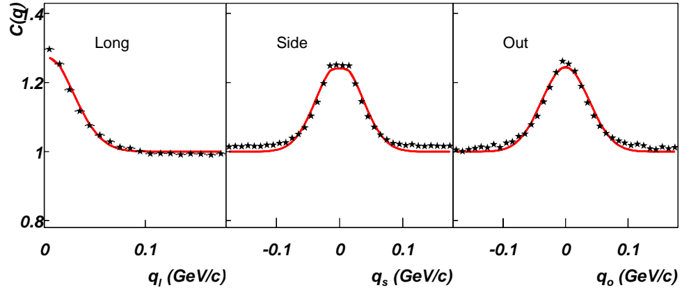
Figure 4.3: Bertsch-Pratt projections for an analysis with no vertex binning. The event vertices vary from -75 < z_{vtx} < 75cm with a cut on rapidity -1 < y < 1 . Of note is the slope in q_l which forces the normalization lower. This is evident in the offset between the data (black stars) and the fit (red line) in q_o and q_s .
