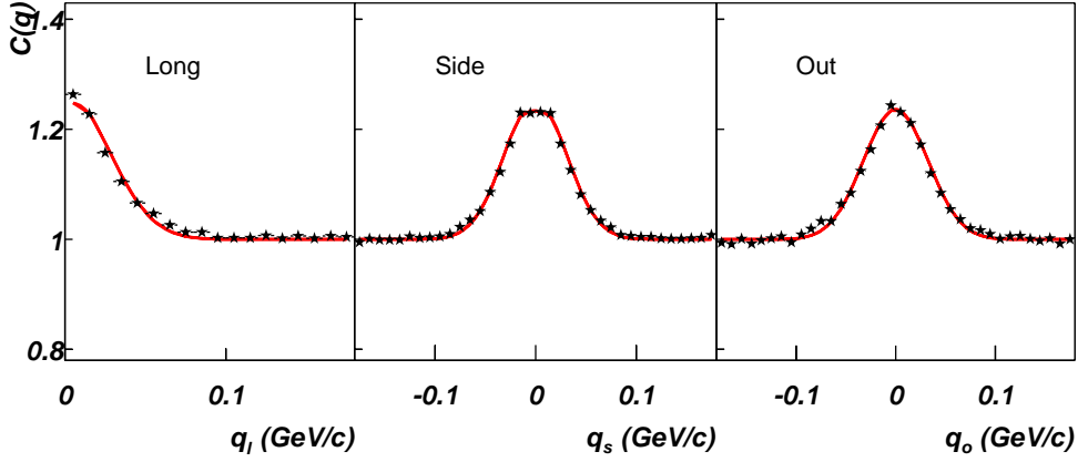
Figure 4.5: Bertsch-Pratt projections for an analysis with no vertex binning but a tighter cut on track rapidity. The event vertices vary from -75 < z_{vtx} < 75\text{cm} while the rapidity cut is -0.5 < y < 0.5 . Of note is the reduced slope in q_l improving the agreement between the data and the Gaussian fit (red line) when compared to Fig. 4.3.
