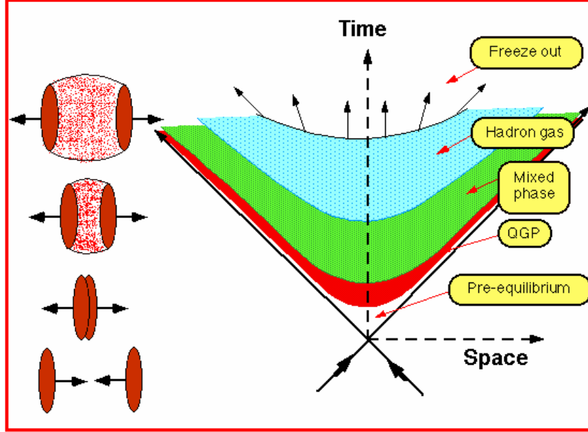
Figure 1.2: Theoretical evolution of a heavy ion collisions.
