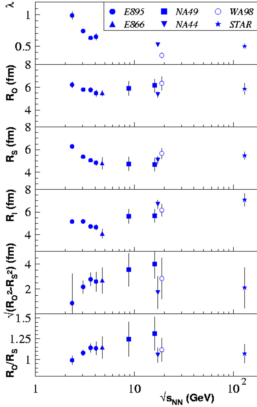
Figure 2.5: The energy dependence of midrapidity \pi^- HBT radii from central Au + Au or Pb + Pb collisions at p_T \sim 0.17 \text{ GeV}/c [25, 26, 27, 28].
