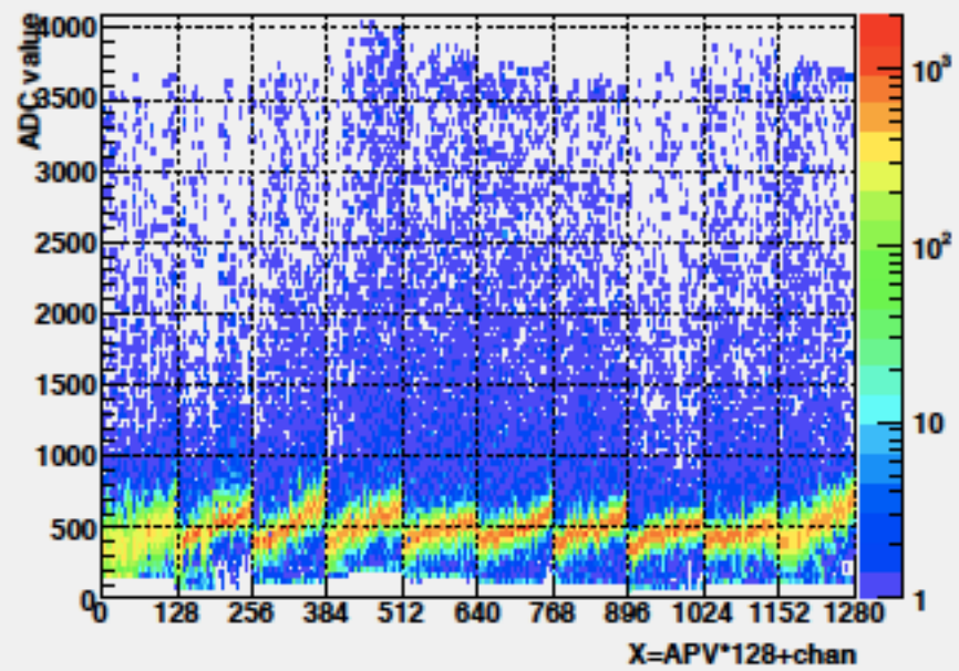
Assembly 6BC with RDO:2, ARM:3, group:1
