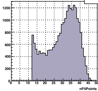
prim tr nFitP, TPC sec=10
