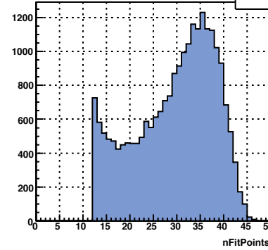
prim tr nFitP, TPC sec=12
