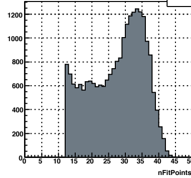
prim tr nFitP, TPC sec=11
