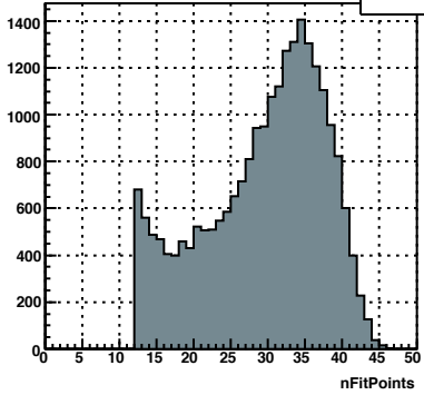
prim tr nFitP, TPC sec=9
