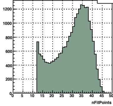
prim tr nFitP, TPC sec=6
