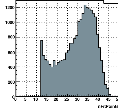
prim tr nFitP, TPC sec=8
