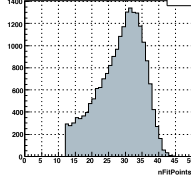
prim tr nFitP, TPC sec=7
