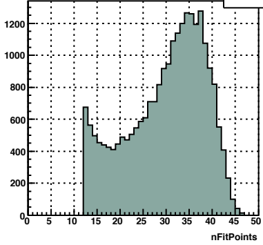
prim tr nFitP, TPC sec=5
