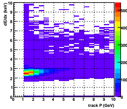
dEdX vs. P, acctpd , TPC sec=20
