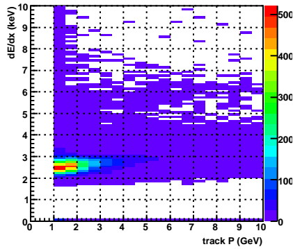
dEdX vs. P, acctpd , TPC sec=18
