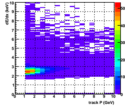
dEdX vs. P, accepted, TPC sec=12
