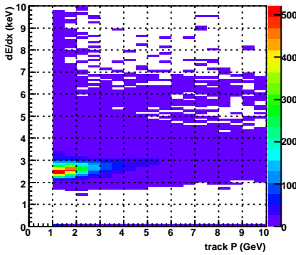
dEdX vs. P, acctpd , TPC sec=17
