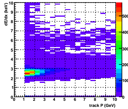
dEdX vs. P, acctpd , TPC sec=19
