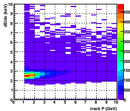
dEdX vs. P, acctpd , TPC sec=24
