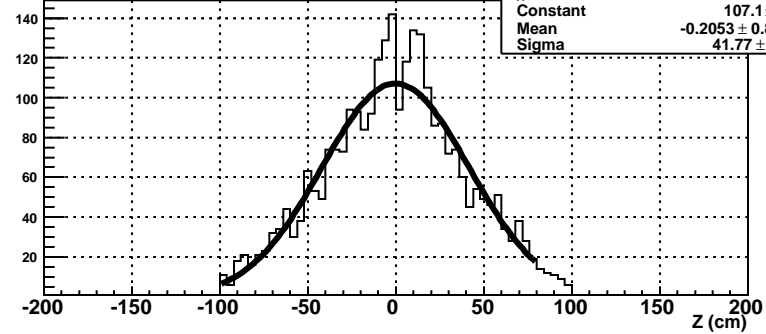
Barrel W: Vertex Z, final selection, 2x2 ET>25 GeV
