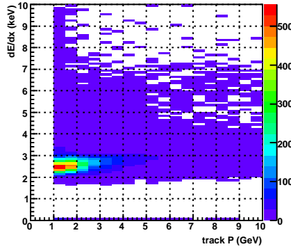
dEdX vs. P, accepted, TPC sec=6
