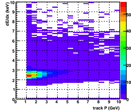
dEdX vs. P, accepted, TPC sec=8
