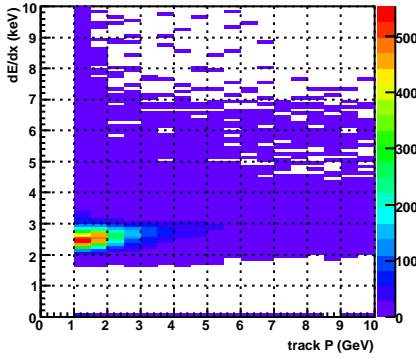
dEdX vs. P, accepted, TPC sec=5
