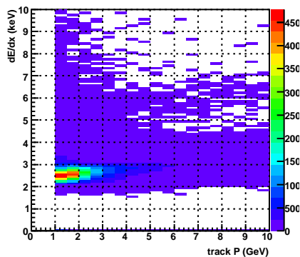
dEdX vs. P, acctpd , TPC sec=22
