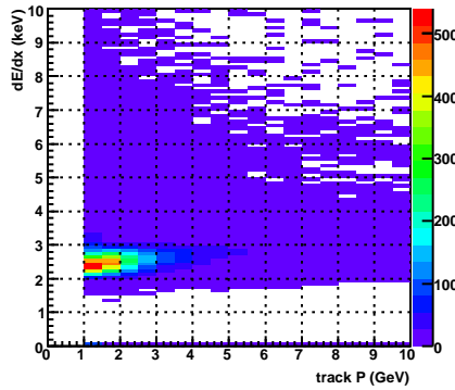
dEdX vs. P, accepted, TPC sec=10
