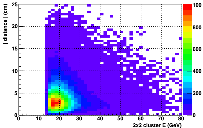
Barrel: R\Delta\phi (track-cluster) vs. 2x2 E Entries 81163
