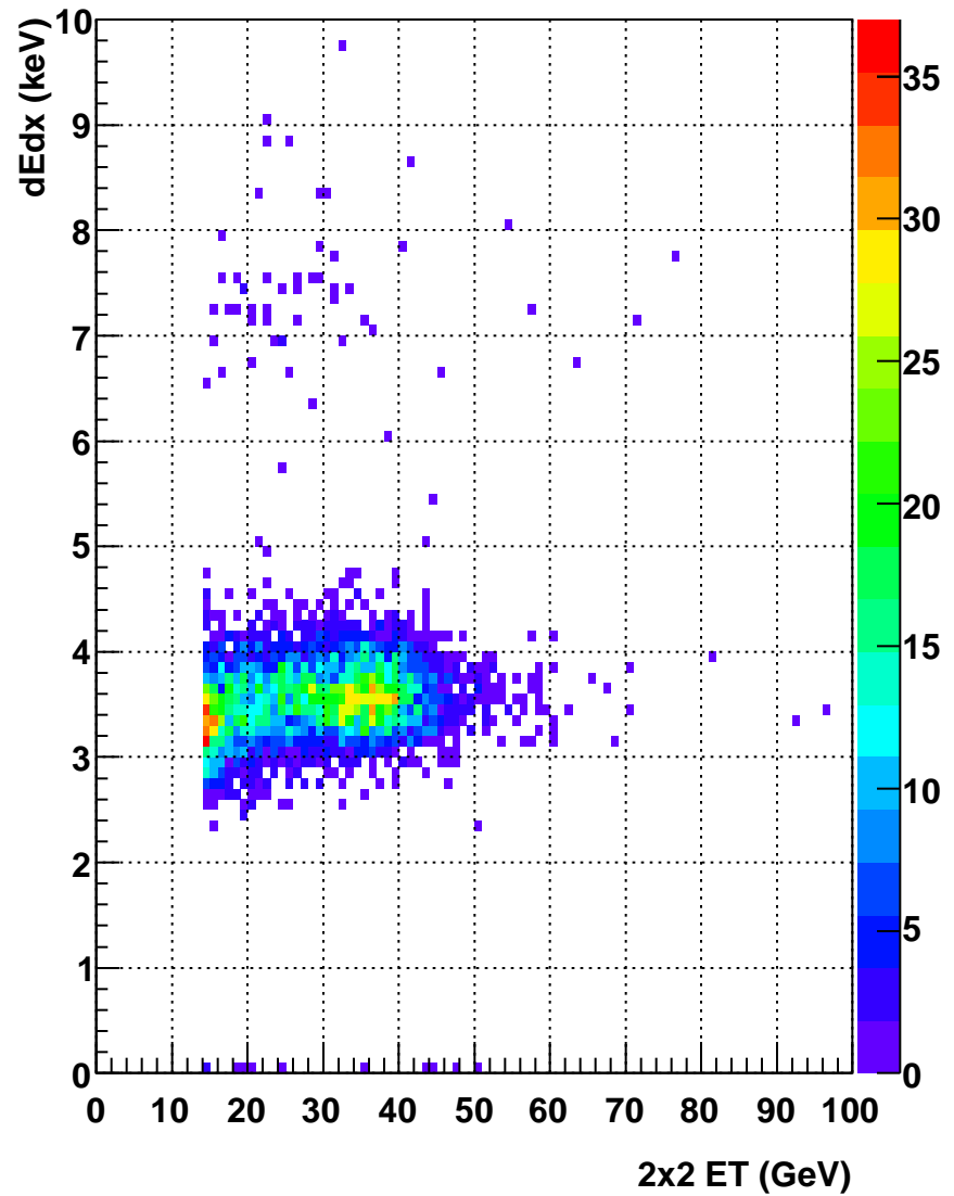
Barrel W: Track dEdx, final selection
