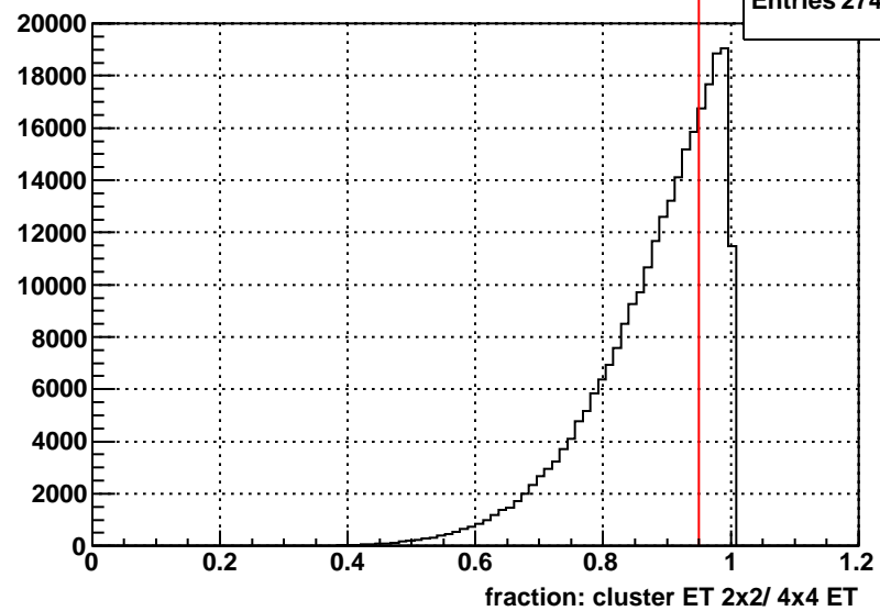
Barrel: ratio (2x2/4x4) cluster ET
