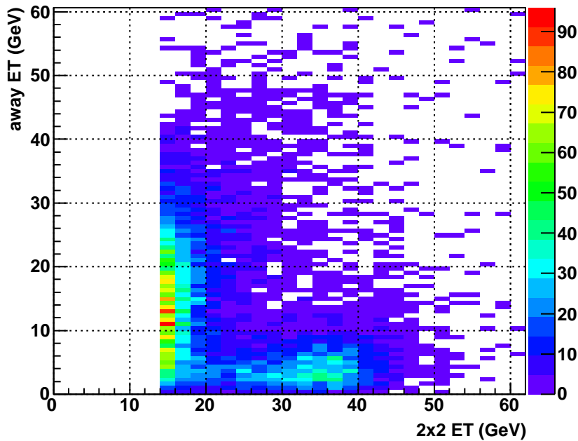
Barrel W: Final Selection : 2011Walgo
