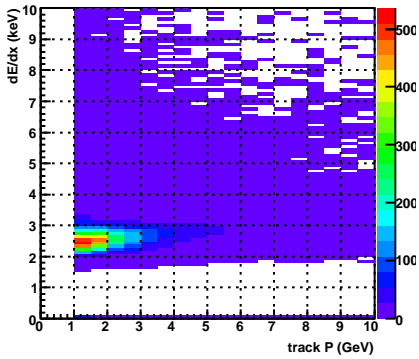
dEdX vs. P, accepted, TPC sec=9
