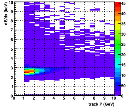
dEdX vs. P, accepted, TPC sec=7
