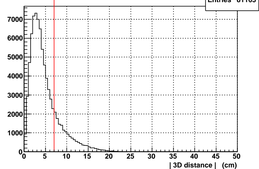
Barrel: 3D Distance(track-cluster) vs. 2x2 E Entries 81163
