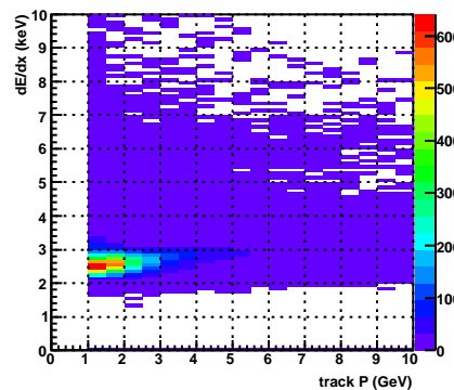
dEdX vs. P, accepted, TPC sec=11
