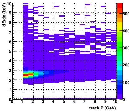
dEdX vs. P, acctpd , TPC sec=21
