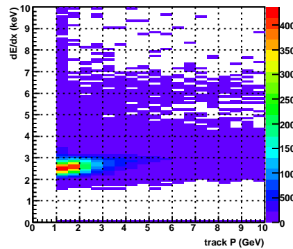
dEdX vs. P, acctpd , TPC sec=23
