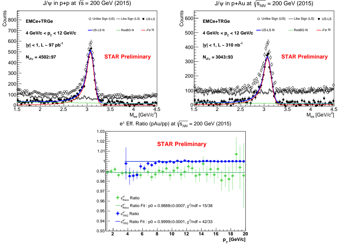
Figure 1: Top left and right: J/\psi yield extraction for p+p and p+Au collisions achieved by fitting the invariant mass distribution to a Crystal Ball function with an exponential background. Open circle: unlike-sign (US) pairs; black histogram: like-sign (LS) pairs; solid circle: unlike-sign minus like-sign (US-LS) pairs; blue line: fitted US-LS; red line: J/\psi signal from fit; green line: residual background from fit. Bottom: Electron detection efficiency ratio (green circle, fitted with green line) and triggering efficiency ratio (blue circle, fitted with blue line) between p+Au and p+p systems, studied with J/\psi embedded into real data.
