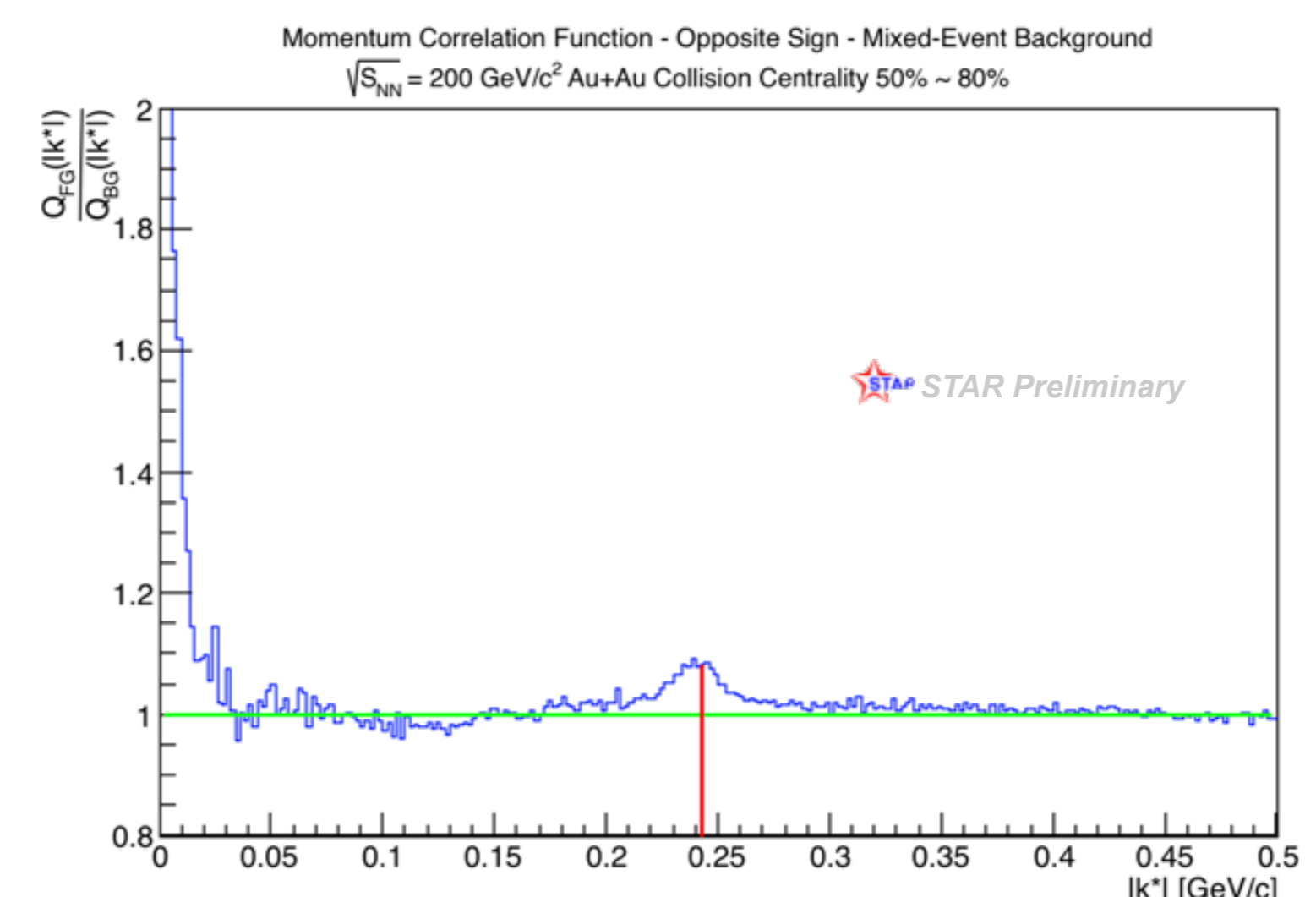
Figure 4. Signal of momentum correlation function for opposite sign particles.
