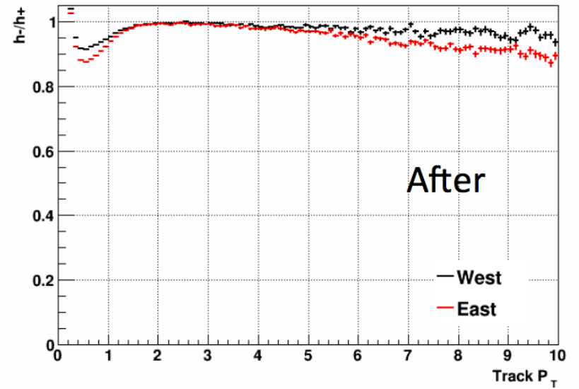
Run 13 Primary After
