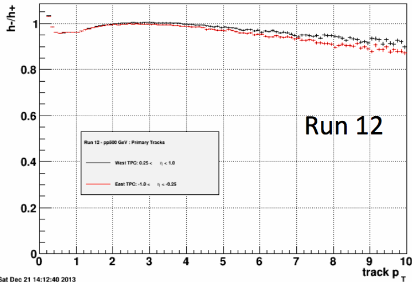
h-/h+ vs track p T : Primary Tracks
