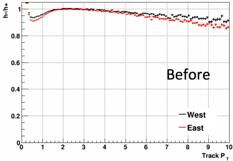
Run 13 Primary Before
