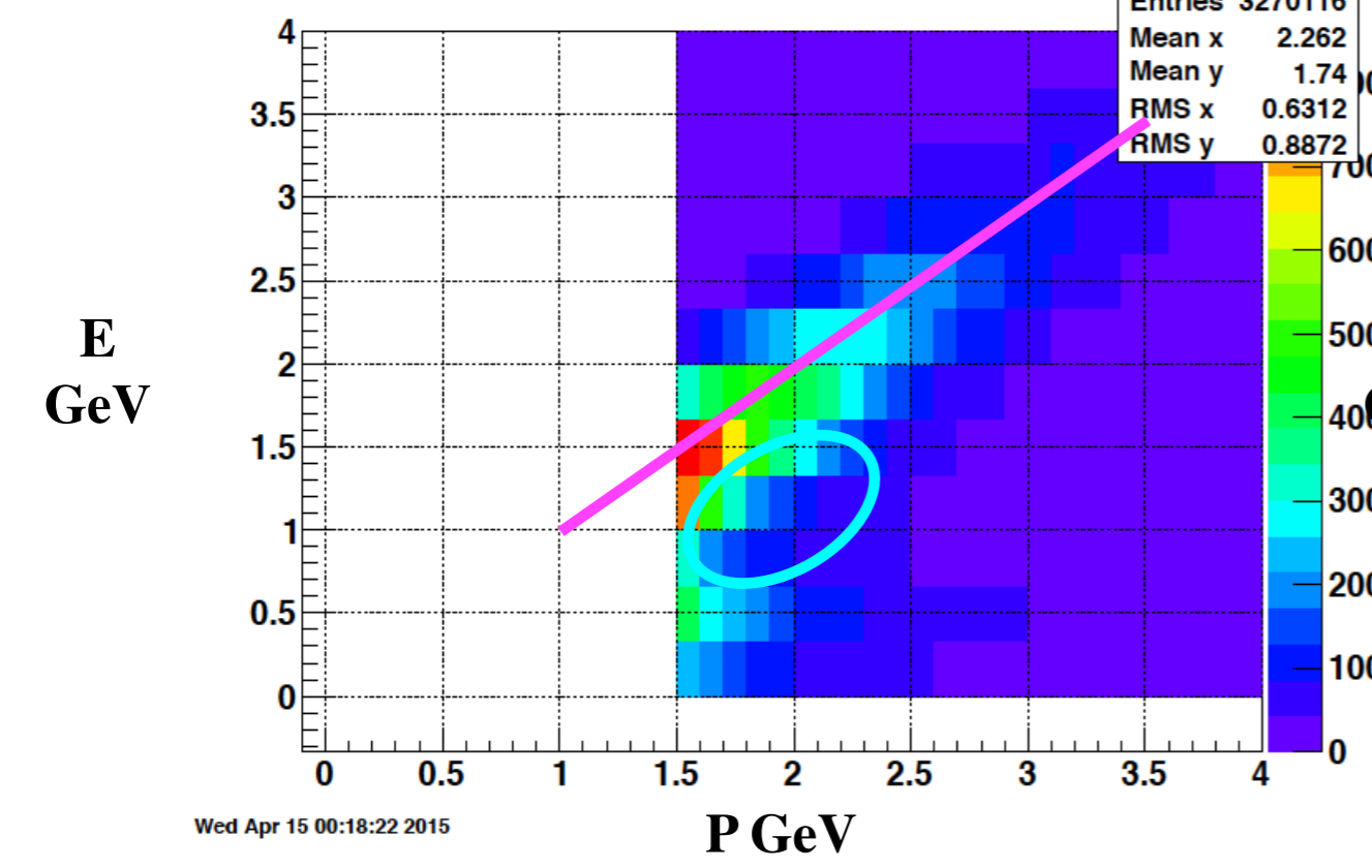
Evsp_Unbiased
