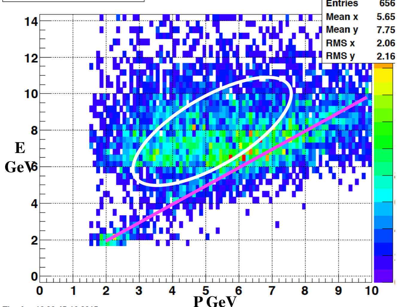
Evsp_Unbiased
