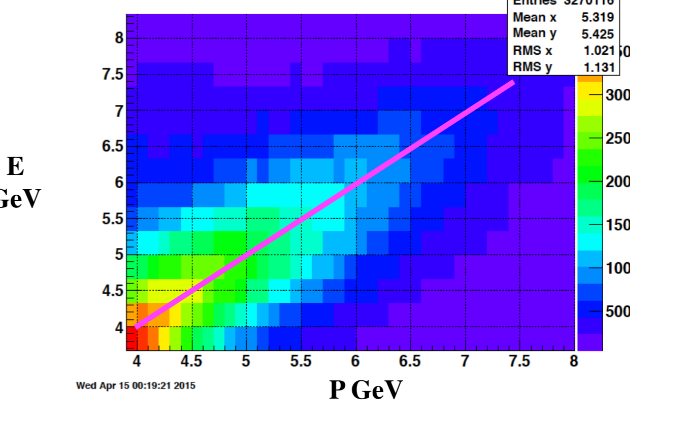
Evsp_Unbiased
