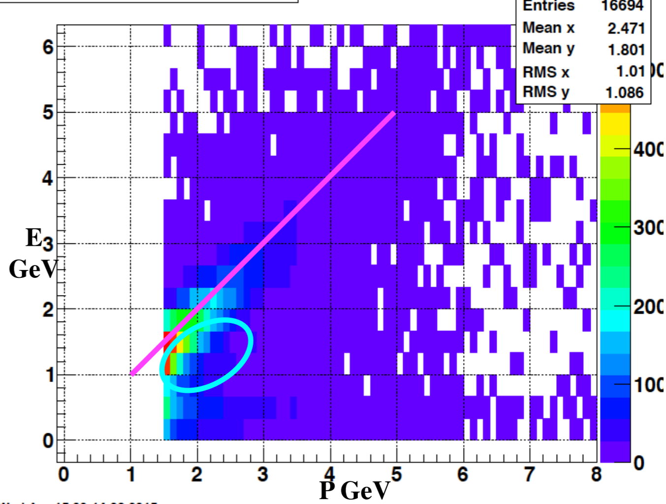
Evsp_Unbiased
