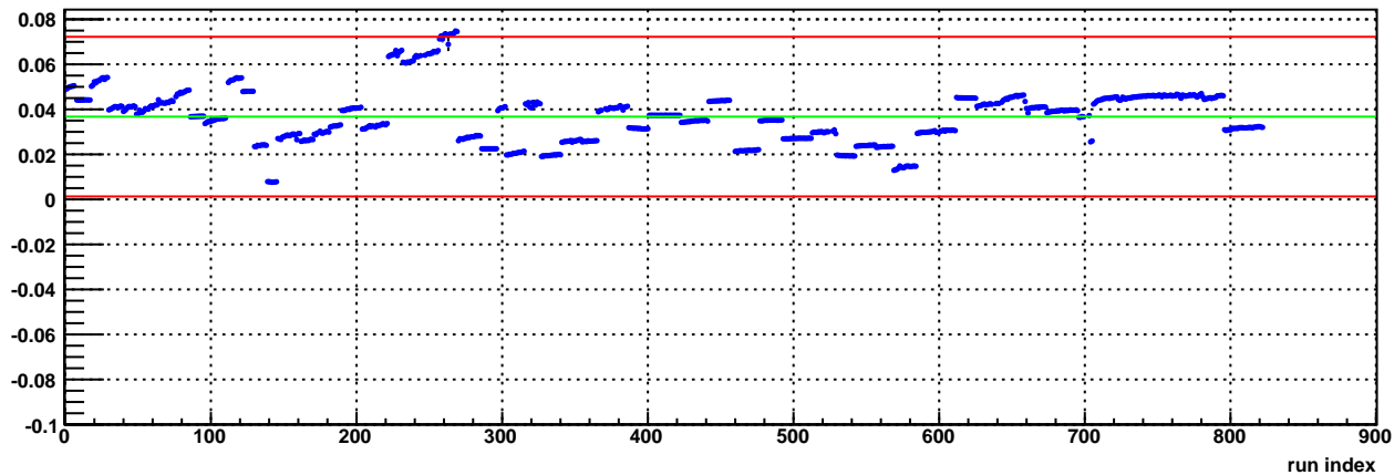
L2EW Vertex X (cm)
