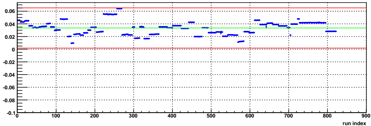
L2BW Vertex X (cm)
