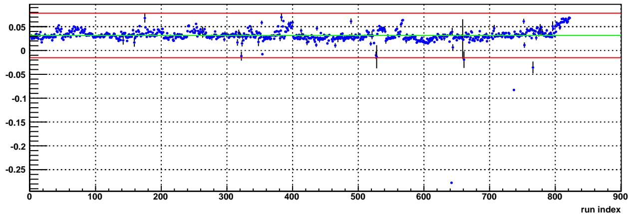
L2EW BARREL Tower \eta
