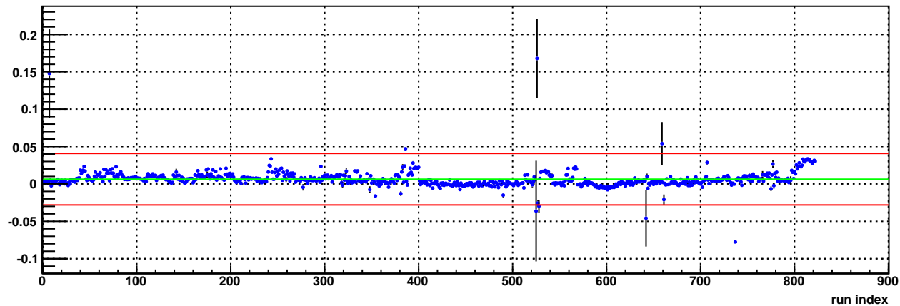
L2BW BARREL Tower \eta
