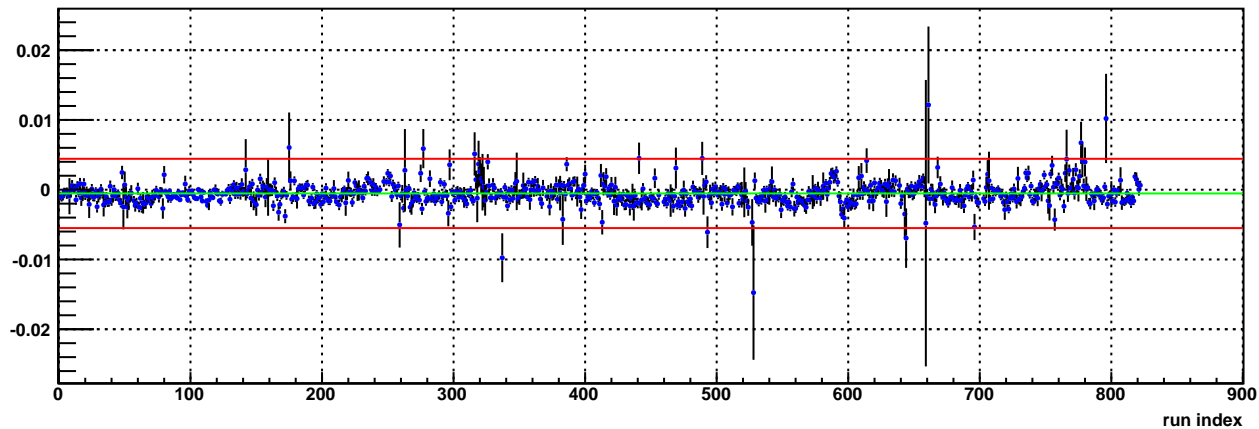
L2EW Track dcaZ (cm)
