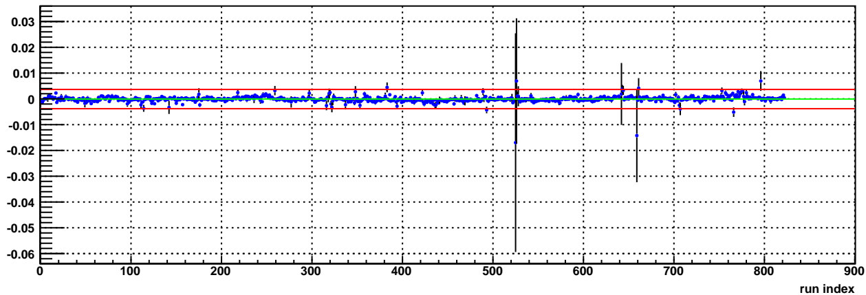
L2BW Track dcaZ (cm)
