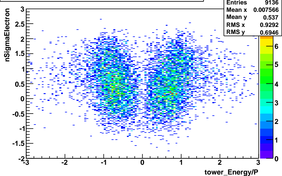
BHT1_nSigmaElectron_vs_EoverP-nSigmaPion_Cut-applied
