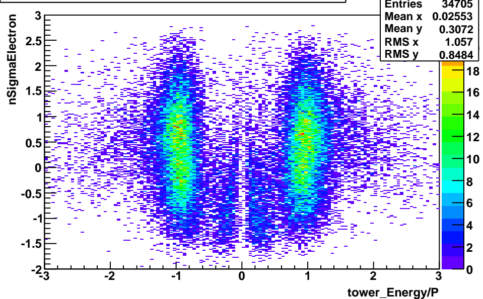
BHT1_nSigmaElectron_vs_EoverP-nSigmaPion_Cut-applied
