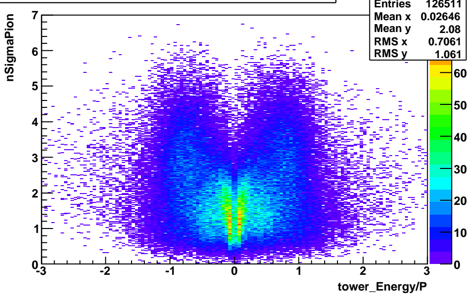
BHT3_nSigmaPion_vs_EoverP-nSigmaElectron_cut-applied
