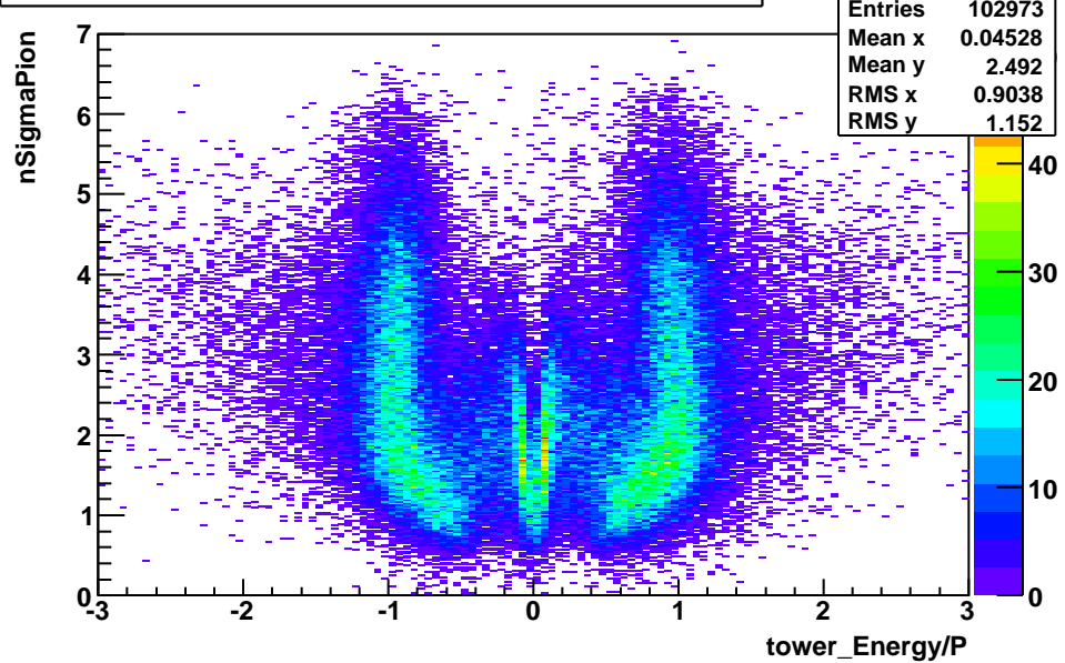
BHT1_nSigmaPion_vs_EoverP-nSigmaPion_Cut-applied
