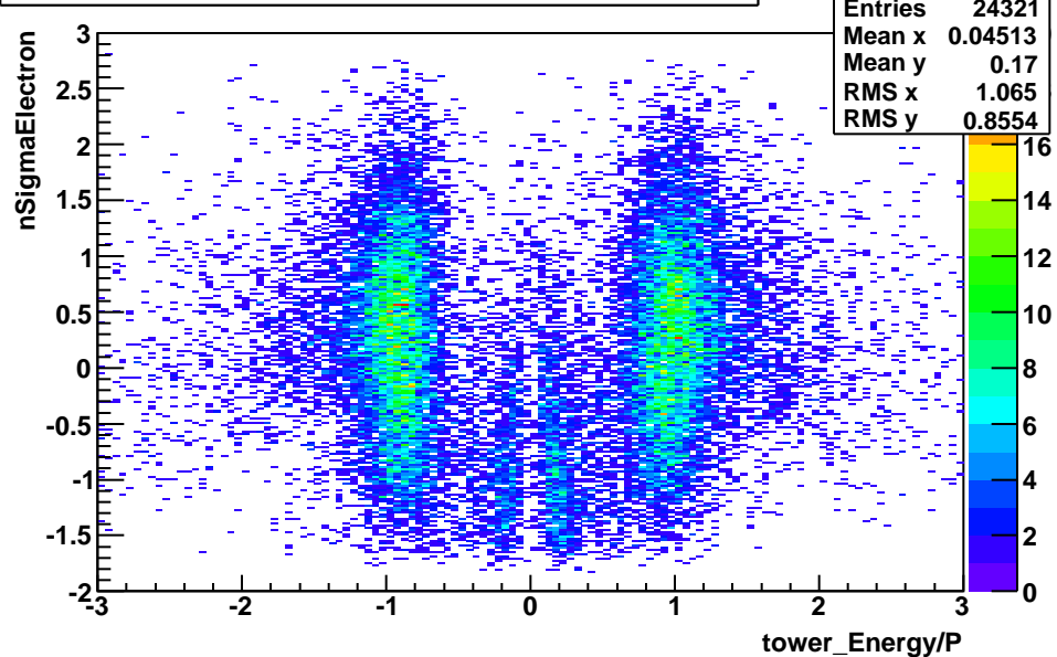
BHT1_nSigmaElectron_vs_EoverP-nSigmaPion_Cut-applied
