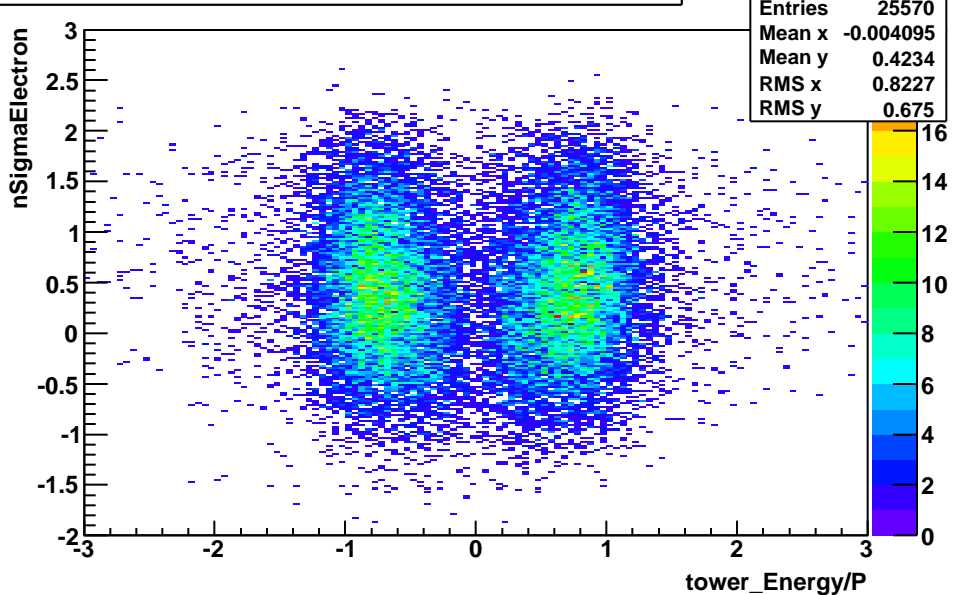
BHT3_nSigmaElectron_vs_EoverP-nSigmaPion_Cut-applied
