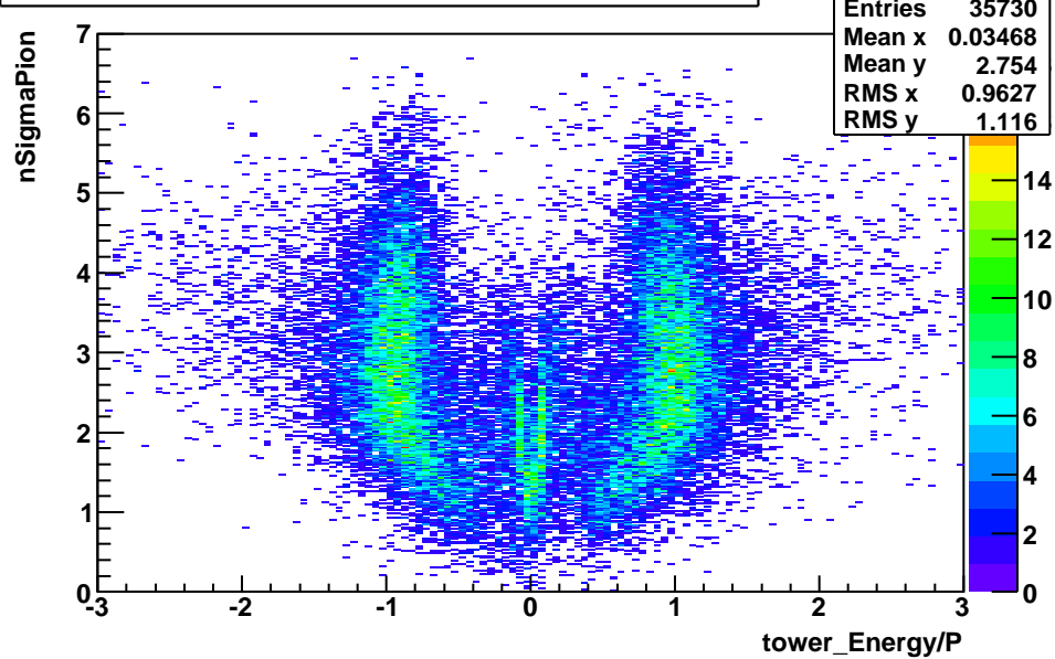
BHT1_nSigmaPion_vs_EoverP-nSigmaPion_Cut-applied
