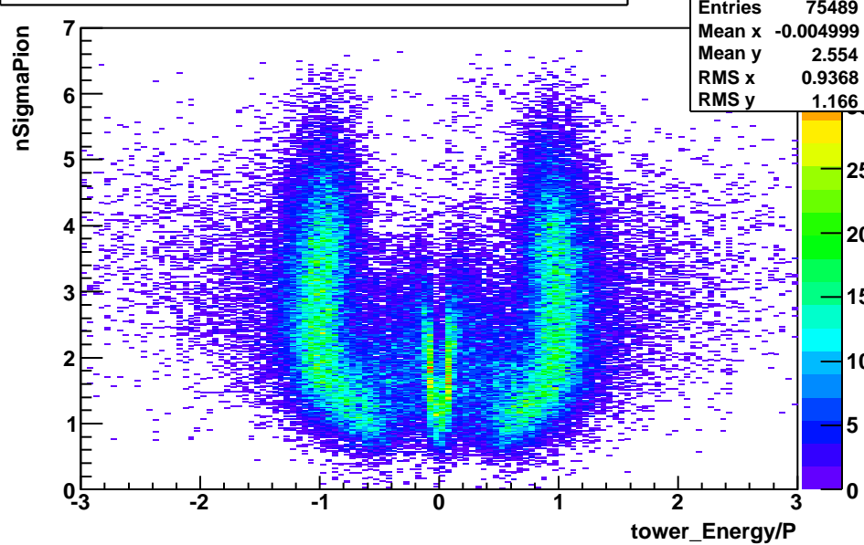
BHT1_nSigmaPion_vs_EoverP-nSigmaPion_Cut-applied
