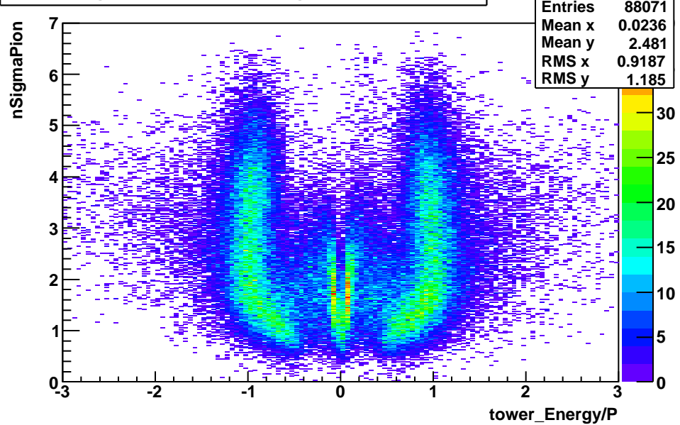
BHT1_nSigmaPion_vs_EoverP-nSigmaPion_Cut-applied
