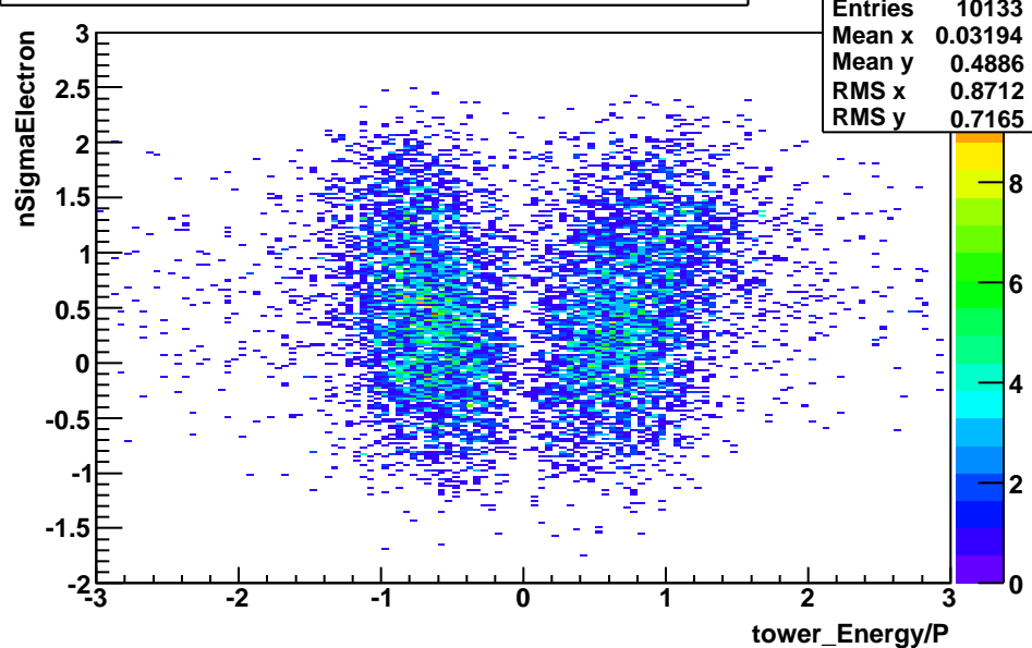
BHT1_nSigmaElectron_vs_EoverP-nSigmaPion_Cut-applied
