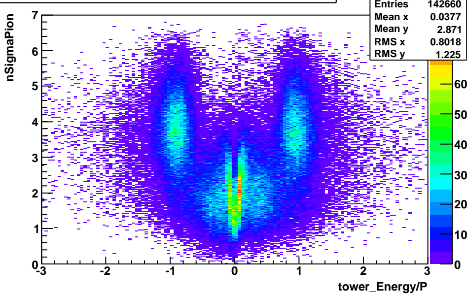
BHT3_nSigmaPion_vs_EoverP-nSigmaElectron_cut-applied
