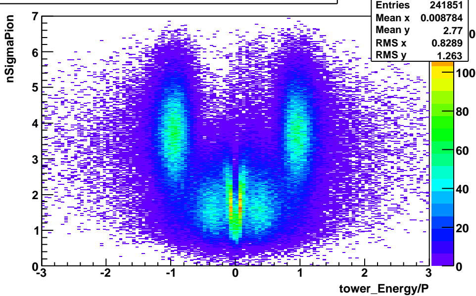
BHT3_nSigmaPion_vs_EoverP-nSigmaElectron_cut-applied
