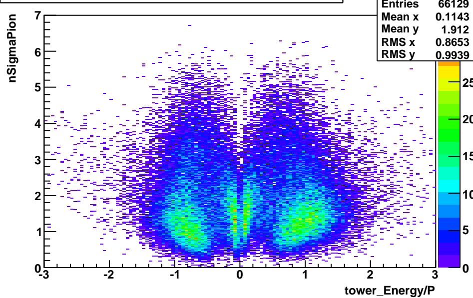
BHT1_nSigmaPion_vs_EoverP-nSigmaPion_Cut-applied
