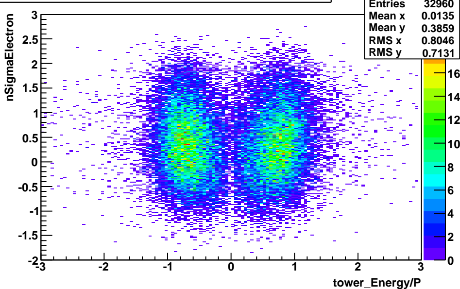
BHT3_nSigmaElectron_vs_EoverP-nSigmaPion_Cut-applied
