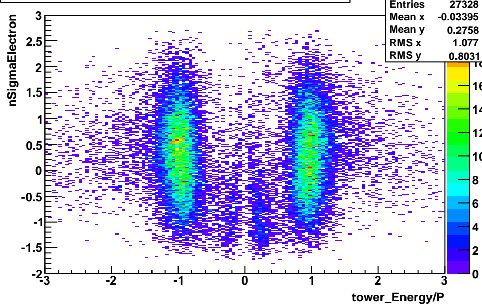
BHT1_nSigmaElectron_vs_EoverP-nSigmaPion_Cut-applied
