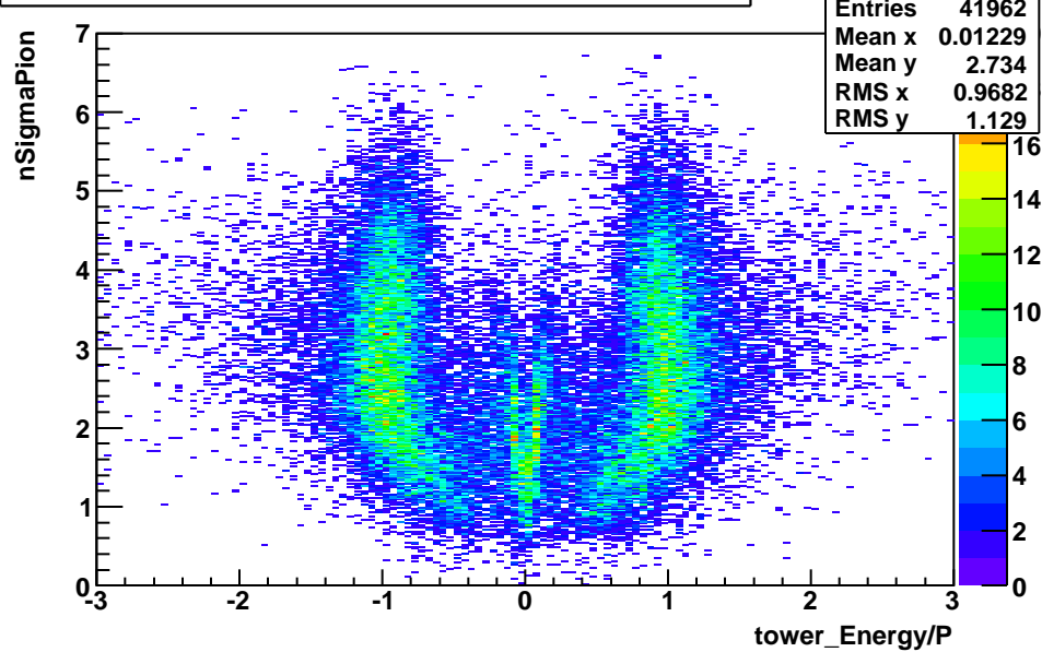
BHT1_nSigmaPion_vs_EoverP-nSigmaPion_Cut-applied
