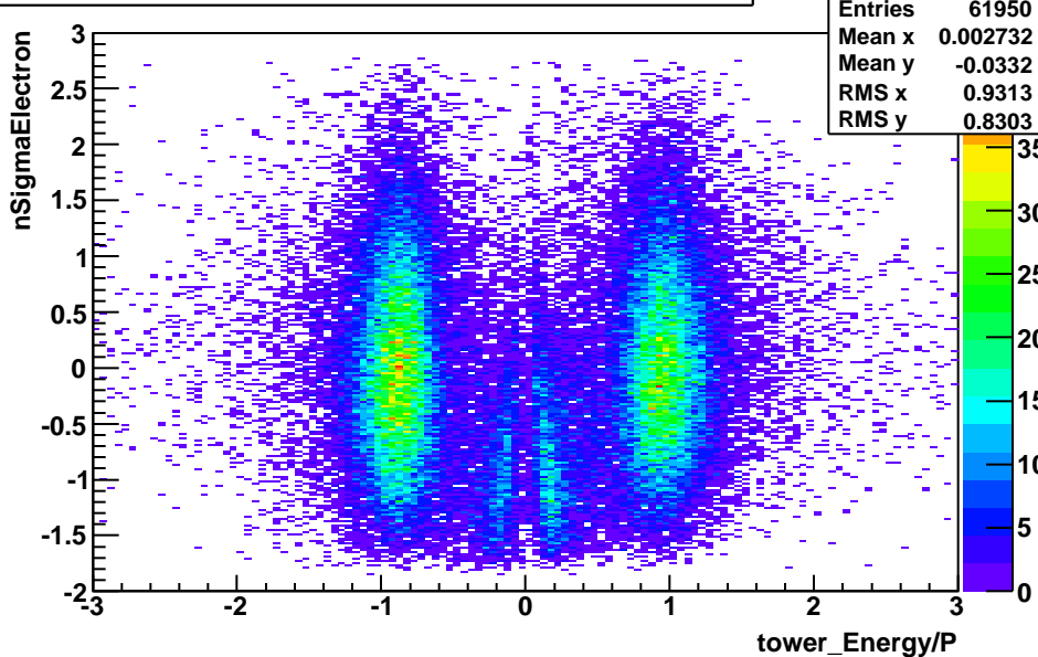
BHT3_nSigmaElectron_vs_EoverP-nSigmaPion_Cut-applied
