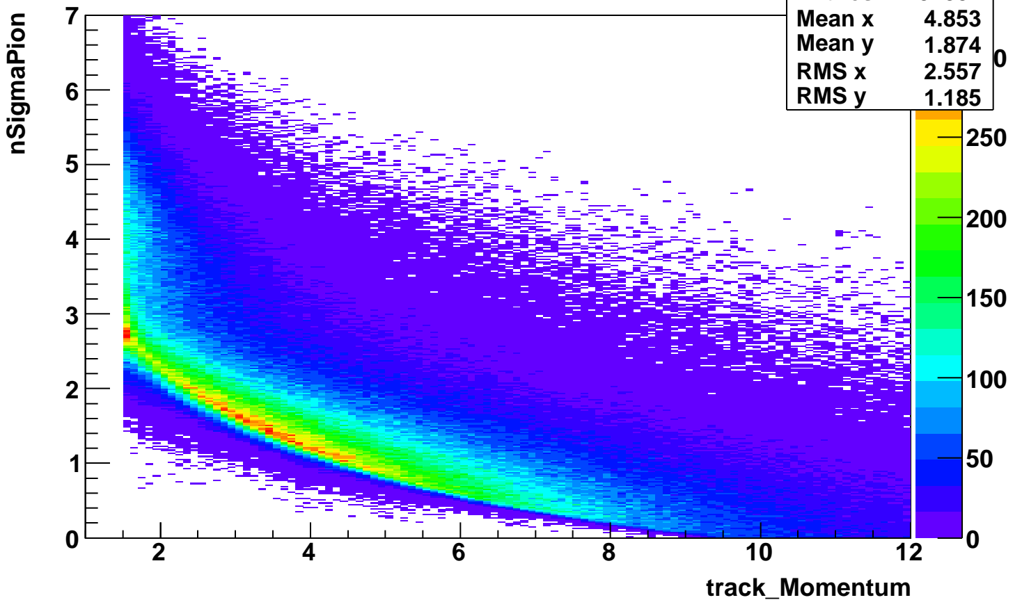
nSigmaPion_vs_momentum-NoElectronCut-applied
