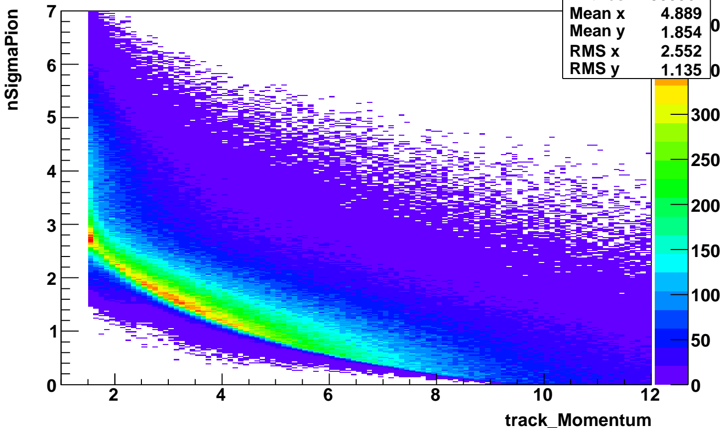
nSigmaPion_vs_momentum-NoElectronCut-applied
