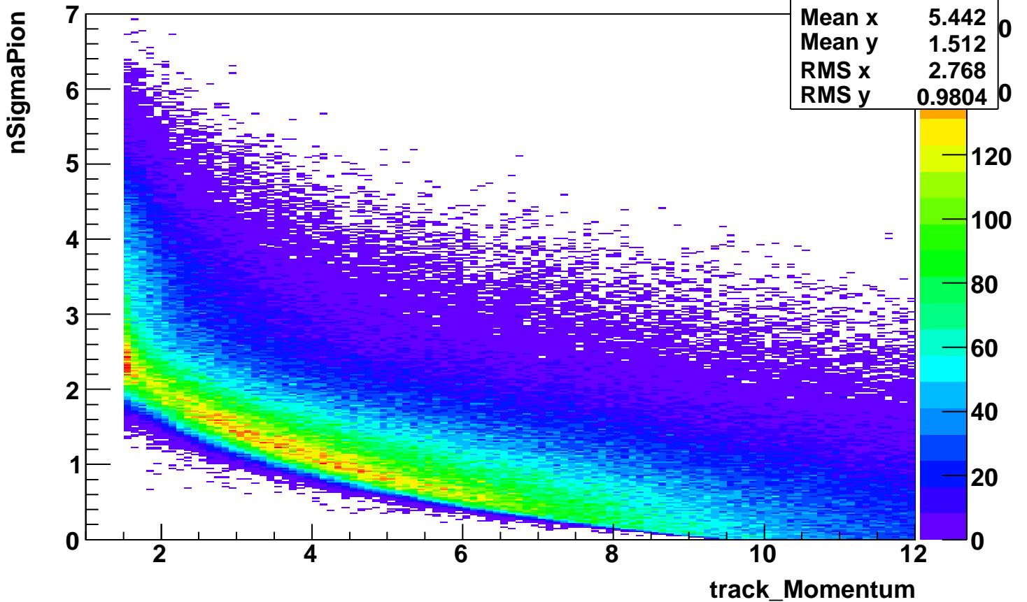
nSigmaPion_vs_momentum-NoElectronCut-applied
