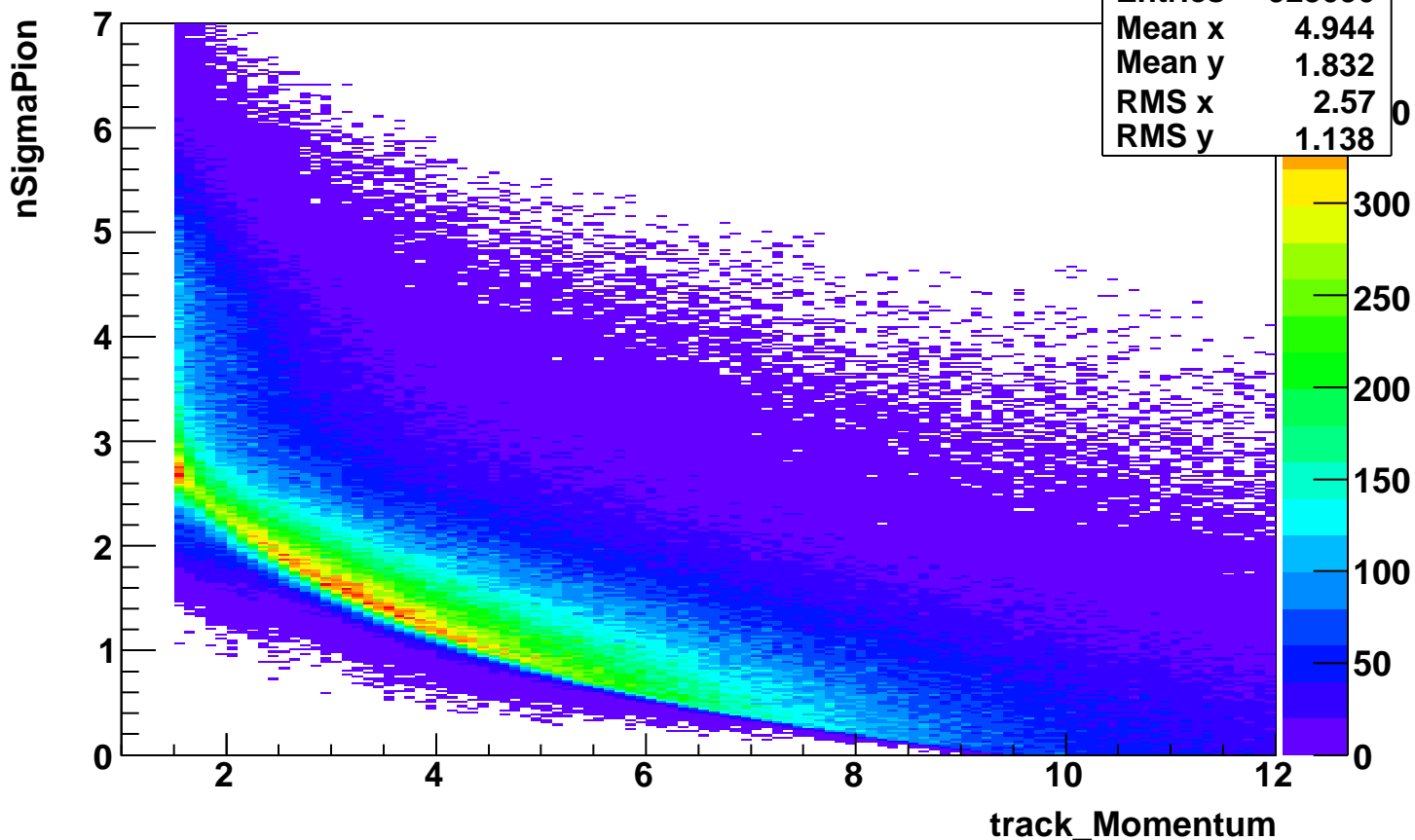
nSigmaPion_vs_momentum-NoElectronCut-applied
