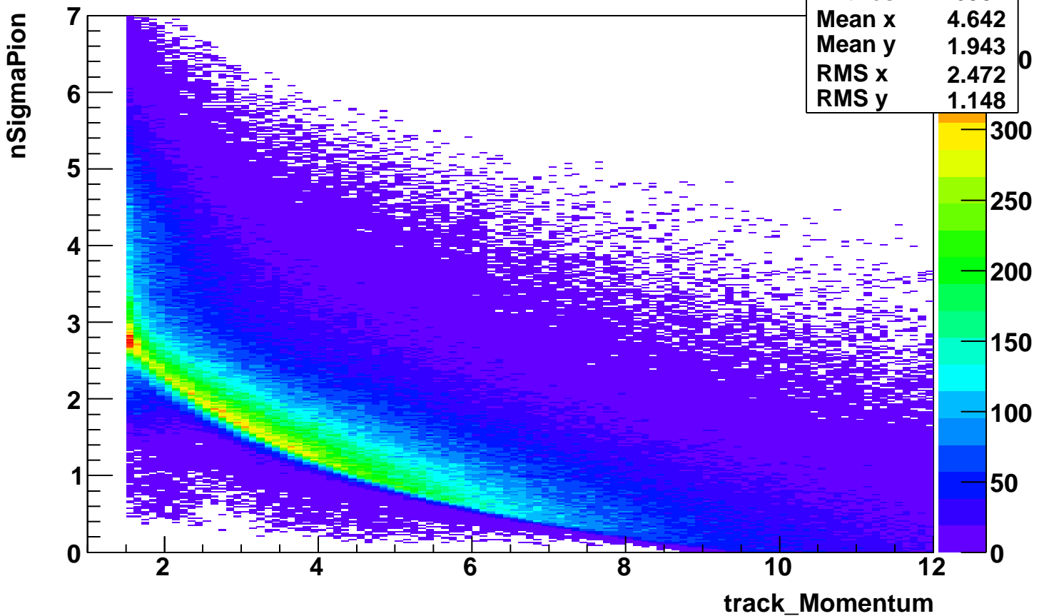
nSigmaPion_vs_momentum-NoElectronCut-applied
