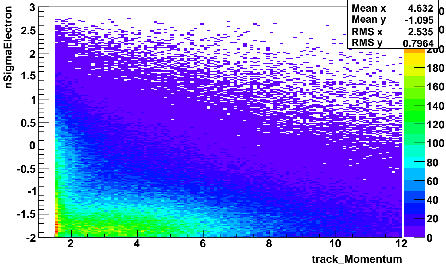
nSigmaElectron_vs_momentum-NOpionCut-applied
