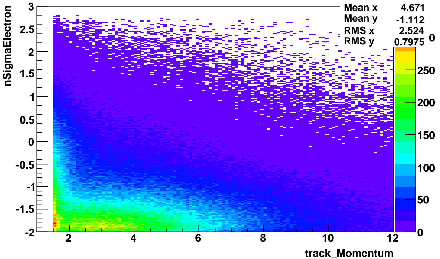
nSigmaElectron_vs_momentum-NOpionCut-applied
