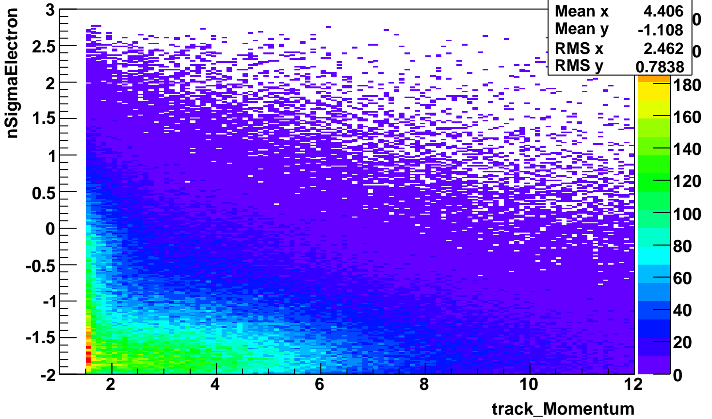
nSigmaElectron_vs_momentum-NOpionCut-applied
