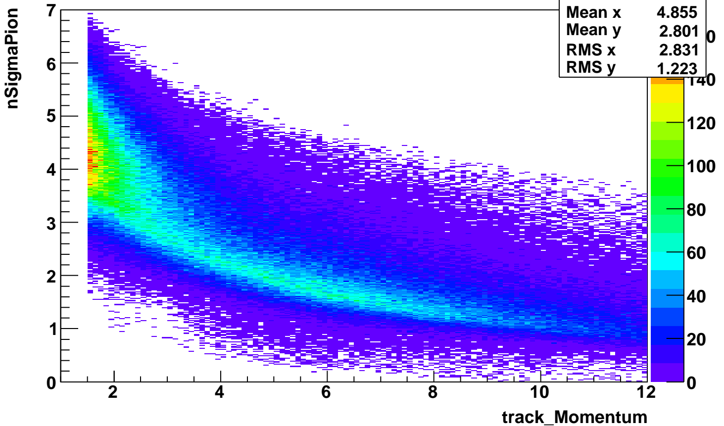
nSigmaPion_vs_momentum-ElectronCut-applied
