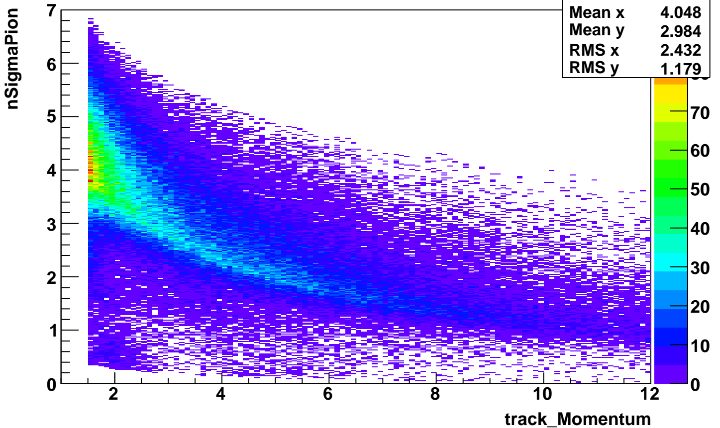
nSigmaPion_vs_momentum-ElectronCut-applied
