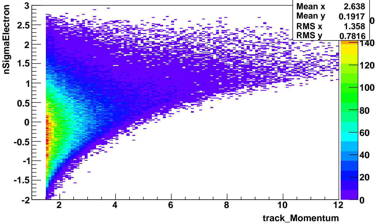
nSigmaElectron_vs_momentum-pionCut-applied
