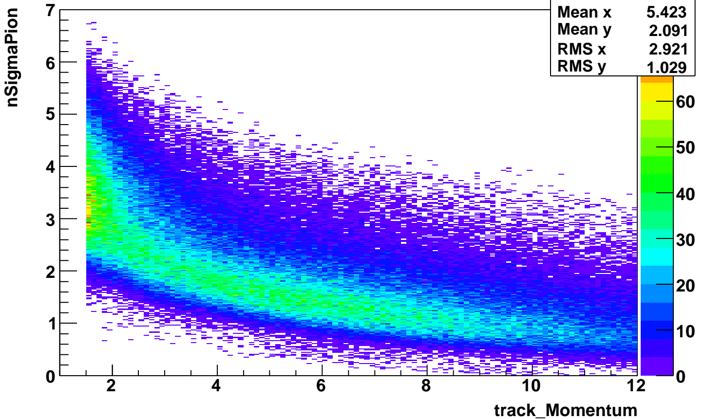
nSigmaPion_vs_momentum-ElectronCut-applied
