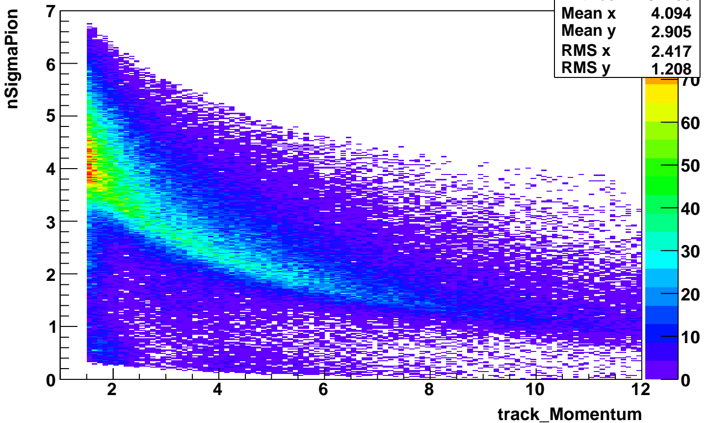
nSigmaPion_vs_momentum-ElectronCut-applied
