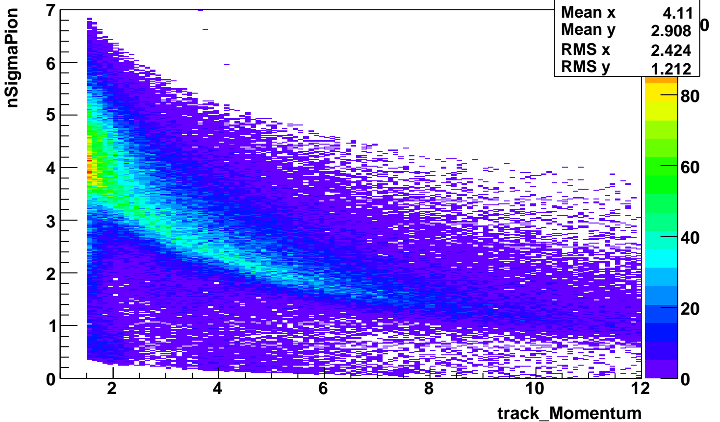
nSigmaPion_vs_momentum-ElectronCut-applied
