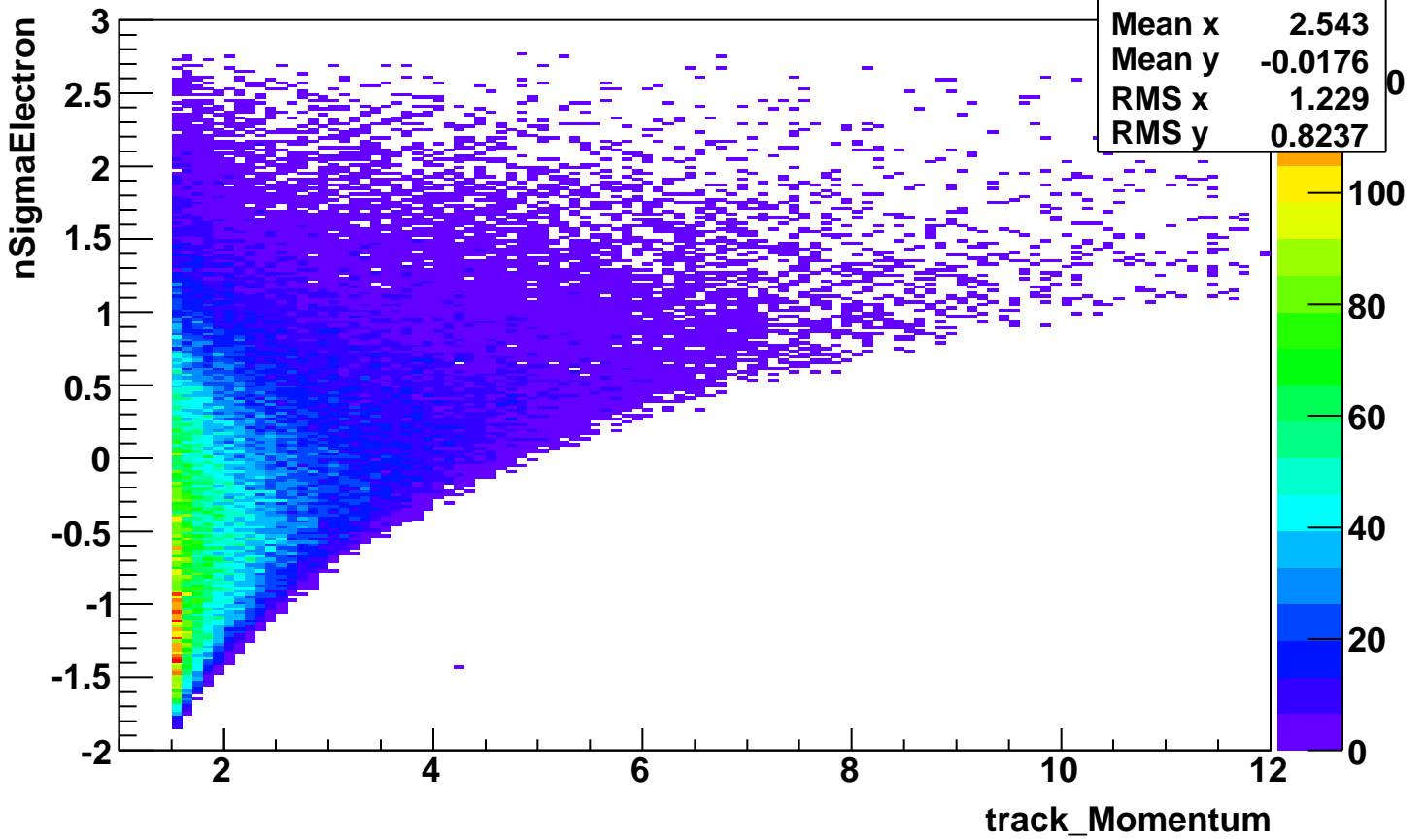
nSigmaElectron_vs_momentum-pionCut-applied
