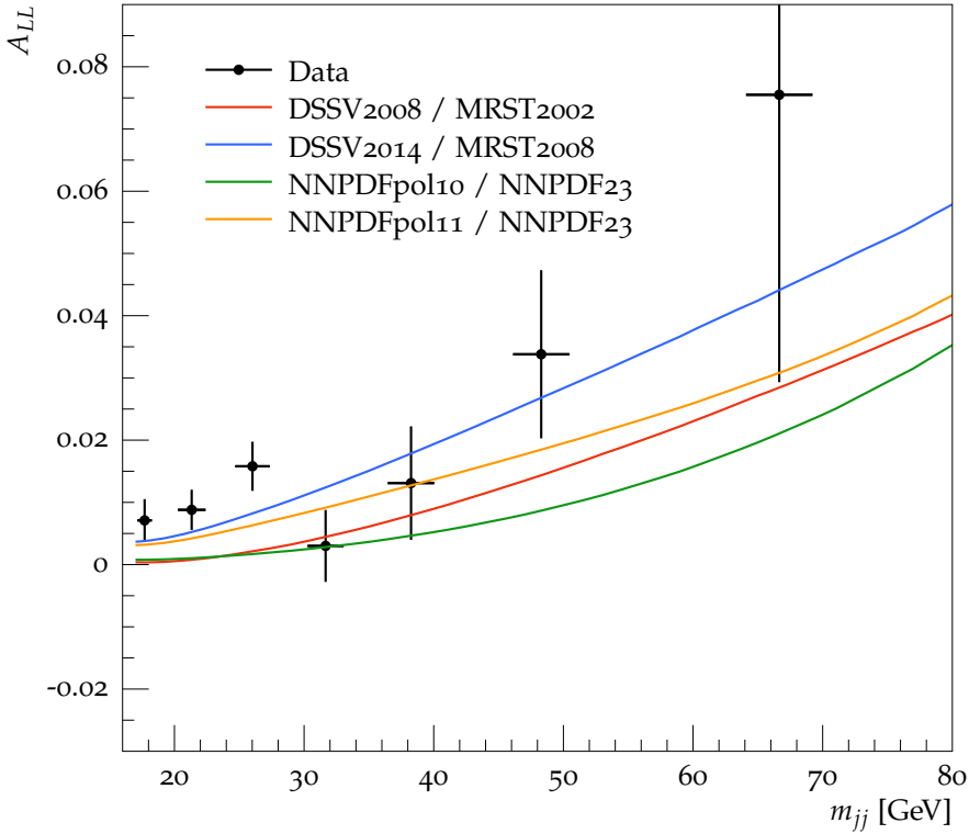
Dijet A_{LL} for |y| < 0.8 , EE+WW, anti- k_T , R = 0.6
