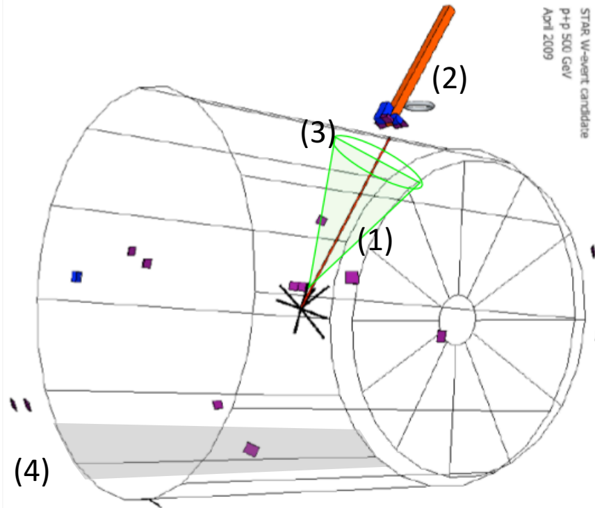
Event Display of typical W event
