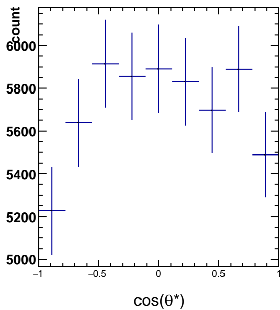
RawYields 1.8 < p_T < 2.4 , 10\pi/6 < \phi' < 11\pi/6
