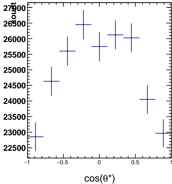
RawYields 1.2 < p_T < 1.8 , 8\pi/6 < \phi^* < 9\pi/6
