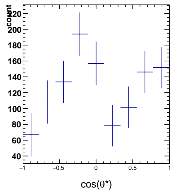
RawYields 3.0 < p_T < 4.2 , 11\pi/6 < \phi' < 12\pi/6
