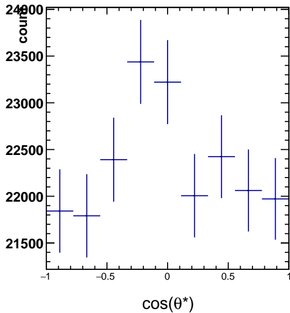
RawYields 1.2 < p_T < 1.8 , 10\pi/6 < \phi' < 11\pi/6
