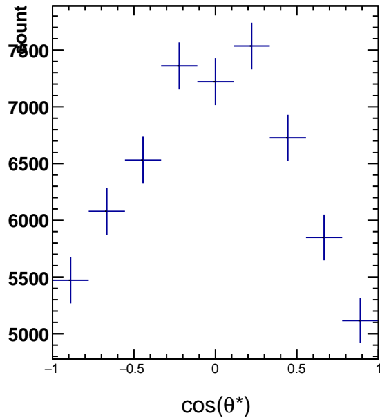
RawYields 1.8 < p_T < 2.4 , 2\pi/6 < \phi^* < 3\pi/6
