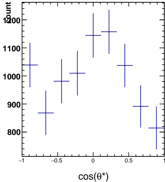
RawYields 2.4 < p_T < 3.0 , 4\pi/6 < \phi^* < 5\pi/6
