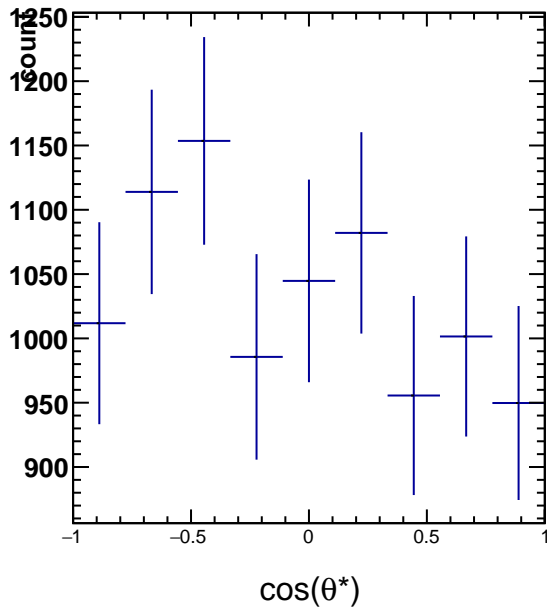
RawYields 2.4 < p_T < 3.0, 9\pi/6 < \phi' < 10\pi/6
