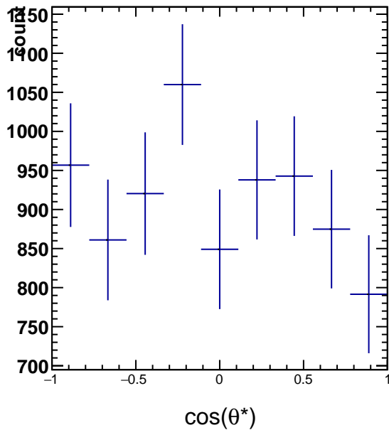
RawYields 2.4 < p_T < 3.0 , 6\pi/6 < \phi^* < 7\pi/6
