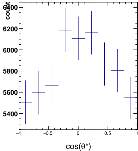
RawYields 1.8 < p_T < 2.4 , 4\pi/6 < \phi^* < 5\pi/6
