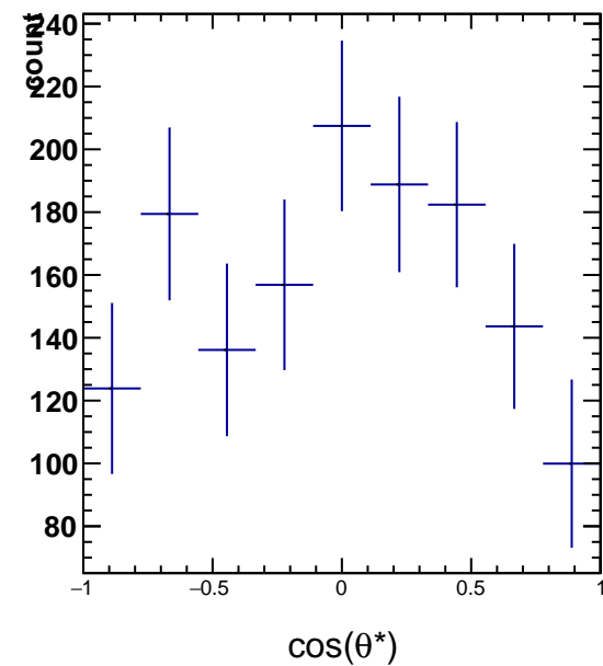
RawYields 3.0 < p_T < 4.2, 9\pi/6 < \phi' < 10\pi/6
