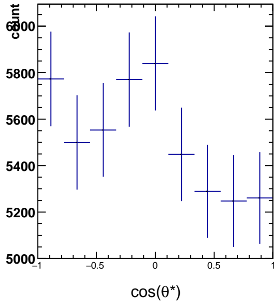
RawYields 1.8 < p_T < 2.4 , 0\pi/6 < \phi' < 1\pi/6
