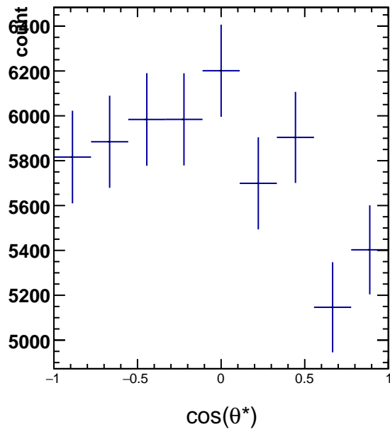
RawYields 1.8 < p_T < 2.4 , 1\pi/6 < \phi' < 2\pi/6
