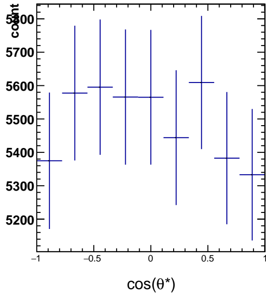
RawYields 1.8 < p_T < 2.4 , 5\pi/6 < \phi^* < 6\pi/6
