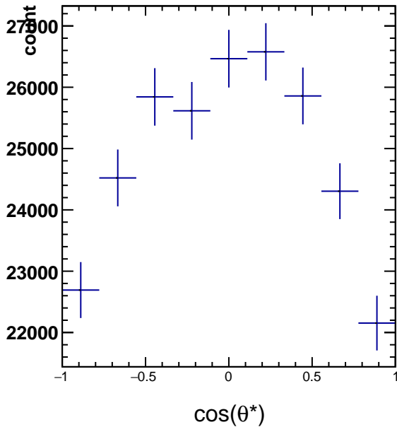
RawYields 1.2 < p_T < 1.8, 9\pi/6 < \phi' < 10\pi/6
