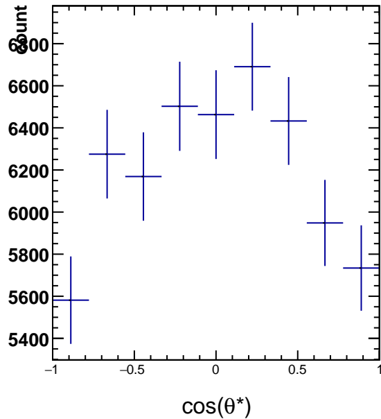
RawYields 1.8 < p_T < 2.4 , 8\pi/6 < \phi^* < 9\pi/6
