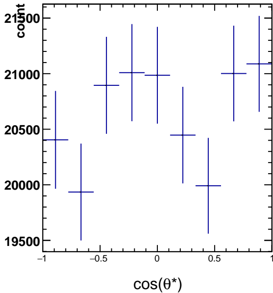
RawYields 1.2 < p_T < 1.8 , 0\pi/6 < \phi' < 1\pi/6
