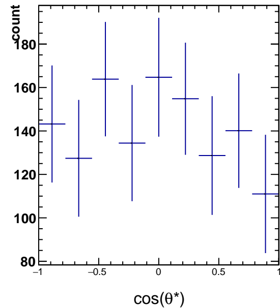
RawYields 3.0 < p_T < 4.2 , 10\pi/6 < \phi' < 11\pi/6
