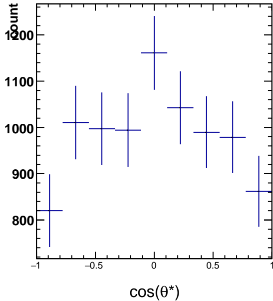
RawYields 2.4 < p_T < 3.0 , 8\pi/6 < \phi^* < 9\pi/6
