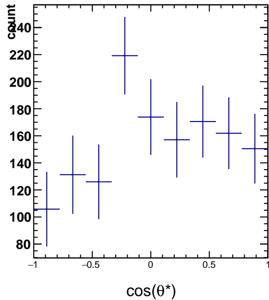
RawYields 3.0 < p_T < 4.2 , 1\pi/6 < \phi' < 2\pi/6
