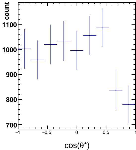
RawYields 2.4 < p_T < 3.0 , 1\pi/6 < \phi' < 2\pi/6
