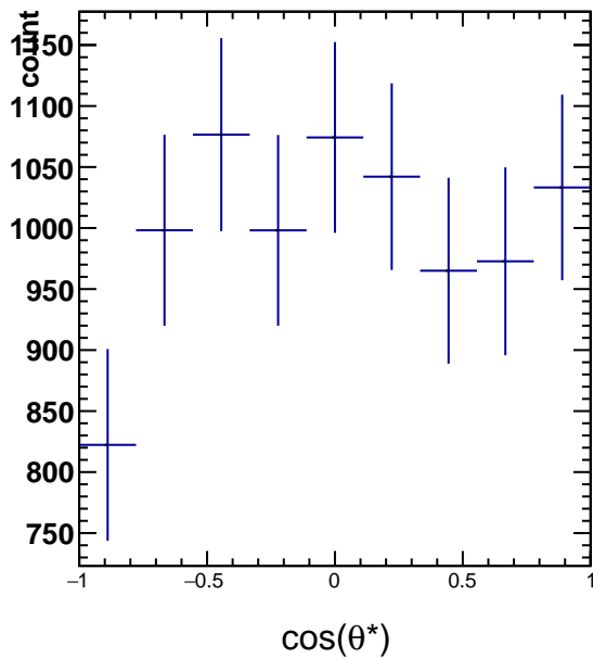
RawYields 2.4 < p_T < 3.0 , 10\pi/6 < \phi' < 11\pi/6
