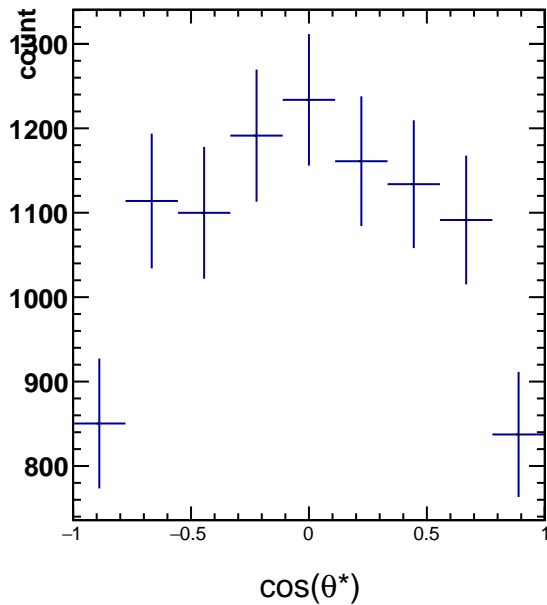
RawYields 2.4 < p_T < 3.0 , 2\pi/6 < \phi^* < 3\pi/6
