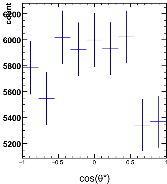
RawYields 1.8 < p_T < 2.4, 7\pi/6 < \phi^1 < 8\pi/6
