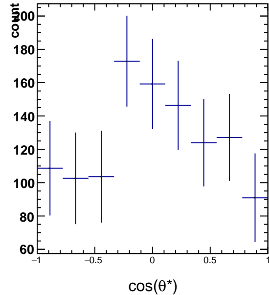
RawYields 3.0 < p_T < 4.2 , 8\pi/6 < \phi^* < 9\pi/6
