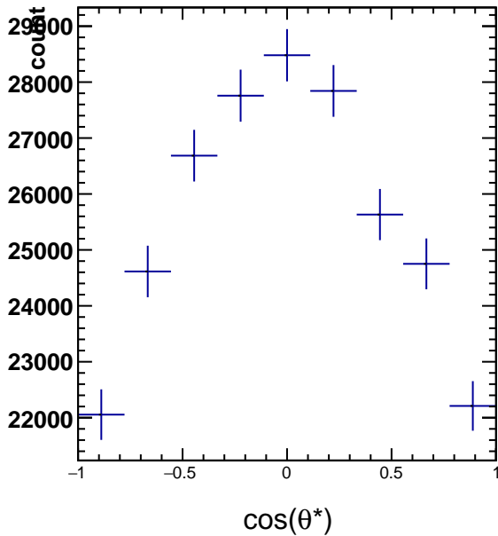
RawYields 1.2 < p_T < 1.8 , 3\pi/6 < \phi^* < 4\pi/6
