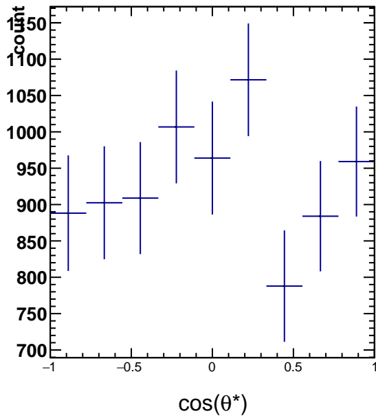
RawYields 2.4 < p_T < 3.0, 7\pi/6 < \phi^1 < 8\pi/6
