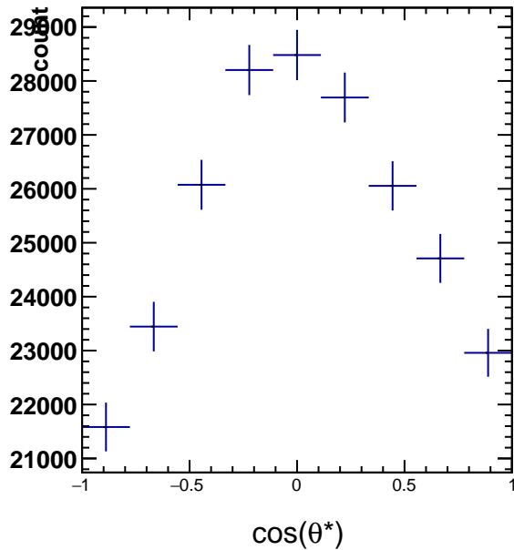
RawYields 1.2 < p_T < 1.8 , 2\pi/6 < \phi^* < 3\pi/6
