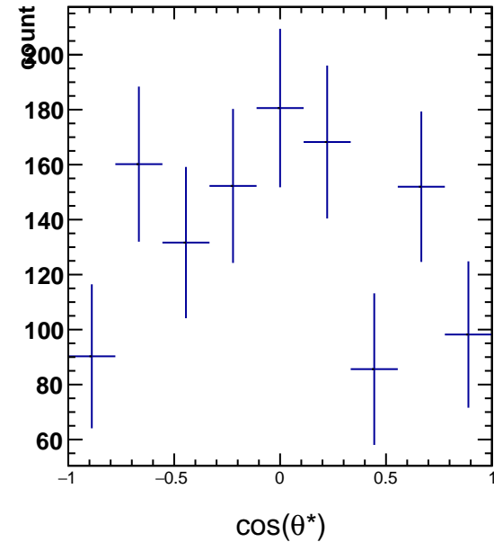
RawYields 3.0 < p_T < 4.2 , 4\pi/6 < \phi^* < 5\pi/6
