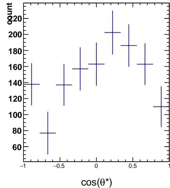
RawYields 3.0 < p_T < 4.2 , 2\pi/6 < \phi^* < 3\pi/6
