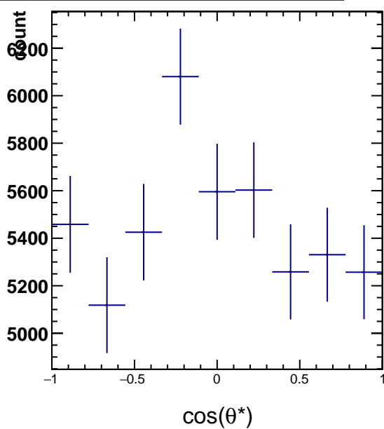
RawYields 1.8 < p_T < 2.4 , 11\pi/6 < \phi' < 12\pi/6
