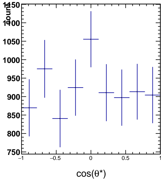
RawYields 2.4 < p_T < 3.0 , 5\pi/6 < \phi^* < 6\pi/6
