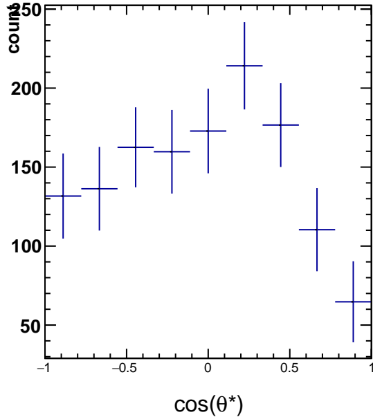
RawYields 3.0 < p_T < 4.2 , 3\pi/6 < \phi^* < 4\pi/6
