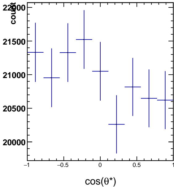
RawYields 1.2 < p_T < 1.8 , 5\pi/6 < \phi^* < 6\pi/6
