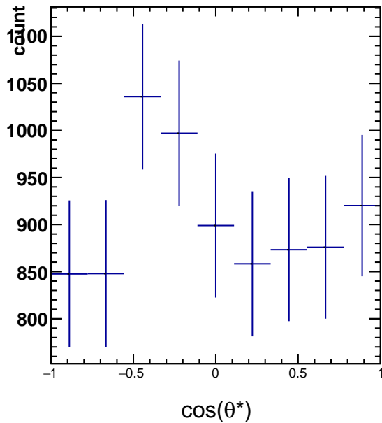
RawYields 2.4 < p_T < 3.0 , 0\pi/6 < \phi' < 1\pi/6
