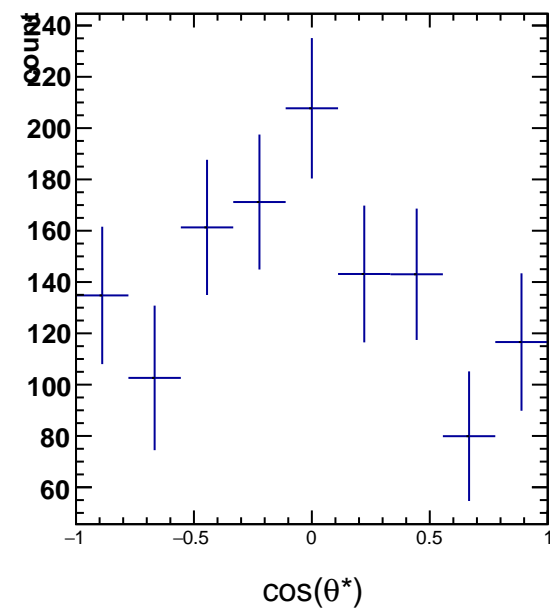
RawYields 3.0 < p_T < 4.2 , 5\pi/6 < \phi^* < 6\pi/6
