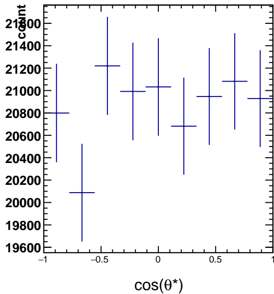
RawYields 1.2 < p_T < 1.8 , 6\pi/6 < \phi^* < 7\pi/6
