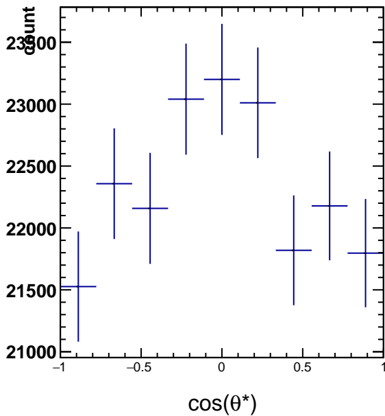
RawYields 1.2 < p_T < 1.8, 7\pi/6 < \phi^1 < 8\pi/6
