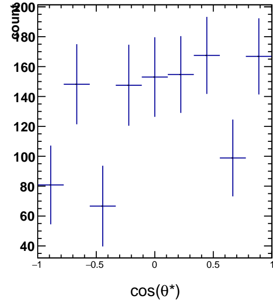
RawYields 3.0 < p_T < 4.2 , 0\pi/6 < \phi' < 1\pi/6
