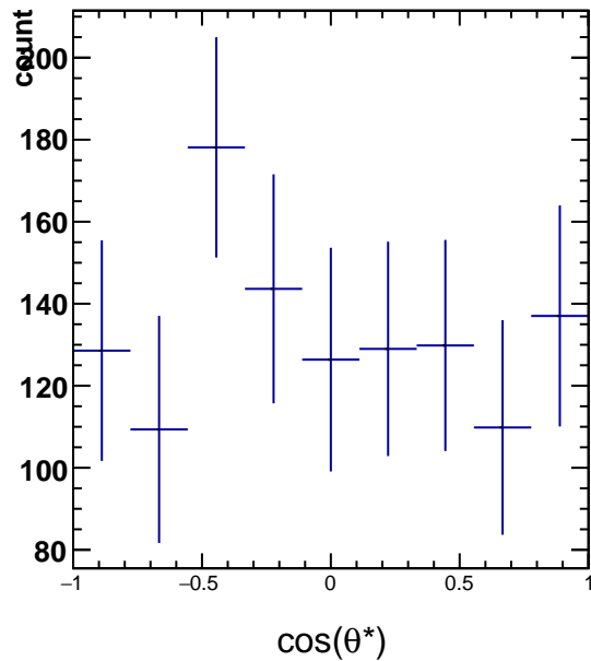
RawYields 3.0 < p_T < 4.2 , 6\pi/6 < \phi^* < 7\pi/6
