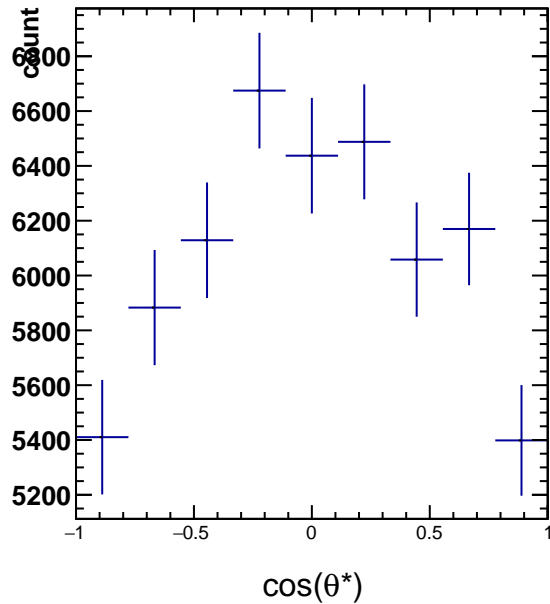
RawYields 1.8 < p_T < 2.4, 9\pi/6 < \phi' < 10\pi/6
