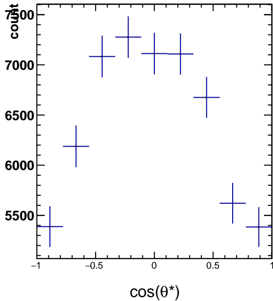
RawYields 1.8 < p_T < 2.4 , 3\pi/6 < \phi^* < 4\pi/6
