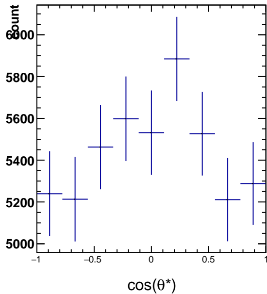
RawYields 1.8 < p_T < 2.4 , 6\pi/6 < \phi^* < 7\pi/6
