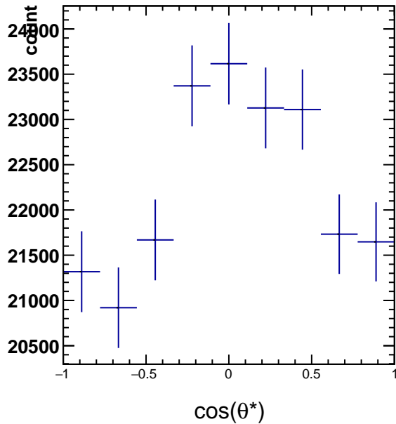
RawYields 1.2 < p_T < 1.8 , 4\pi/6 < \phi^* < 5\pi/6
