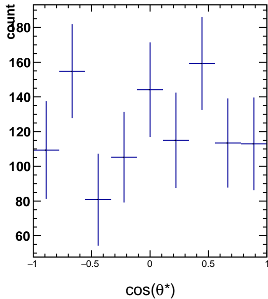
RawYields 3.0 < p_T < 4.2, 7\pi/6 < \phi^1 < 8\pi/6
