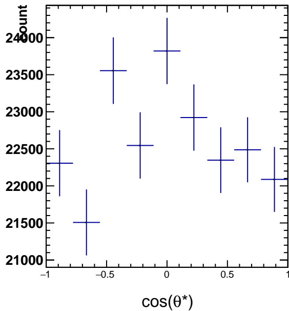
RawYields 1.2 < p_T < 1.8 , 1\pi/6 < \phi' < 2\pi/6
