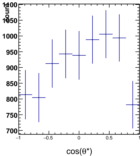
RawYields 2.4 < p_T < 3.0 , 11\pi/6 < \phi' < 12\pi/6
