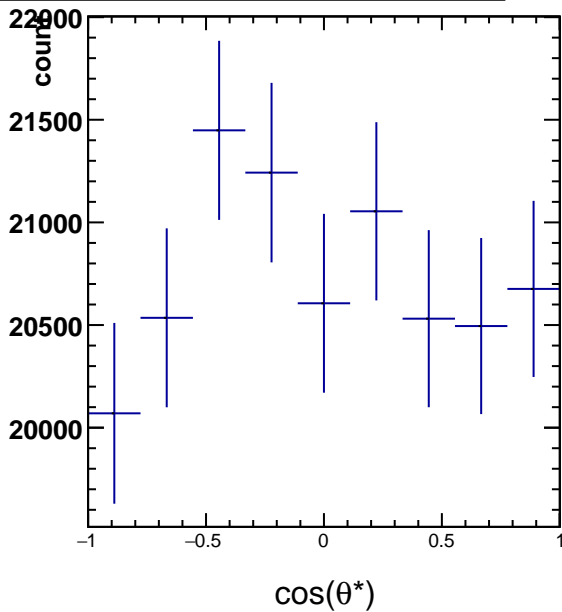
RawYields 1.2 < p_T < 1.8 , 11\pi/6 < \phi' < 12\pi/6
