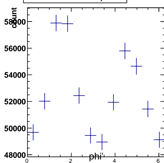
Raw Yields 1.8 < p_T < 2.4
