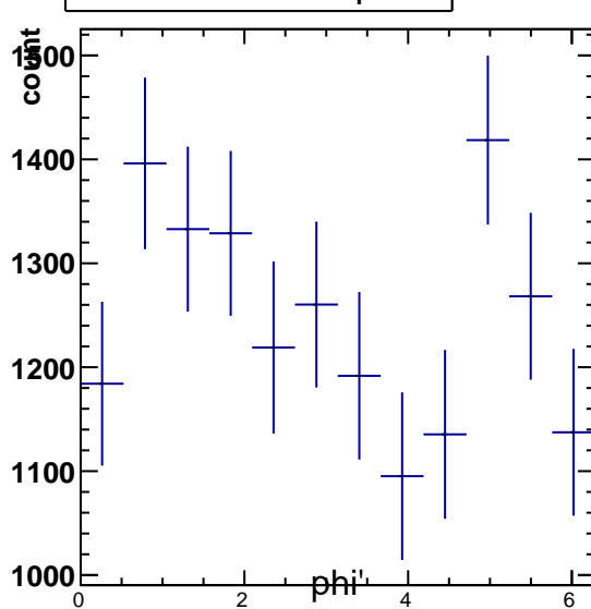
Raw Yields 3.0 < p_T < 4.2
