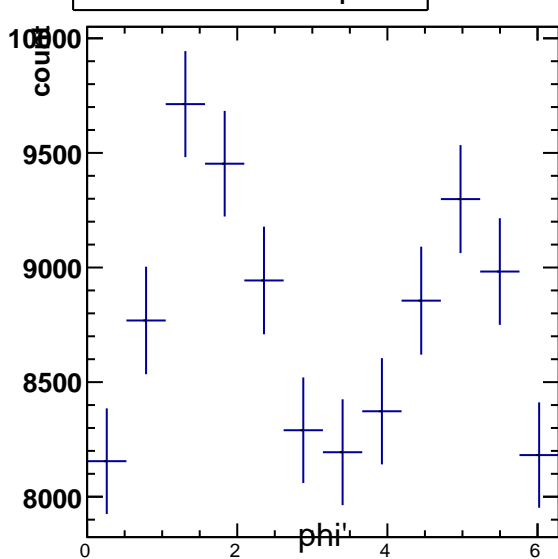
Raw Yields 2.4 < p_T < 3.0
