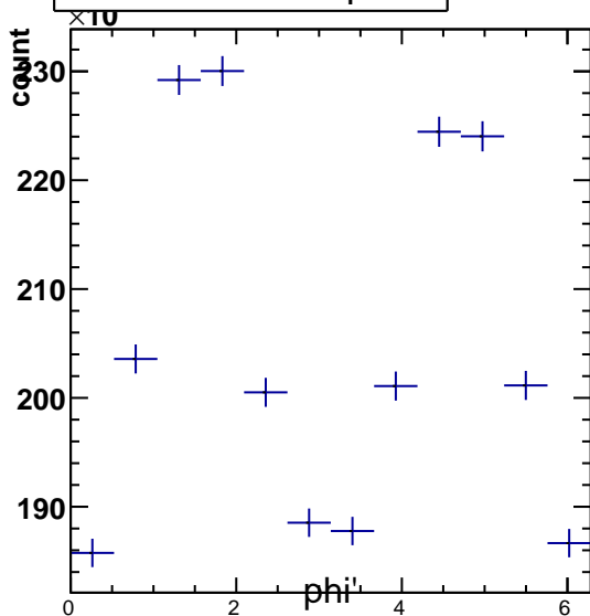
Raw Yields 1.2 < p_T < 1.8
