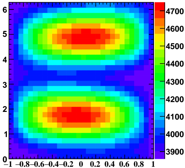
SpinDensity2Dcos
