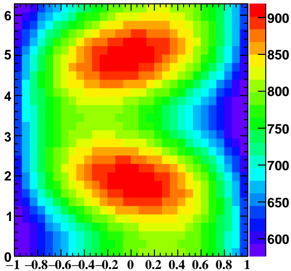
SpinDensity2Dcos
