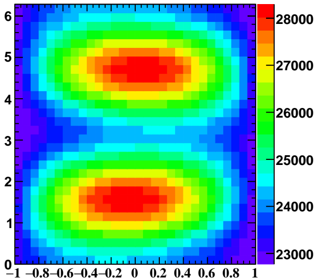
SpinDensity2Dcos
