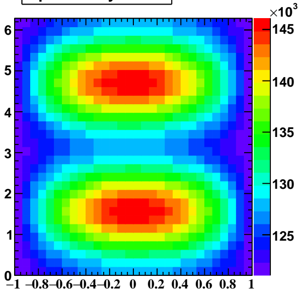
SpinDensity2Dcos
