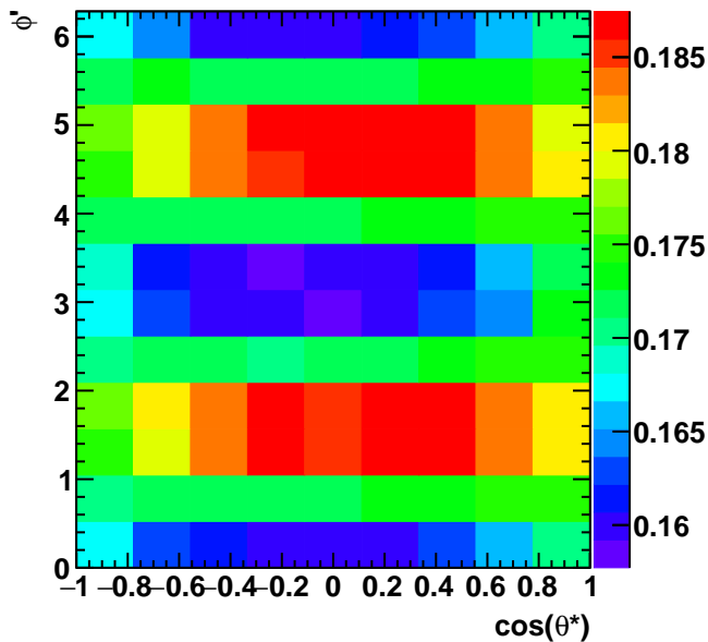
Efficiency 1.2 < p_{\top} < 1.8
