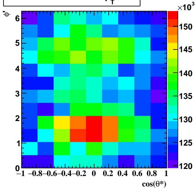
Corrected Yields 1.2 < p_T < 1.8
