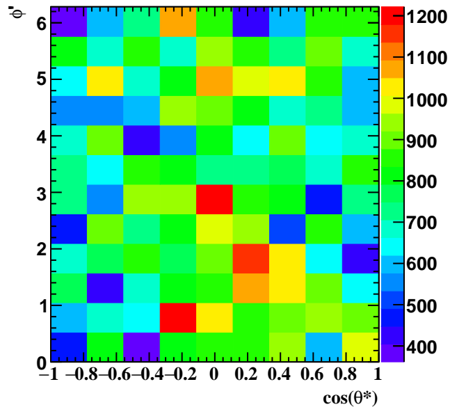
Corrected Yields 3.0 < p_T < 4.2
