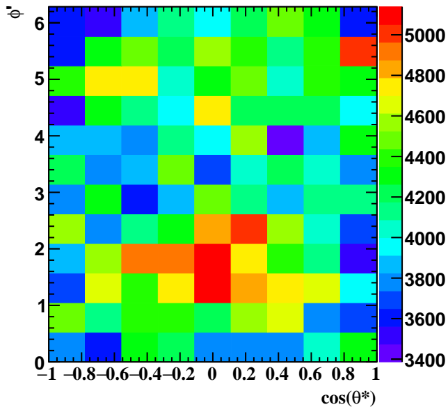
Corrected Yields 2.4 < p_T < 3.0
