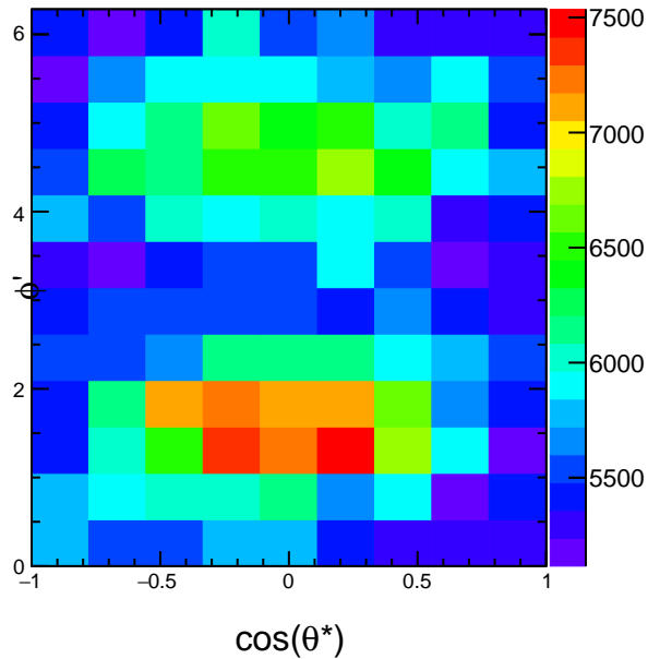
Raw Yields 1.8 < p_T < 2.4
