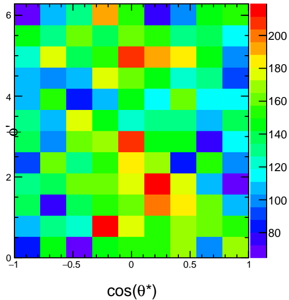
Raw Yields 3.0 < p_T < 4.2
