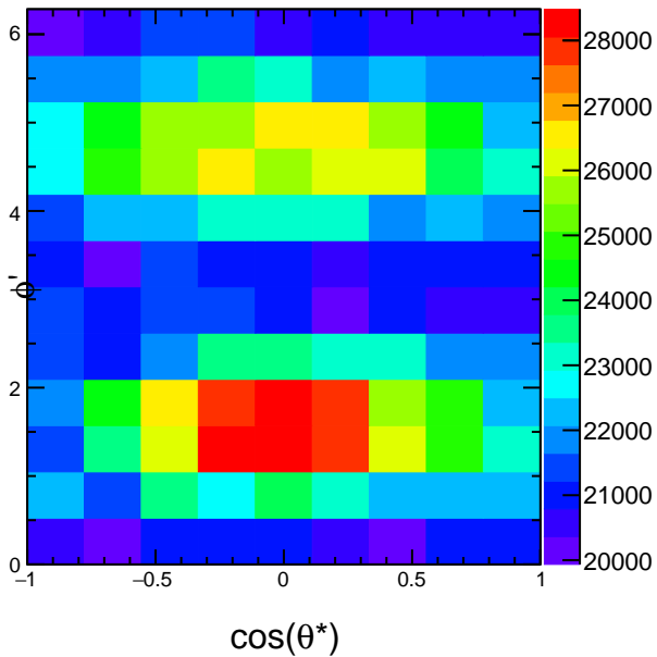
Raw Yields 1.2 < p_T < 1.8
