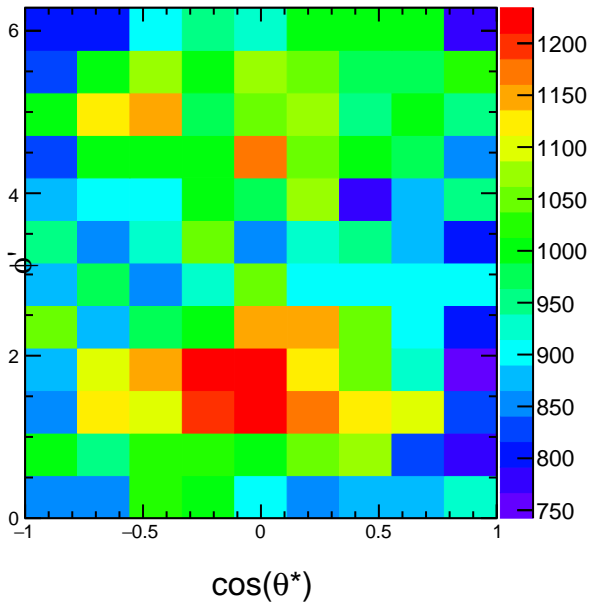
Raw Yields 2.4 < p_T < 3.0
