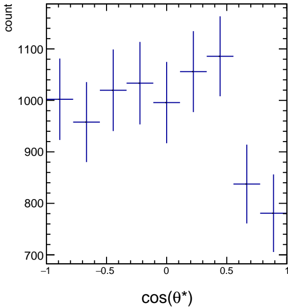
RawYields 2.4 < p_T < 3.0 , 1\pi/6 < \phi' < 2\pi/6
