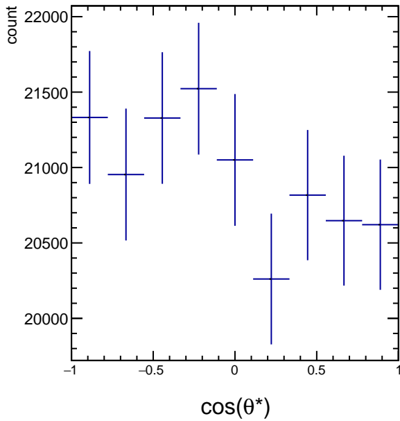
RawYields 1.2 < p_T < 1.8 , 5\pi/6 < \phi' < 6\pi/6
