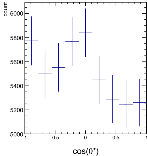
RawYields 1.8 < p_T < 2.4 , 0\pi/6 < \phi' < 1\pi/6
