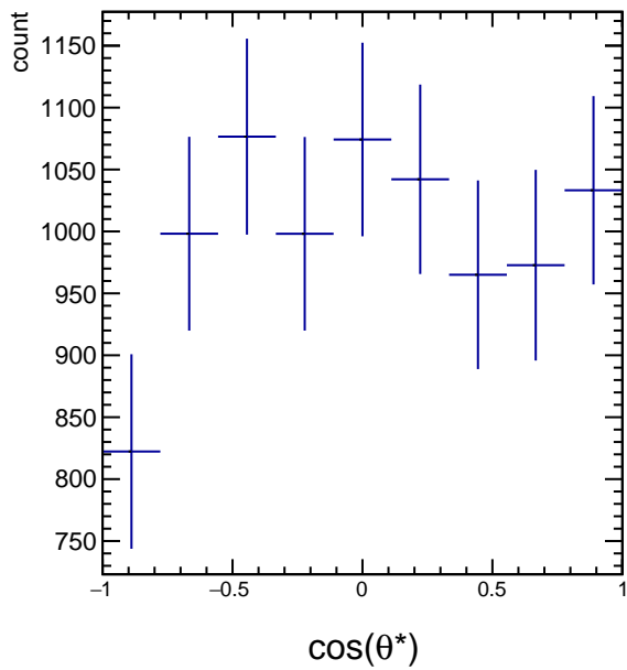
RawYields 2.4 < p_T < 3.0 , 10\pi/6 < \phi' < 11\pi/6
