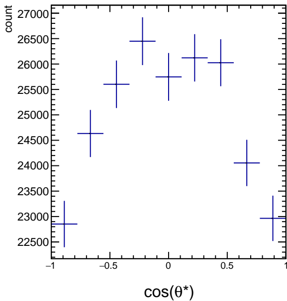
RawYields 1.2 < p_T < 1.8 , 8\pi/6 < \phi' < 9\pi/6
