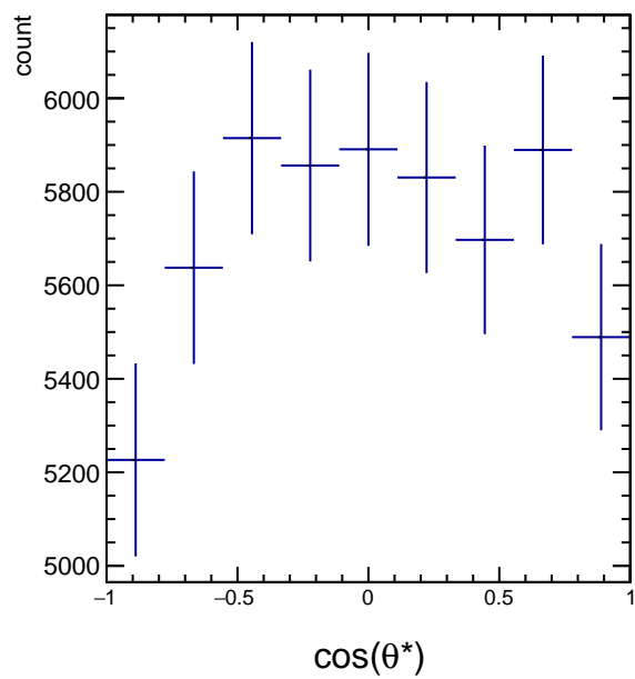
RawYields 1.8 < p_T < 2.4 , 10\pi/6 < \phi' < 11\pi/6
