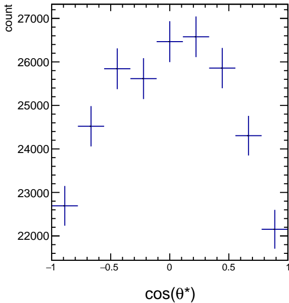
RawYields 1.2 < p_T < 1.8 , 9\pi/6 < \phi' < 10\pi/6
