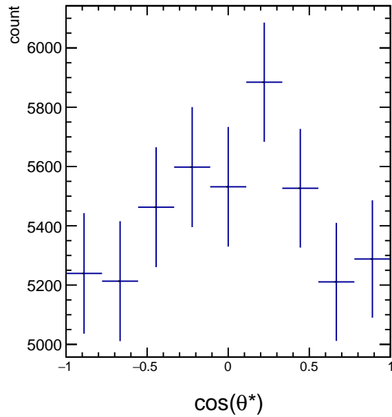
RawYields 1.8 < p_{\text{T}} < 2.4 , 6\pi/6 < \phi' < 7\pi/6
