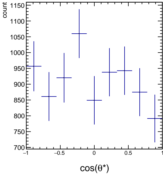
RawYields 2.4 < p_{\text{T}} < 3.0 , 6\pi/6 < \phi' < 7\pi/6
