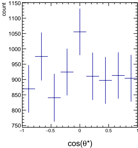
RawYields 2.4 < p_T < 3.0 , 5\pi/6 < \phi' < 6\pi/6
