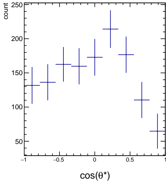
RawYields 3.0 < p_T < 4.2 , 3\pi/6 < \phi' < 4\pi/6
