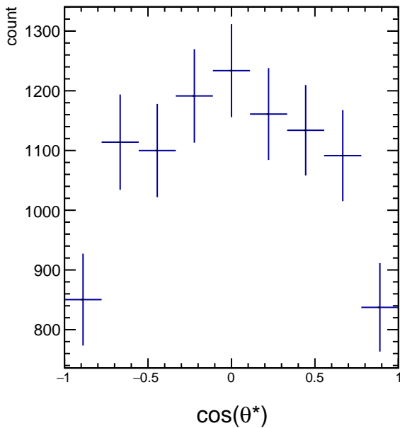
RawYields 2.4 < p_T < 3.0 , 2\pi/6 < \phi' < 3\pi/6
