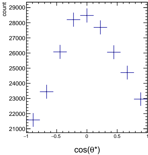
RawYields 1.2 < p_T < 1.8 , 2\pi/6 < \phi' < 3\pi/6
