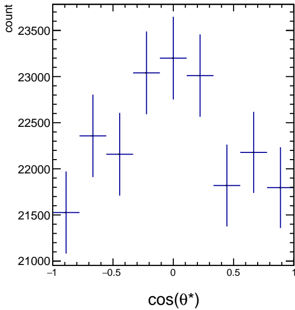
RawYields 1.2 < p_T < 1.8 , 7\pi/6 < \phi' < 8\pi/6
