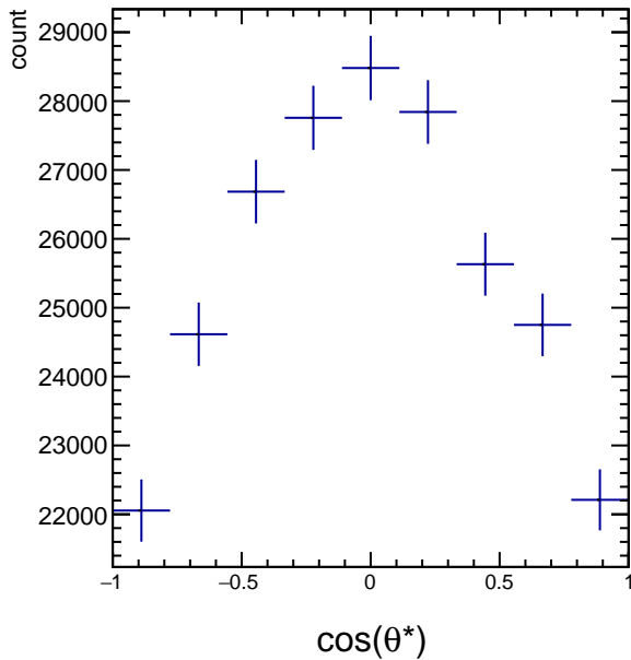
RawYields 1.2 < p_T < 1.8 , 3\pi/6 < \phi' < 4\pi/6
