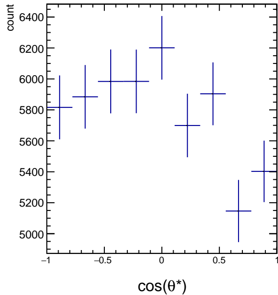
RawYields 1.8 < p_T < 2.4 , 1\pi/6 < \phi' < 2\pi/6
