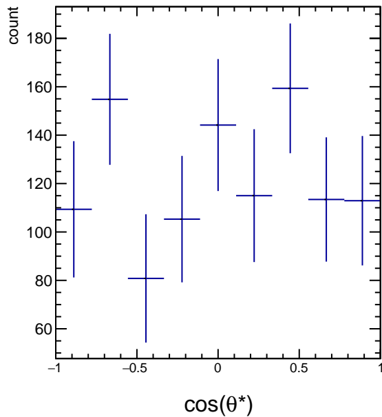
RawYields 3.0 < p_T < 4.2 , 7\pi/6 < \phi' < 8\pi/6
