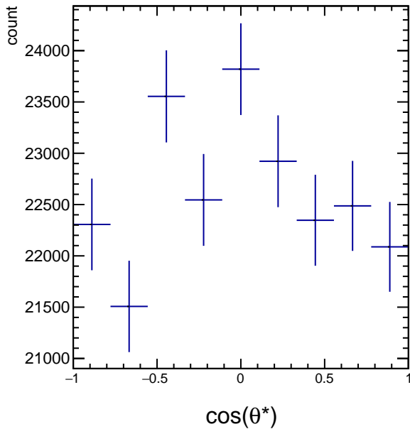
RawYields 1.2 < p_T < 1.8 , 1\pi/6 < \phi' < 2\pi/6
