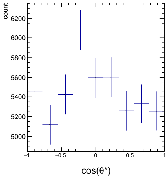
RawYields 1.8 < p_T < 2.4, 11\pi/6 < \phi' < 12\pi/6
