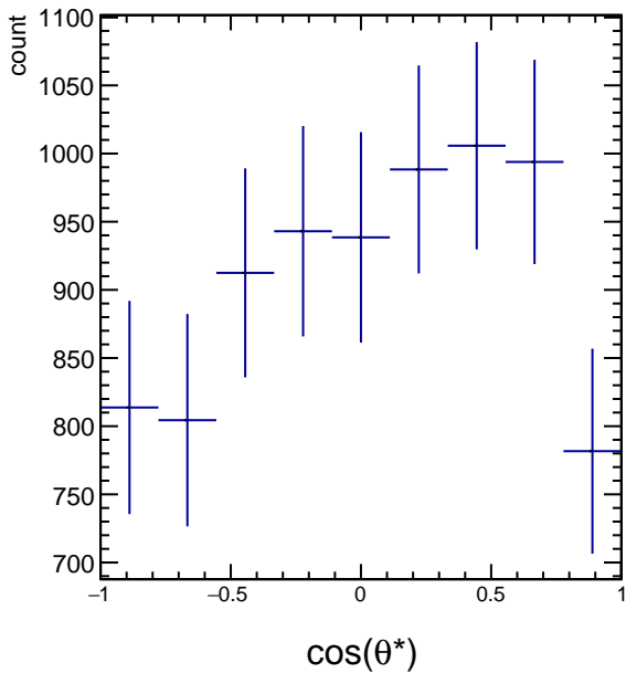
RawYields 2.4 < p_T < 3.0, 11\pi/6 < \phi' < 12\pi/6
