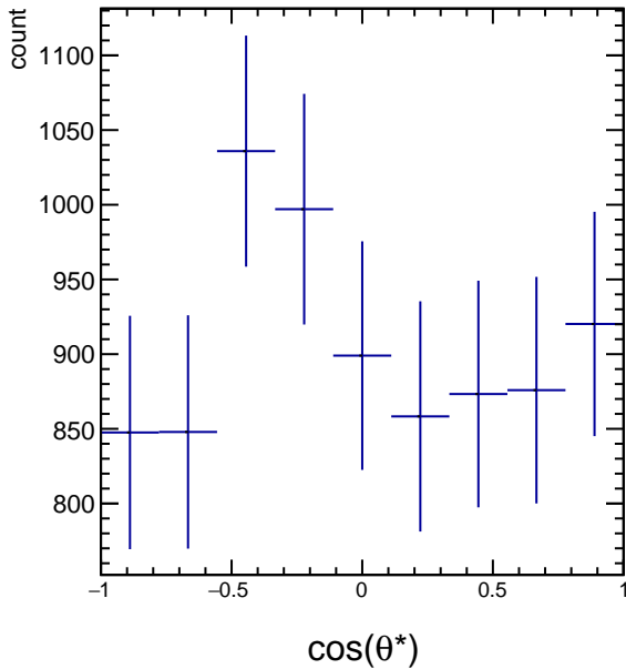
RawYields 2.4 < p_T < 3.0 , 0\pi/6 < \phi' < 1\pi/6
