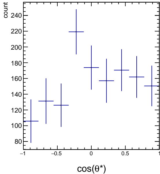
RawYields 3.0 < p_T < 4.2 , 1\pi/6 < \phi' < 2\pi/6
