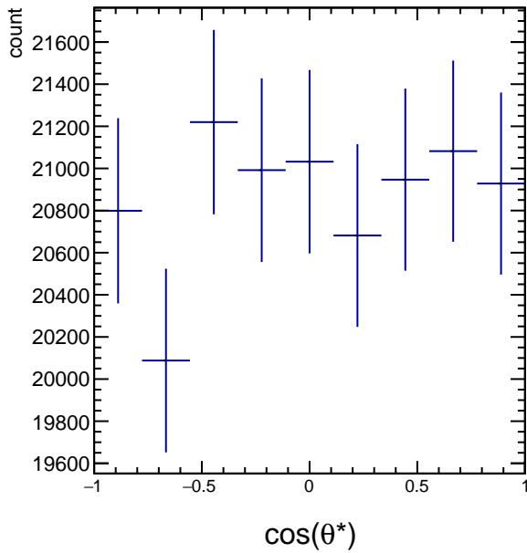
RawYields 1.2 < p_{\text{T}} < 1.8 , 6\pi/6 < \phi' < 7\pi/6
