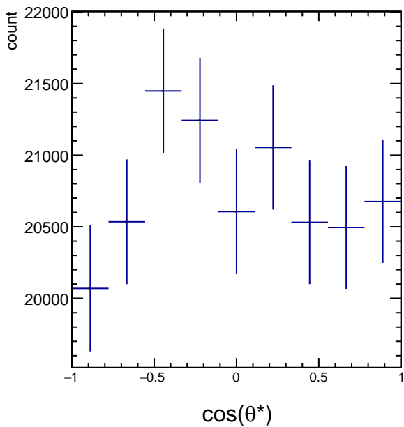
RawYields 1.2 < p_T < 1.8, 11\pi/6 < \phi' < 12\pi/6
