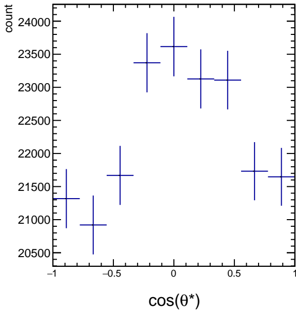
RawYields 1.2 < p_T < 1.8 , 4\pi/6 < \phi' < 5\pi/6
