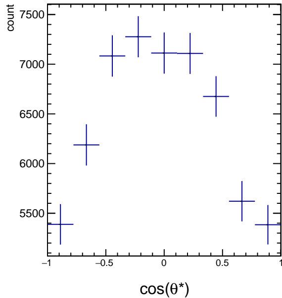
RawYields 1.8 < p_T < 2.4 , 3\pi/6 < \phi' < 4\pi/6
