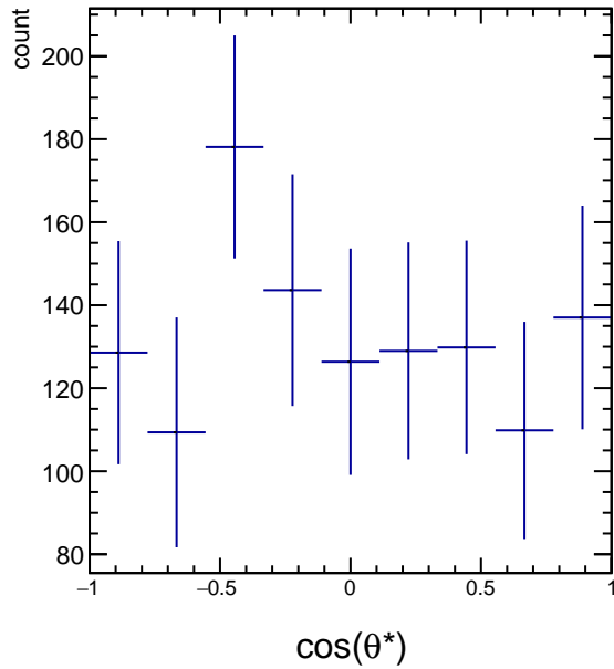
RawYields 3.0 < p_{\text{T}} < 4.2 , 6\pi/6 < \phi' < 7\pi/6
