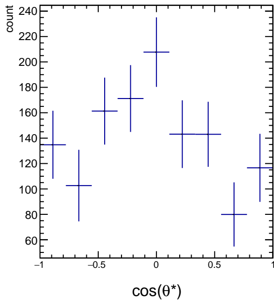
RawYields 3.0 < p_T < 4.2 , 5\pi/6 < \phi' < 6\pi/6
