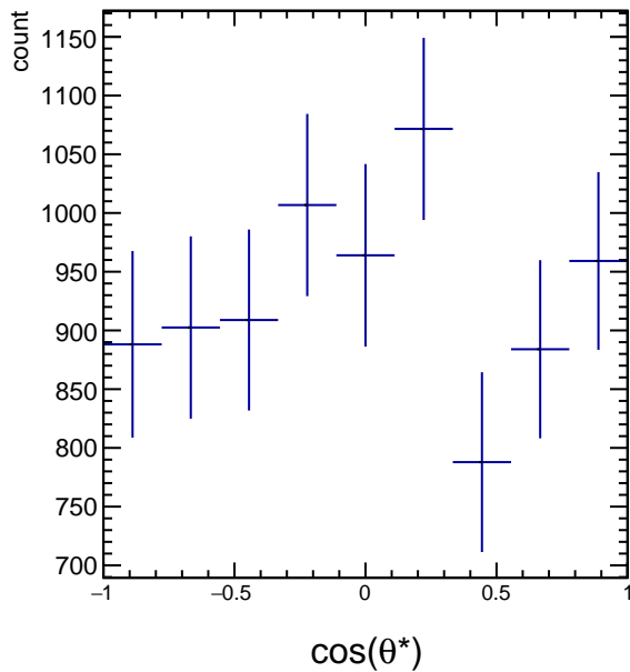
RawYields 2.4 < p_T < 3.0 , 7\pi/6 < \phi' < 8\pi/6
