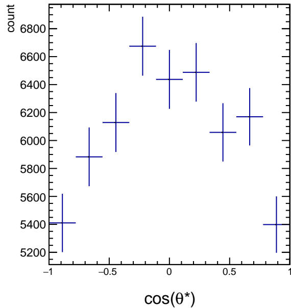
RawYields 1.8 < p_T < 2.4 , 9\pi/6 < \phi' < 10\pi/6
