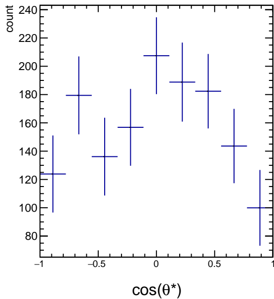
RawYields 3.0 < p_T < 4.2 , 9\pi/6 < \phi' < 10\pi/6
