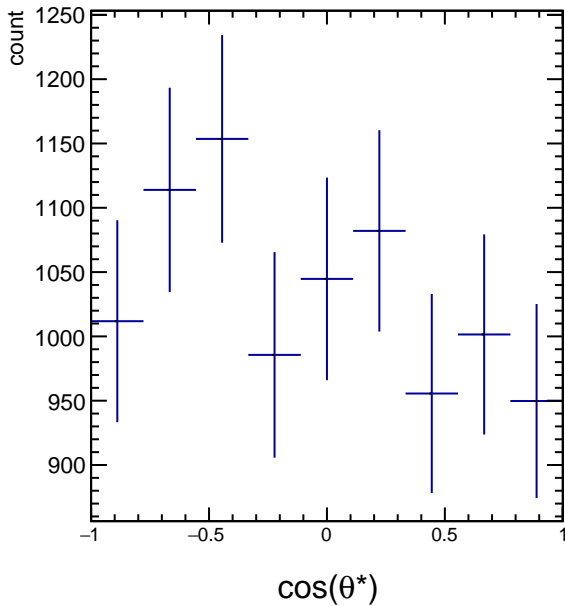
RawYields 2.4 < p_T < 3.0 , 9\pi/6 < \phi' < 10\pi/6
