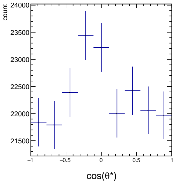
RawYields 1.2 < p_T < 1.8 , 10\pi/6 < \phi' < 11\pi/6
