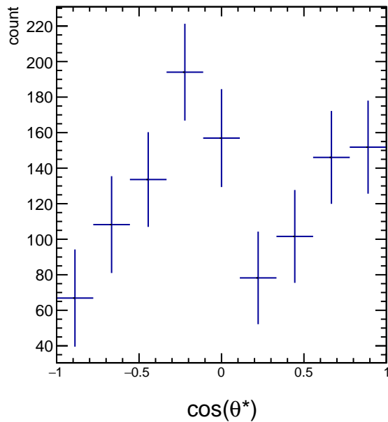
RawYields 3.0 < p_T < 4.2, 11\pi/6 < \phi' < 12\pi/6
