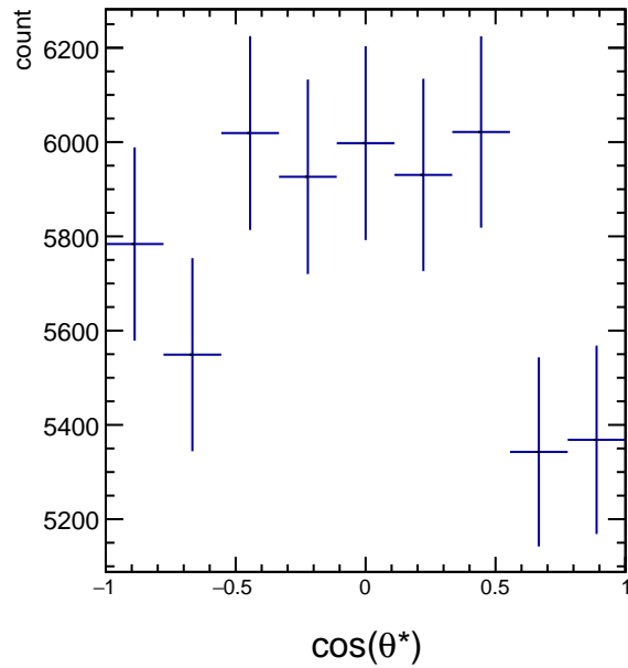
RawYields 1.8 < p_T < 2.4 , 7\pi/6 < \phi' < 8\pi/6
