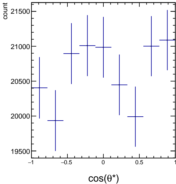
RawYields 1.2 < p_T < 1.8 , 0\pi/6 < \phi' < 1\pi/6
