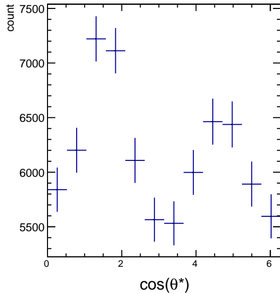
Raw Yields 1.8 < p_T < 2.4 , -0.5/4.5 < \cos(\theta^*) < 0.5/4.5
