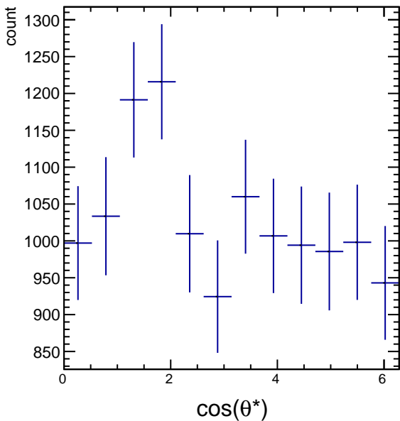
Raw Yields 2.4 < p_T < 3.0 , -1.5/4.5 < \cos(\theta^*) < -0.5/4.5
