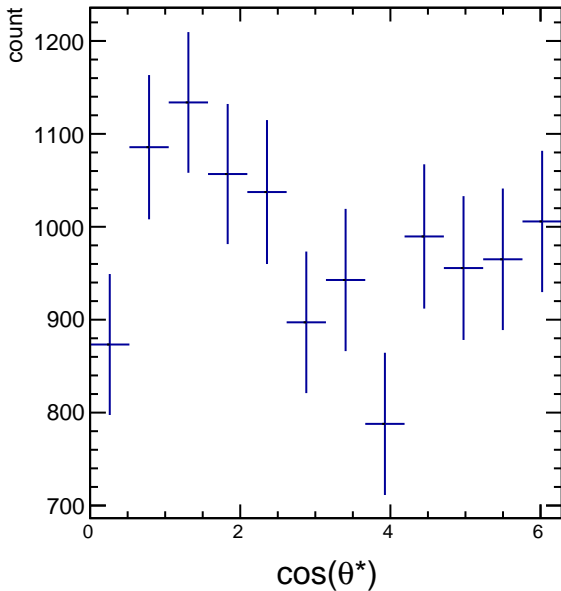
Raw Yields 2.4 < p_T < 3.0, 1.5/4.5 < \cos(\theta^*) < 2.5/4.5
