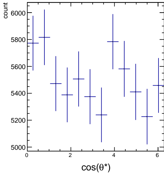
Raw Yields 1.8 < p_T < 2.4 , -4.5/4.5 < \cos(\theta^*) < -3.5/4.5
