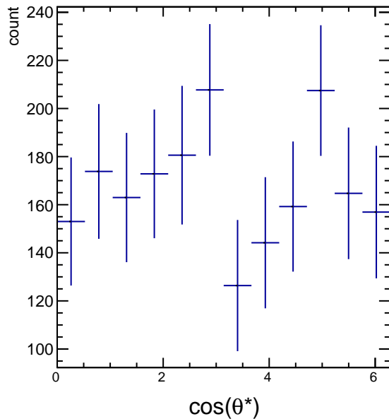
Raw Yields 3.0 < p_T < 4.2 , -0.5/4.5 < \cos(\theta^*) < 0.5/4.5
