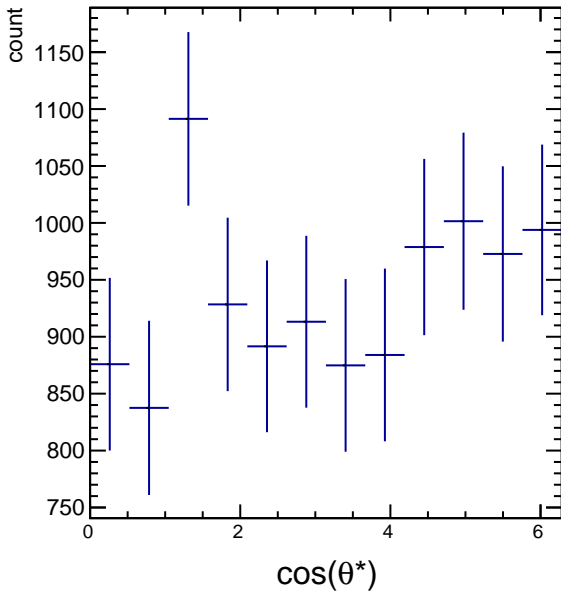
Raw Yields 2.4 < p_T < 3.0 , 2.5/4.5 < \cos(\theta^*) < 3.5/4.5
