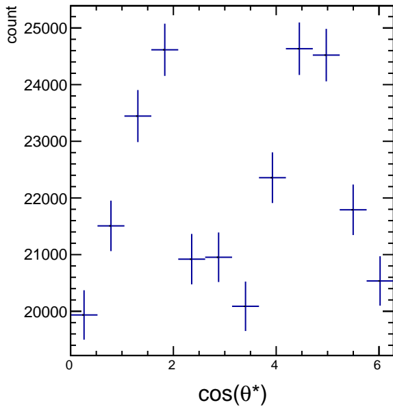
Raw Yields 1.2 < p_T < 1.8 , -3.5/4.5 < \cos(\theta^*) < -2.5/4.5
