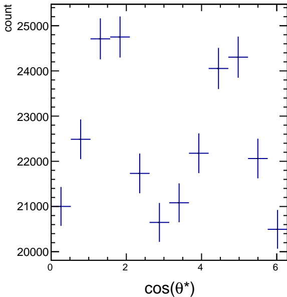
Raw Yields 1.2 < p_T < 1.8 , 2.5/4.5 < \cos(\theta^*) < 3.5/4.5
