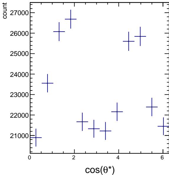
Raw Yields 1.2 < p_T < 1.8 , -2.5/4.5 < \cos(\theta^*) < -1.5/4.5
