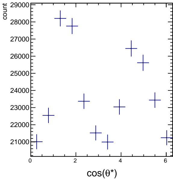
Raw Yields 1.2 < p_T < 1.8 , -1.5/4.5 < \cos(\theta^*) < -0.5/4.5
