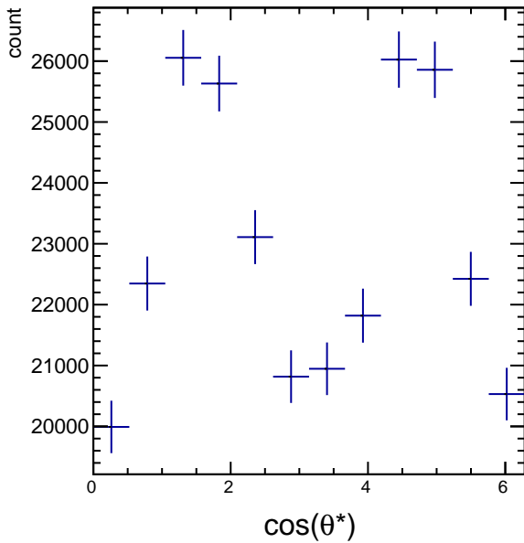
Raw Yields 1.2 < p_T < 1.8, 1.5/4.5 < \cos(\theta^*) < 2.5/4.5
