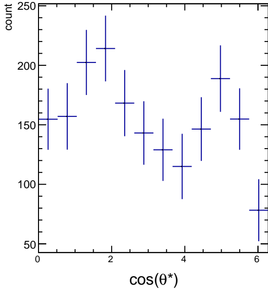
Raw Yields 3.0 < p_T < 4.2 , 0.5/4.5 < \cos(\theta^*) < 1.5/4.5
