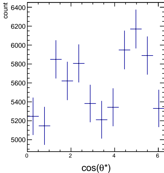
Raw Yields 1.8 < p_T < 2.4 , 2.5/4.5 < \cos(\theta^*) < 3.5/4.5
