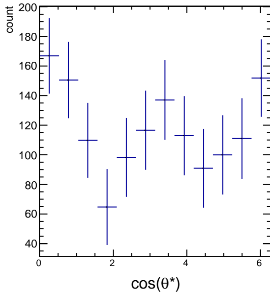
Raw Yields 3.0 < p_T < 4.2 , 3.5/4.5 < \cos(\theta^*) < 4.5/4.5
