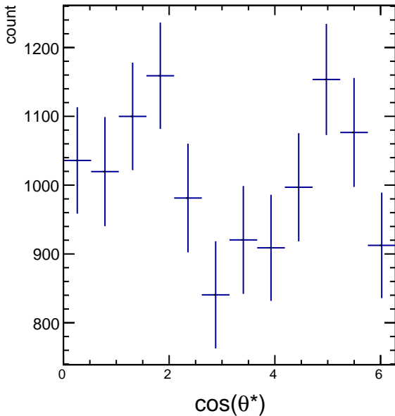
Raw Yields 2.4 < p_T < 3.0 , -2.5/4.5 < \cos(\theta^*) < -1.5/4.5
