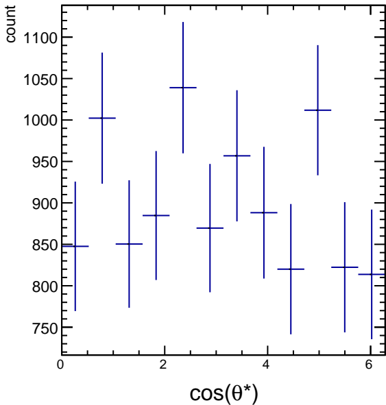
Raw Yields 2.4 < p_T < 3.0 , -4.5/4.5 < \cos(\theta^*) < -3.5/4.5
