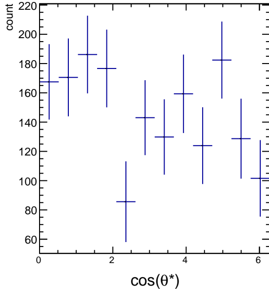
Raw Yields 3.0 < p_T < 4.2, 1.5/4.5 < \cos(\theta^*) < 2.5/4.5
