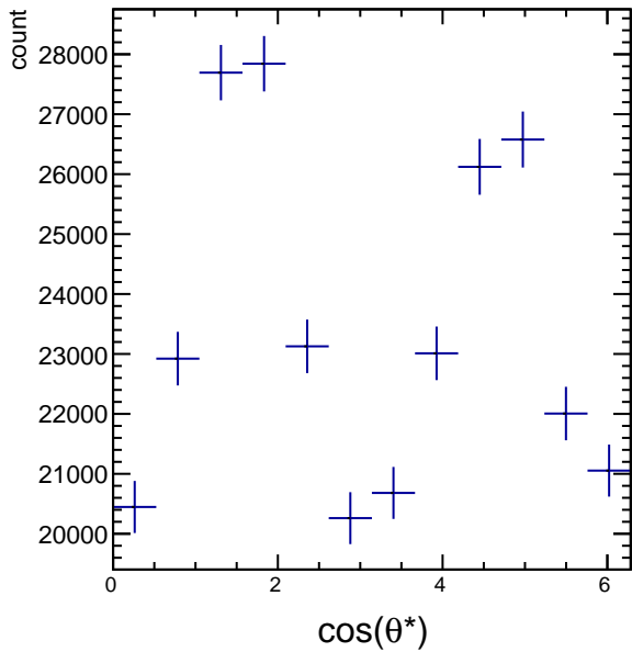
Raw Yields 1.2 < p_T < 1.8 , 0.5/4.5 < \cos(\theta^*) < 1.5/4.5
