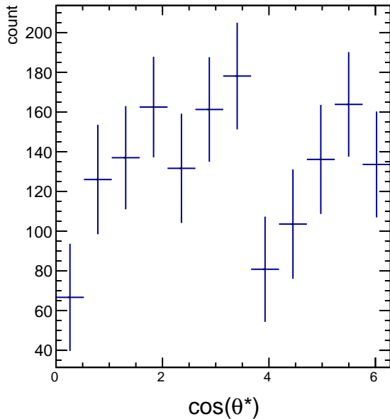
Raw Yields 3.0 < p_T < 4.2 , -2.5/4.5 < \cos(\theta^*) < -1.5/4.5
