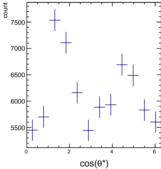
Raw Yields 1.8 < p_T < 2.4 , 0.5/4.5 < \cos(\theta^*) < 1.5/4.5
