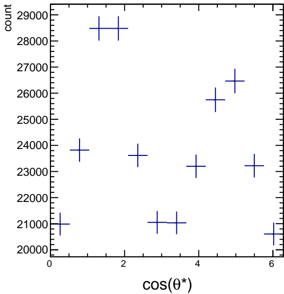
Raw Yields 1.2 < p_T < 1.8 , -0.5/4.5 < \cos(\theta^*) < 0.5/4.5
