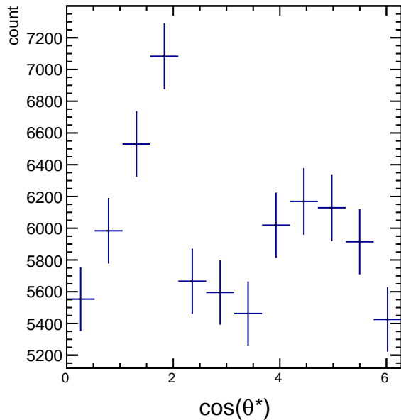
Raw Yields 1.8 < p_T < 2.4 , -2.5/4.5 < \cos(\theta^*) < -1.5/4.5
