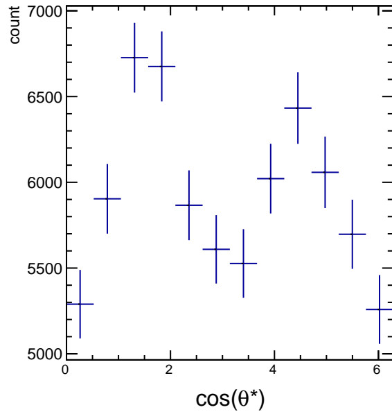
Raw Yields 1.8 < p_T < 2.4, 1.5/4.5 < \cos(\theta^*) < 2.5/4.5
