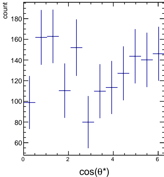
Raw Yields 3.0 < p_T < 4.2 , 2.5/4.5 < \cos(\theta^*) < 3.5/4.5
