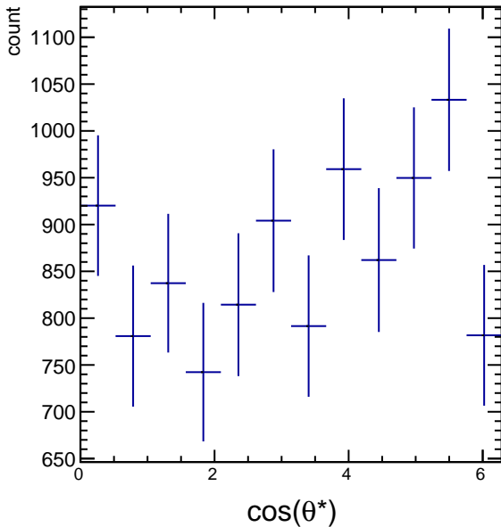
Raw Yields 2.4 < p_T < 3.0 , 3.5/4.5 < \cos(\theta^*) < 4.5/4.5
