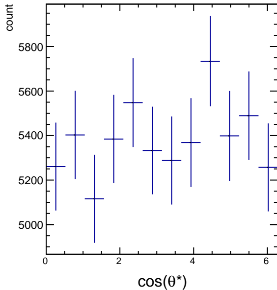
Raw Yields 1.8 < p_T < 2.4 , 3.5/4.5 < \cos(\theta^*) < 4.5/4.5
