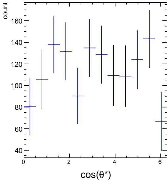
Raw Yields 3.0 < p_T < 4.2 , -4.5/4.5 < \cos(\theta^*) < -3.5/4.5
