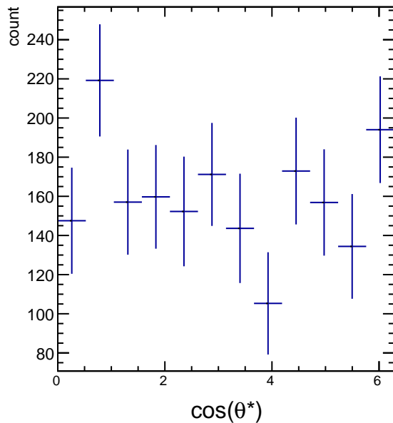
Raw Yields 3.0 < p_T < 4.2 , -1.5/4.5 < \cos(\theta^*) < -0.5/4.5
