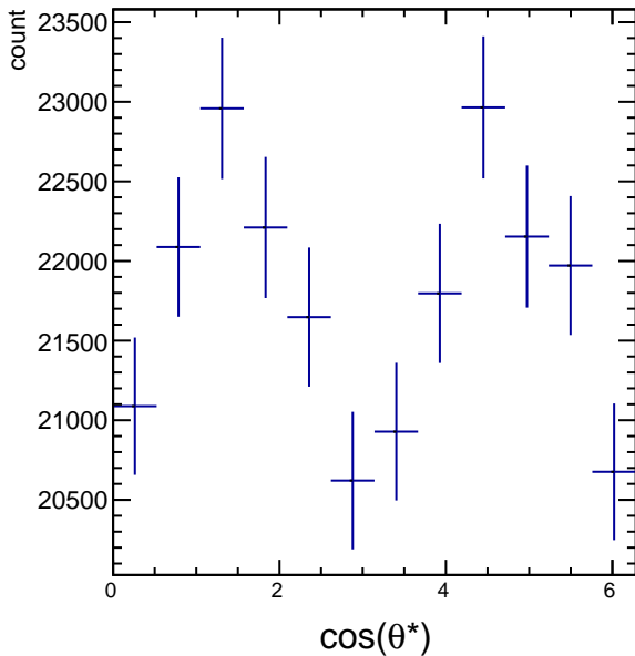
Raw Yields 1.2 < p_T < 1.8 , 3.5/4.5 < \cos(\theta^*) < 4.5/4.5
