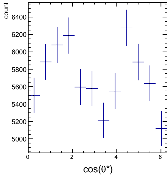
Raw Yields 1.8 < p_T < 2.4 , -3.5/4.5 < \cos(\theta^*) < -2.5/4.5
