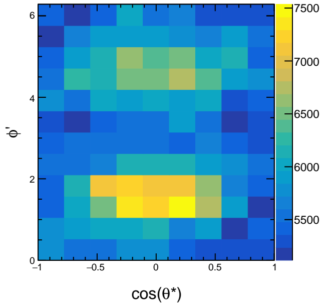
Raw Yields 1.8 < p_T < 2.4
