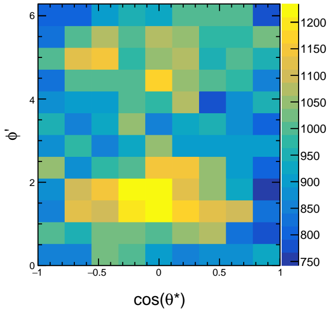
Raw Yields 2.4 < p_T < 3.0
