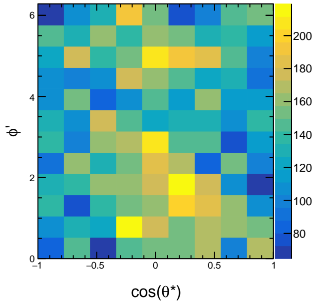
Raw Yields 3.0 < p_T < 4.2
