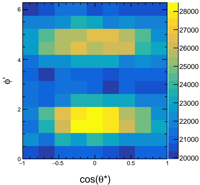
Raw Yields 1.2 < p_T < 1.8
