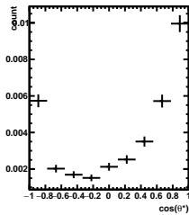
Efficiency -5/5 < y < -4/5 , 5\pi/6 < \phi' < 6\pi/6
