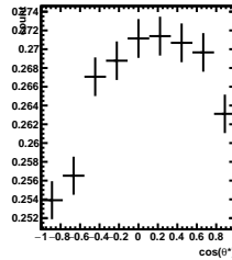
Efficiency 2/5 < y < 3/5, 9\pi/6 < \phi' < 10\pi/6
