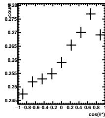
Efficiency -3/5 < y < -2/5 , 7\pi/6 < \phi' < 8\pi/6
