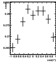
Efficiency -3/5 < y < -2/5, 3\pi/6 < \phi' < 4\pi/6
