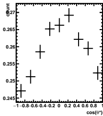
Efficiency -1/5 < y < 0/5 , 6\pi/6 < \phi' < 7\pi/6
