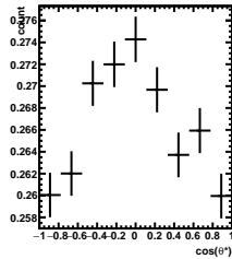
Efficiency 1/5 < y < 2/5 , 7\pi/6 < \phi' < 8\pi/6
