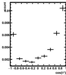
Efficiency -5/5 < y < -4/5 , 6\pi/6 < \phi' < 7\pi/6
