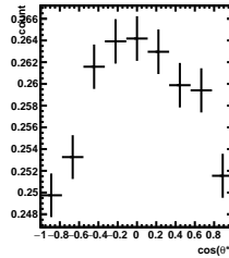
Efficiency -1/5 < y < 0/5, 9\pi/6 < \phi' < 10\pi/6
