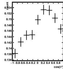
Efficiency -4/5 < y < -3/5 , 8\pi/6 < \phi' < 9\pi/6
