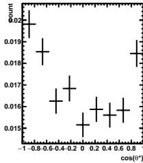
Efficiency -5/5 < y < -4/5, 9\pi/6 < \phi' < 10\pi/6
