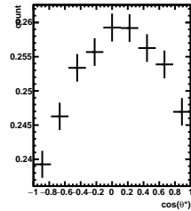
Efficiency 0/5 < y < 1/5, 1\pi/6 < \phi' < 2\pi/6
