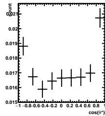
Efficiency -5/5 < y < -4/5 , 8\pi/6 < \phi' < 9\pi/6
