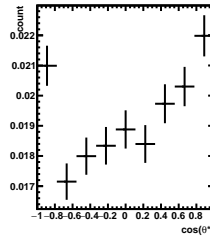
Efficiency 4/5 < y < 5/5, 9\pi/6 < \phi' < 10\pi/6
