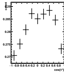
Efficiency -2/5 < y < -1/5 , 7\pi/6 < \phi' < 8\pi/6
