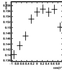
Efficiency 3/5 < y < 4/5, 9\pi/6 < \phi' < 10\pi/6
