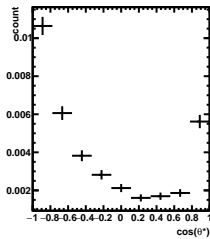
Efficiency -5/5 < y < -4/5 , 0\pi/6 < \phi' < 1\pi/6
