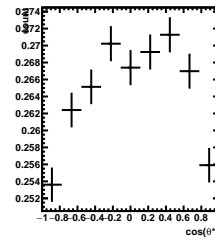
Efficiency 1/5 < y < 2/5 , 4\pi/6 < \phi' < 5\pi/6
