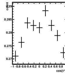
Efficiency -2/5 < y < -1/5 , 2\pi/6 < \phi' < 3\pi/6
