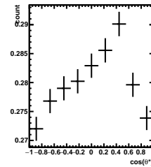
Efficiency -2/5 < y < -1/5 , 4\pi/6 < \phi' < 5\pi/6
