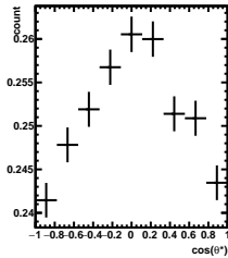
Efficiency 0/5 < y < 1/5 , 6\pi/6 < \phi' < 7\pi/6
