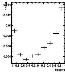
Efficiency -5/5 < y < -4/5 , 4\pi/6 < \phi' < 5\pi/6
