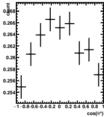
Efficiency 1/5 < y < 2/5 , 6\pi/6 < \phi' < 7\pi/6
