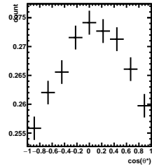
Efficiency 1/5 < y < 2/5, 3\pi/6 < \phi' < 4\pi/6
