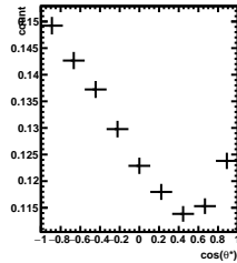
Efficiency 3/5 < y < 4/5 , 7\pi/6 < \phi' < 8\pi/6
