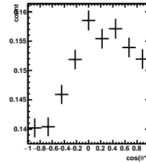
Efficiency 3/5 < y < 4/5 , 2\pi/6 < \phi' < 3\pi/6
