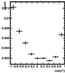
Efficiency 4/5 < y < 5/5 , 6\pi/6 < \phi' < 7\pi/6
