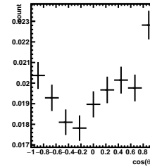
Efficiency 4/5 < y < 5/5 , 2\pi/6 < \phi' < 3\pi/6
