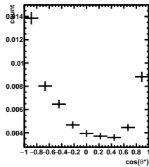
Efficiency -5/5 < y < -4/5, 10\pi/6 < \phi' < 11\pi/6
