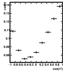
Efficiency -4/5 < y < -3/5 , 6\pi/6 < \phi' < 7\pi/6
