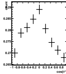
Efficiency -3/5 < y < -2/5, 9\pi/6 < \phi' < 10\pi/6
