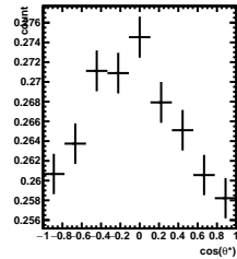
Efficiency 2/5 < y < 3/5, 3\pi/6 < \phi' < 4\pi/6
