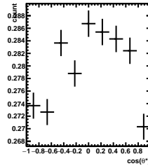
Efficiency -2/5 < y < -1/5, 9\pi/6 < \phi' < 10\pi/6
