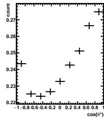
Efficiency -3/5 < y < -2/5 , 6\pi/6 < \phi' < 7\pi/6
