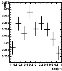
Efficiency 1/5 < y < 2/5 , 5\pi/6 < \phi' < 6\pi/6
