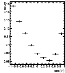
Efficiency 3/5 < y < 4/5 , 6\pi/6 < \phi' < 7\pi/6
