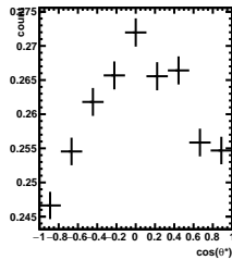
Efficiency -1/5 < y < 0/5 , 7\pi/6 < \phi' < 8\pi/6
