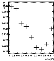
Efficiency 2/5 < y < 3/5 , 5\pi/6 < \phi' < 6\pi/6
