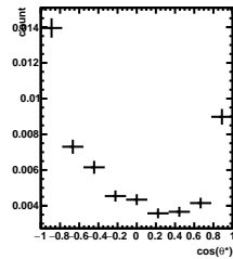
Efficiency -5/5 < y < -4/5, 1\pi/6 < \phi' < 2\pi/6
