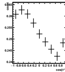
Efficiency 2/5 < y < 3/5 , 4\pi/6 < \phi' < 5\pi/6
