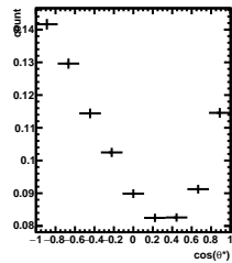
Efficiency 3/5 < y < 4/5 , 5\pi/6 < \phi' < 6\pi/6
