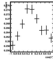
Efficiency 2/5 < y < 3/5 , 8\pi/6 < \phi' < 9\pi/6
