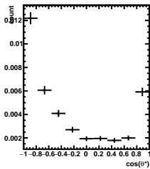
Efficiency 4/5 < y < 5/5 , 5\pi/6 < \phi' < 6\pi/6
