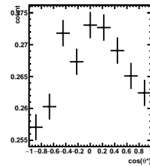
Efficiency 1/5 < y < 2/5 , 8\pi/6 < \phi' < 9\pi/6
