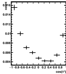
Efficiency 4/5 < y < 5/5 , 7\pi/6 < \phi' < 8\pi/6
