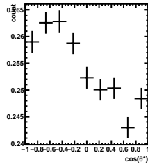
Efficiency 2/5 < y < 3/5 , 7\pi/6 < \phi' < 8\pi/6
