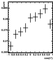
Efficiency -2/5 < y < -1/5 , 6\pi/6 < \phi' < 7\pi/6
