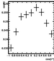
Efficiency 0/5 < y < 1/5, 9\pi/6 < \phi' < 10\pi/6
