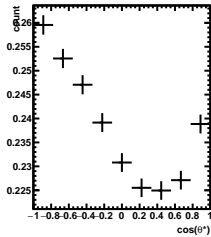
Efficiency 2/5 < y < 3/5 , 6\pi/6 < \phi' < 7\pi/6
