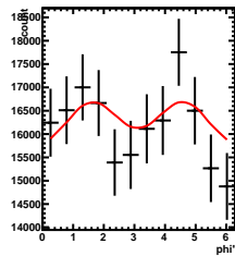
Corrected Yields 1/5 < y < 2/5 , 1.5/4.5 < \cos(\theta^*) < 2.5/4.5
