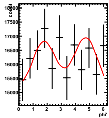
Corrected Yields -3/5 < y < 2/5 , -2.5/4.5 < \cos(\theta^*) < -1.5/4.5
