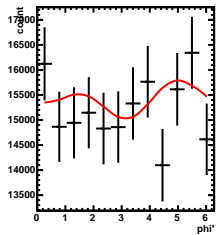
Corrected Yields -1/5 < \gamma < 0/5 , 3.5/4.5 < \cos(\theta^*) < 4.5/4.5
