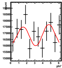
Corrected Yields 0/5 < y < 1/5 , -2.5/4.5 < \cos(\theta^*) < -1.5/4.5
