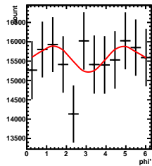
Corrected Yields 1/5 < y < 2/5, -3.5/4.5 < \cos(\theta^*) < -2.5/4.5
