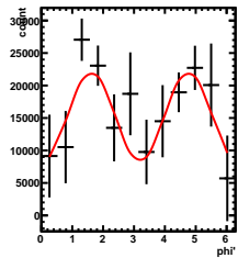
Corrected Yields -5/5 < y < -4/5, -0.5/4.5 < \cos(\theta^*) < 0.5/4.5
