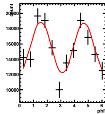
Corrected Yields 3/5 < y < 4/5, -1.5/4.5 < \cos(\theta^*) < 0.5/4.5
