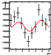
Corrected Yields -4/5 < \gamma < 3/5 , 3.5/4.5 < \cos(\theta^*) < 4.5/4.5
