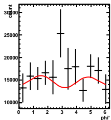
Corrected Yields 4/5 < \gamma < 5/5 , 3.5/4.5 < \cos(\theta^*) < 4.5/4.5
