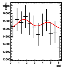
Corrected Yields 0/5 < \gamma < 1/5 , 3.5/4.5 < \cos(\theta^*) < 4.5/4.5
