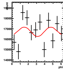
Corrected Yields 1/5 < y < 2/5, -1.5/4.5 < \cos(\theta^*) < 0.5/4.5
