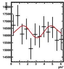
Corrected Yields 1/5 < y < 2/5 , -2.5/4.5 < \cos(\theta^*) < -1.5/4.5
