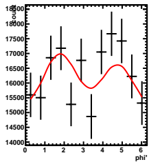
Corrected Yields -1/5 < y < 0/5, -3.5/4.5 < \cos(\theta^*) < -2.5/4.5
