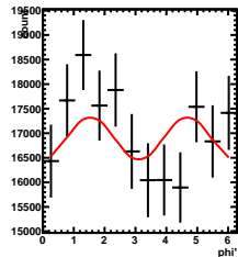
Corrected Yields 1/5 < y < 2/5, -0.5/4.5 < \cos(\theta^*) < 0.5/4.5
