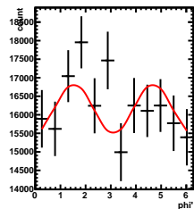
Corrected Yields 2/5 < y < 3/5, -0.5/4.5 < \cos(\theta^*) < 0.5/4.5
