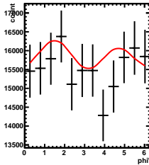
Corrected Yields -2/5 < y < 1/5 , 2.5/4.5 < \cos(\theta^*) < 3.5/4.5
