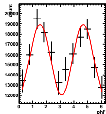
Corrected Yields 3/5 < y < 4/5, -0.5/4.5 < \cos(\theta^*) < 0.5/4.5
