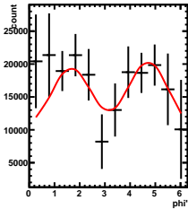
Corrected Yields -5/5 < y < 4/5 , 2.5/4.5 < \cos(\theta^*) < 3.5/4.5
