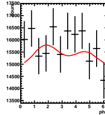
Corrected Yields -1/5 < y < 0/5 , -4.5/4.5 < \cos(\theta^*) < -3.5/4.5
