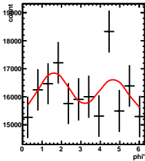
Corrected Yields 0/5 < y < 1/5 , 2.5/4.5 < \cos(\theta^*) < 3.5/4.5
