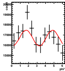
Corrected Yields -3/5 < y < -2/5, -0.5/4.5 < \cos(\theta^*) < 0.5/4.5
