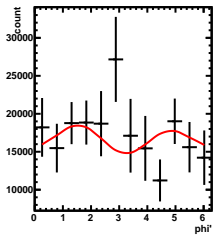
Corrected Yields -5/5 < y < -4/5 , -4.5/4.5 < \cos(\theta^*) < -3.5/4.5
