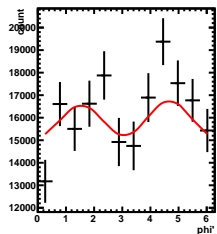
Corrected Yields 3/5 < \gamma < 4/5 , 3.5/4.5 < \cos(\theta^*) < 4.5/4.5
