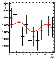
Corrected Yields -3/5 < \gamma < 2/5 , 3.5/4.5 < \cos(\theta^*) < 4.5/4.5
