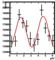
Corrected Yields 3/5 < y < 4/5 , 1.5/4.5 < \cos(\theta^*) < 2.5/4.5
