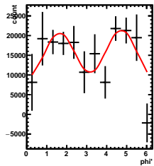
Corrected Yields -5/5 < y < 4/5 , 1.5/4.5 < \cos(\theta^*) < 2.5/4.5
