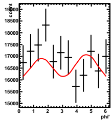
Corrected Yields -2/5 < y < 1/5 , -2.5/4.5 < \cos(\theta^*) < -1.5/4.5
