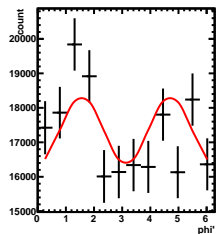
Corrected Yields 0/5 < y < 1/5, -0.5/4.5 < \cos(\theta^*) < 0.5/4.5
