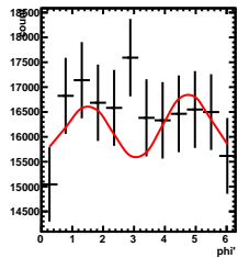
Corrected Yields 0/5 < y < 1/5, -3.5/4.5 < \cos(\theta^*) < -2.5/4.5
