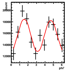
Corrected Yields 3/5 < y < 4/5 , -2.5/4.5 < \cos(\theta^*) < -1.5/4.5
