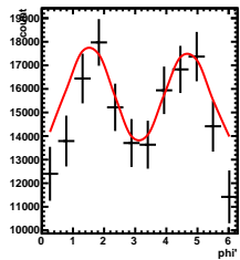
Corrected Yields 3/5 < y < 4/5, -3.5/4.5 < \cos(\theta^*) < -2.5/4.5
