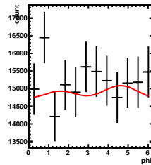
Corrected Yields -2/5 < y < -1/5 , -4.5/4.5 < \cos(\theta^*) < -3.5/4.5
