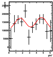
Corrected Yields 4/5 < y < 5/5, -3.5/4.5 < \cos(\theta^*) < -2.5/4.5
