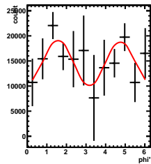
Corrected Yields 4/5 < y < 5/5 , 1.5/4.5 < \cos(\theta^*) < 2.5/4.5
