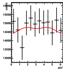
Corrected Yields 1/5 < \gamma < 2/5 , 3.5/4.5 < \cos(\theta^*) < 4.5/4.5
