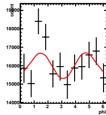
Corrected Yields 2/5 < y < 3/5, -1.5/4.5 < \cos(\theta^*) < 0.5/4.5
