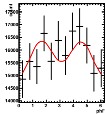
Corrected Yields 2/5 < y < 3/5 , 1.5/4.5 < \cos(\theta^*) < 2.5/4.5
