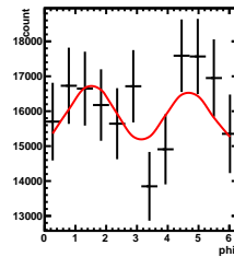
Corrected Yields 3/5 < y < 4/5 , -4.5/4.5 < \cos(\theta^*) < -3.5/4.5
