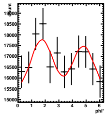
Corrected Yields -1/5 < y < 0/5 , -2.5/4.5 < \cos(\theta^*) < -1.5/4.5
