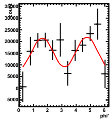
Corrected Yields -5/5 < y < 4/5 , 0.5/4.5 < \cos(\theta^*) < 1.5/4.5
