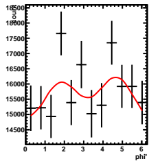
Corrected Yields -3/5 < y < 2/5, -3.5/4.5 < \cos(\theta^*) < -2.5/4.5
