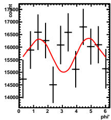
Corrected Yields 2/5 < y < 3/5 , -2.5/4.5 < \cos(\theta^*) < -1.5/4.5
