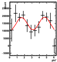
Corrected Yields 4/5 < y < 5/5 , -2.5/4.5 < \cos(\theta^*) < -1.5/4.5
