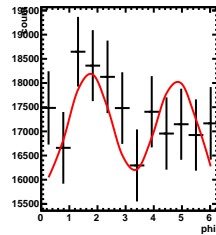
Corrected Yields -1/5 < y < 0/5, -1.5/4.5 < \cos(\theta^*) < 0.5/4.5
