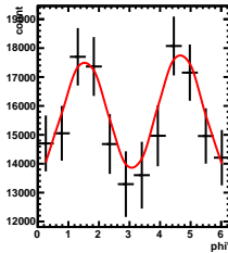
Corrected Yields 3/5 < y < 4/5 , 2.5/4.5 < \cos(\theta^*) < 3.5/4.5
