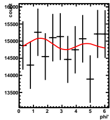
Corrected Yields -2/5 < \gamma < 1/5 , 3.5/4.5 < \cos(\theta^*) < 4.5/4.5
