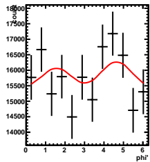
Corrected Yields -2/5 < y < 1/5, -3.5/4.5 < \cos(\theta^*) < -2.5/4.5
