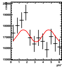
Corrected Yields -2/5 < y < -1/5, -0.5/4.5 < \cos(\theta^*) < 0.5/4.5
