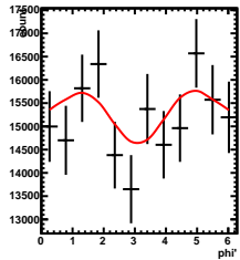
Corrected Yields 2/5 < y < 3/5, -3.5/4.5 < \cos(\theta^*) < -2.5/4.5
