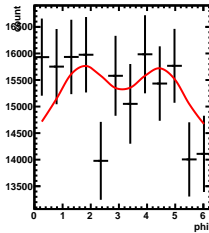
Corrected Yields 2/5 < y < 3/5 , 2.5/4.5 < \cos(\theta^*) < 3.5/4.5
