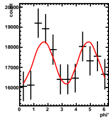
Corrected Yields -1/5 < y < 0/5, -0.5/4.5 < \cos(\theta^*) < 0.5/4.5
