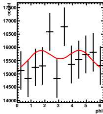
Corrected Yields 1/5 < y < 2/5 , 2.5/4.5 < \cos(\theta^*) < 3.5/4.5
