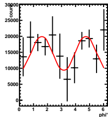
Corrected Yields 4/5 < y < 5/5, -0.5/4.5 < \cos(\theta^*) < 0.5/4.5
