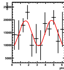
Corrected Yields 4/5 < y < 5/5, -1.5/4.5 < \cos(\theta^*) < 0.5/4.5
