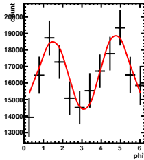
Corrected Yields -4/5 < y < 3/5 , 2.5/4.5 < \cos(\theta^*) < 3.5/4.5
