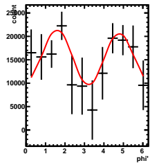
Corrected Yields -5/5 < y < 4/5 , -2.5/4.5 < \cos(\theta^*) < -1.5/4.5
