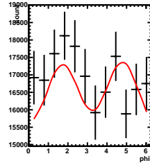
Corrected Yields -3/5 < y < 2/5, -1.5/4.5 < \cos(\theta^*) < 0.5/4.5
