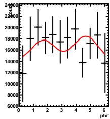
Corrected Yields -5/5 < \gamma < 4/5 , 3.5/4.5 < \cos(\theta^*) < 4.5/4.5
