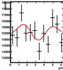
Corrected Yields -3/5 < y < 2/5 , 2.5/4.5 < \cos(\theta^*) < 3.5/4.5
