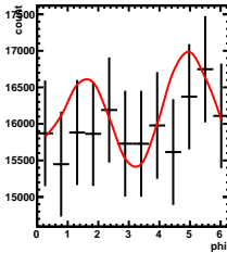
Corrected Yields -1/5 < y < 0/5 , 2.5/4.5 < \cos(\theta^*) < 3.5/4.5
