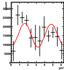
Corrected Yields -5/5 < y < 4/5, -1.5/4.5 < \cos(\theta^*) < 0.5/4.5
