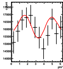
Corrected Yields -3/5 < y < 2/5 , 1.5/4.5 < \cos(\theta^*) < 2.5/4.5
