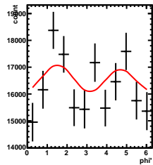
Corrected Yields -2/5 < y < 1/5 , 1.5/4.5 < \cos(\theta^*) < 2.5/4.5
