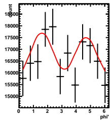
Corrected Yields 0/5 < y < 1/5 , 1.5/4.5 < \cos(\theta^*) < 2.5/4.5
