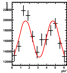
Corrected Yields -4/5 < y < -3/5, -0.5/4.5 < \cos(\theta^*) < 0.5/4.5
