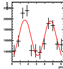
Corrected Yields -4/5 < y < 3/5, -1.5/4.5 < \cos(\theta^*) < 0.5/4.5
