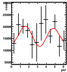
Corrected Yields -5/5 < y < 4/5, -3.5/4.5 < \cos(\theta^*) < -2.5/4.5
