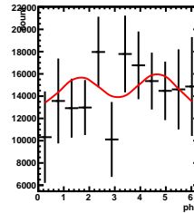
Corrected Yields 4/5 < y < 5/5 , -4.5/4.5 < \cos(\theta^*) < -3.5/4.5
