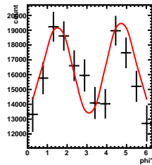
Corrected Yields -4/5 < y < 3/5 , 1.5/4.5 < \cos(\theta^*) < 2.5/4.5
