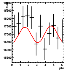
Corrected Yields -2/5 < y < 1/5, -1.5/4.5 < \cos(\theta^*) < 0.5/4.5
