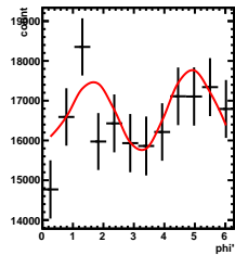
Corrected Yields -1/5 < y < 0/5 , 1.5/4.5 < \cos(\theta^*) < 2.5/4.5
