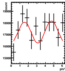
Corrected Yields 0/5 < y < 1/5, -1.5/4.5 < \cos(\theta^*) < 0.5/4.5
