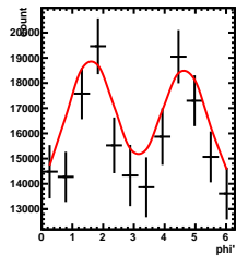
Corrected Yields -4/5 < y < 3/5, -3.5/4.5 < \cos(\theta^*) < -2.5/4.5
