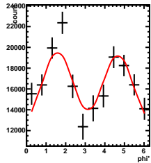
Corrected Yields -4/5 < y < 3/5 , -2.5/4.5 < \cos(\theta^*) < -1.5/4.5
