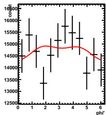
Corrected Yields 2/5 < \gamma < 3/5 , 3.5/4.5 < \cos(\theta^*) < 4.5/4.5
