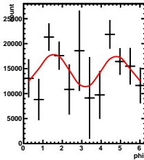
Corrected Yields 4/5 < y < 5/5 , 2.5/4.5 < \cos(\theta^*) < 3.5/4.5
