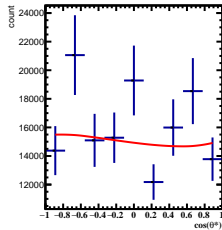
Corrected Yields 2/5 < y < 3/5 , 9\pi/6 < \phi < 10\pi/6
