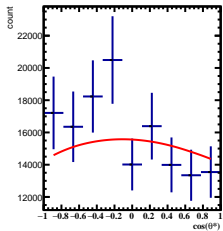
Corrected Yields 0/5 < y < 1/5 , 11\pi/6 < \phi < 12\pi/6
