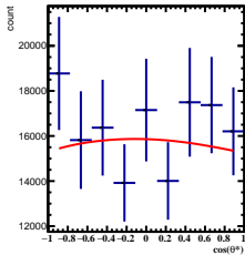
Corrected Yields 2/5 < y < 3/5 , 1\pi/6 < \phi < 2\pi/6
