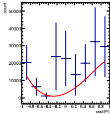
Corrected Yields -5/5 < y < -4/5 , 6\pi/6 < \phi < 7\pi/6
