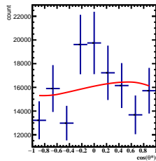
Corrected Yields -1/5 < y < 0/5 , 11\pi/6 < \phi < 12\pi/6
