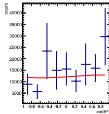
Corrected Yields 4/5 < y < 5/5 , 10\pi/6 < \phi < 11\pi/6
