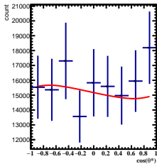
Corrected Yields 2/5 < y < 3/5 , 11\pi/6 < \phi < 12\pi/6
