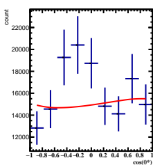
Corrected Yields 2/5 < y < 3/5 , 3\pi/6 < \phi < 4\pi/6
