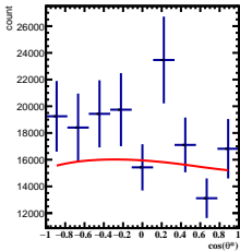
Corrected Yields 1/5 < y < 2/5 , 1\pi/6 < \phi < 2\pi/6
