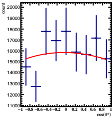
Corrected Yields -2/5 < y < -1/5 , 4\pi/6 < \phi < 5\pi/6
