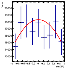
Corrected Yields 0/5 < y < 1/5 , 2\pi/6 < \phi < 3\pi/6
