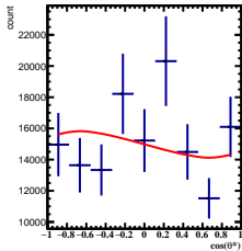
Corrected Yields -3/5 < y < -2/5 , 6\pi/6 < \phi < 7\pi/6
