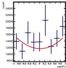
Corrected Yields 3/5 < y < 4/5 , 11\pi/6 < \phi < 12\pi/6
