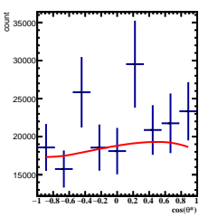
Corrected Yields -4/5 < y < -3/5 , 8\pi/6 < \phi < 9\pi/6
