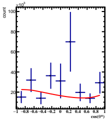
Corrected Yields -5/5 < y < -4/5 , 2\pi/6 < \phi < 3\pi/6
