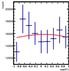
Corrected Yields 2/5 < y < 3/5 , 7\pi/6 < \phi < 8\pi/6
