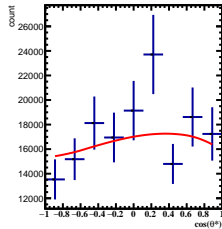
Corrected Yields -1/5 < y < 0/5 , 9\pi/6 < \phi < 10\pi/6
