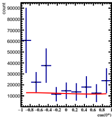
Corrected Yields 4/5 < y < 5/5 , 4\pi/6 < \phi < 5\pi/6
