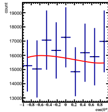
Corrected Yields -1/5 < y < 0/5 , 6\pi/6 < \phi < 7\pi/6
