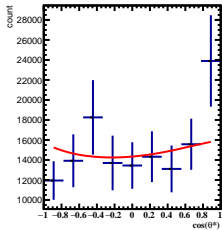
Corrected Yields 3/5 < y < 4/5 , 1\pi/6 < \phi < 2\pi/6
