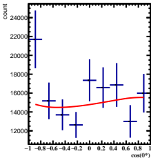
Corrected Yields 2/5 < y < 3/5 , 4\pi/6 < \phi < 5\pi/6
