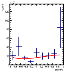
Corrected Yields -5/5 < y < -4/5 , 8\pi/6 < \phi < 9\pi/6
