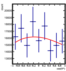
Corrected Yields -3/5 < y < -2/5 , 8\pi/6 < \phi < 9\pi/6
