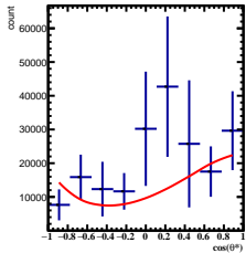
Corrected Yields -5/5 < y < -4/5 , 7\pi/6 < \phi < 8\pi/6
