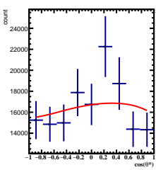
Corrected Yields -1/5 < y < 0/5 , 8\pi/6 < \phi < 9\pi/6
