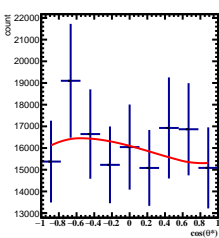
Corrected Yields -1/5 < y < 0/5 , 5\pi/6 < \phi < 6\pi/6
