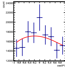
Corrected Yields -2/5 < y < -1/5 , 6\pi/6 < \phi < 7\pi/6
