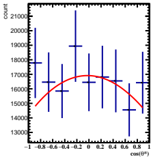
Corrected Yields 0/5 < y < 1/5 , 1\pi/6 < \phi < 2\pi/6
