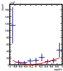
Corrected Yields -5/5 < y < -4/5 , 5\pi/6 < \phi < 6\pi/6
