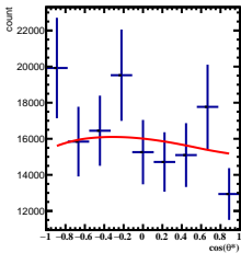
Corrected Yields 1/5 < y < 2/5 , 10\pi/6 < \phi < 11\pi/6
