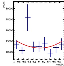
Corrected Yields 3/5 < y < 4/5 , 6\pi/6 < \phi < 7\pi/6
