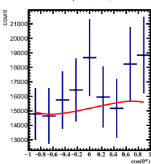
Corrected Yields 2/5 < y < 3/5 , 5\pi/6 < \phi < 6\pi/6
