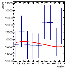
Corrected Yields 1/5 < y < 2/5 , 11\pi/6 < \phi < 12\pi/6
