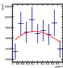
Corrected Yields -3/5 < y < -2/5 , 3\pi/6 < \phi < 4\pi/6
