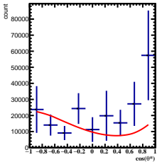
Corrected Yields -5/5 < y < -4/5 , 1\pi/6 < \phi < 2\pi/6
