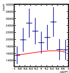
Corrected Yields 3/5 < y < 4/5 , 3\pi/6 < \phi < 4\pi/6
