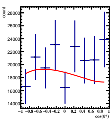
Corrected Yields -4/5 < y < -3/5 , 2\pi/6 < \phi < 3\pi/6
