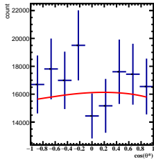
Corrected Yields -1/5 < y < 0/5 , 7\pi/6 < \phi < 8\pi/6
