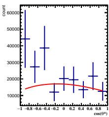
Corrected Yields 4/5 < y < 5/5 , 8\pi/6 < \phi < 9\pi/6
