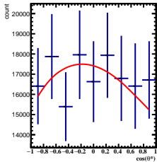
Corrected Yields -2/5 < y < -1/5 , 7\pi/6 < \phi < 8\pi/6
