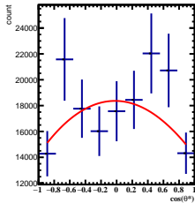
Corrected Yields 0/5 < y < 1/5 , 9\pi/6 < \phi < 10\pi/6
