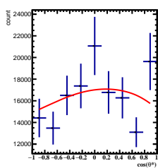
Corrected Yields -2/5 < y < -1/5 , 2\pi/6 < \phi < 3\pi/6
