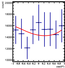
Corrected Yields 3/5 < y < 4/5 , 7\pi/6 < \phi < 8\pi/6
