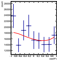
Corrected Yields -4/5 < y < -3/5 , 1\pi/6 < \phi < 2\pi/6
