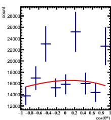
Corrected Yields 1/5 < y < 2/5 , 3\pi/6 < \phi < 4\pi/6
