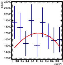
Corrected Yields 0/5 < y < 1/5 , 4\pi/6 < \phi < 5\pi/6
