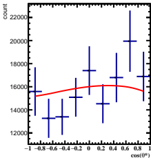
Corrected Yields 1/5 < y < 2/5 , 4\pi/6 < \phi < 5\pi/6
