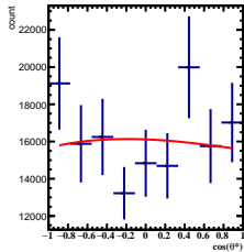
Corrected Yields -1/5 < y < 0/5 , 1\pi/6 < \phi < 2\pi/6
