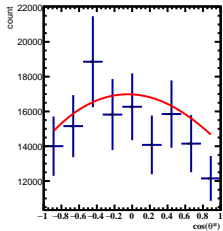
Corrected Yields 0/5 < y < 1/5 , 10\pi/6 < \phi < 11\pi/6
