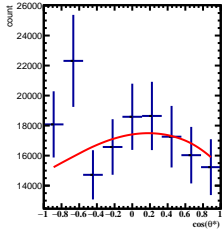
Corrected Yields -2/5 < y < -1/5 , 1\pi/6 < \phi < 2\pi/6
