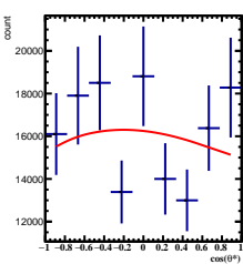
Corrected Yields -2/5 < y < -1/5 , 5\pi/6 < \phi < 6\pi/6
