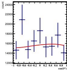
Corrected Yields 2/5 < y < 3/5 , 6\pi/6 < \phi < 7\pi/6
