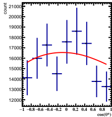
Corrected Yields 1/5 < y < 2/5 , 9\pi/6 < \phi < 10\pi/6
