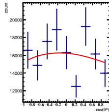
Corrected Yields -2/5 < y < -1/5 , 9\pi/6 < \phi < 10\pi/6
