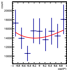
Corrected Yields 3/5 < y < 4/5 , 4\pi/6 < \phi < 5\pi/6
