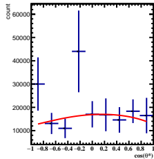
Corrected Yields 4/5 < y < 5/5 , 2\pi/6 < \phi < 3\pi/6
