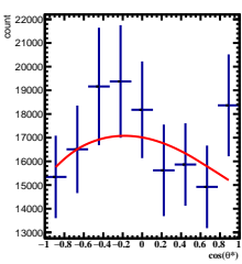
Corrected Yields -2/5 < y < -1/5 , 8\pi/6 < \phi < 9\pi/6
