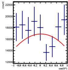
Corrected Yields 0/5 < y < 1/5 , 7\pi/6 < \phi < 8\pi/6
