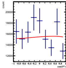
Corrected Yields 2/5 < y < 3/5 , 2\pi/6 < \phi < 3\pi/6
