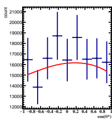
Corrected Yields -3/5 < y < -2/5 , 2\pi/6 < \phi < 3\pi/6
