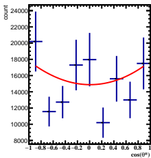
Corrected Yields -4/5 < y < -3/5 , 10\pi/6 < \phi < 11\pi/6
