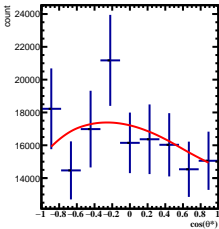
Corrected Yields -3/5 < y < -2/5 , 4\pi/6 < \phi < 5\pi/6
