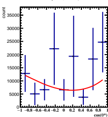
Corrected Yields 4/5 < y < 5/5 , 5\pi/6 < \phi < 6\pi/6
