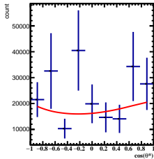
Corrected Yields -5/5 < y < -4/5 , 9\pi/6 < \phi < 10\pi/6
