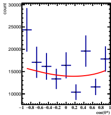
Corrected Yields 3/5 < y < 4/5 , 10\pi/6 < \phi < 11\pi/6
