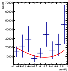
Corrected Yields -5/5 < y < -4/5 , 10\pi/6 < \phi < 11\pi/6
