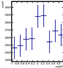
RawYields 3/5 < y < 4/5 , 9\pi/6 < \phi' < 10\pi/6
