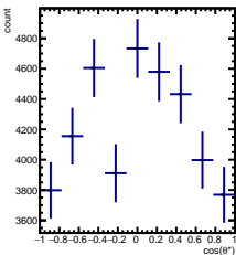
RawYields 1/5 < y < 2/5 , 1\pi/6 < \phi' < 2\pi/6
