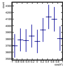
RawYields -3/5 < y < -2/5 , 5\pi/6 < \phi' < 6\pi/6
