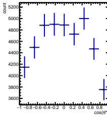
RawYields -2/5 < y < -1/5 , 9\pi/6 < \phi' < 10\pi/6
