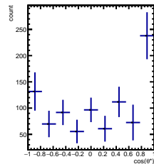
RawYields 4/5 < y < 5/5 , 1\pi/6 < \phi' < 2\pi/6
