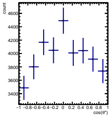
RawYields 0/5 < y < 1/5 , 0\pi/6 < \phi' < 1\pi/6
