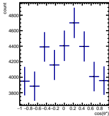
RawYields 1/5 < y < 2/5 , 0\pi/6 < \phi' < 1\pi/6
