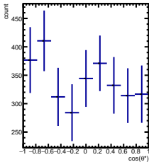
RawYields -5/5 < y < -4/5 , 9\pi/6 < \phi' < 10\pi/6
