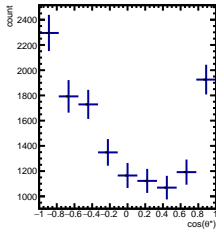
RawYields -4/5 < y < -3/5 , 0\pi/6 < \phi' < 1\pi/6
