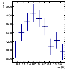
RawYields -2/5 < y < -1/5 , 0\pi/6 < \phi' < 1\pi/6
