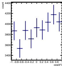
RawYields 2/5 < y < 3/5 , 1\pi/6 < \phi' < 2\pi/6
