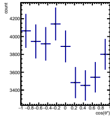
RawYields -3/5 < y < -2/5 , 0\pi/6 < \phi' < 1\pi/6
