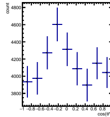
RawYields -1/5 < y < 0/5 , 0\pi/6 < \phi' < 1\pi/6
