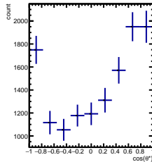
RawYields 3/5 < y < 4/5 , 0\pi/6 < \phi' < 1\pi/6
