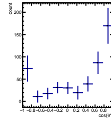
RawYields 4/5 < y < 5/5 , 0\pi/6 < \phi' < 1\pi/6
