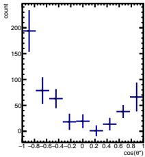
RawYields -5/5 < y < -4/5 , 0\pi/6 < \phi' < 1\pi/6
