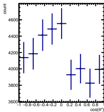
RawYields -3/5 < y < -2/5 , 1\pi/6 < \phi' < 2\pi/6
