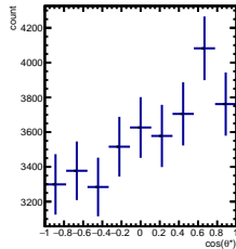
RawYields 2/5 < y < 3/5 , 0\pi/6 < \phi' < 1\pi/6
