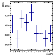
RawYields 2/5 < y < 3/5 , 5\pi/6 < \phi' < 6\pi/6
