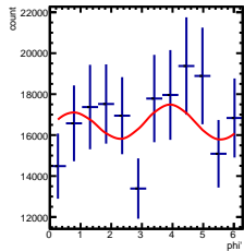
Corrected Yields -2/5 < \gamma < -1/5, -1.5/4.5 < \cos(\theta^*) < -0.5/4.5
