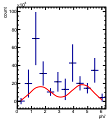
Corrected Yields -5/5 < y < -4/5 , 0.5/4.5 < \cos(\theta^*) < 1.5/4.5
