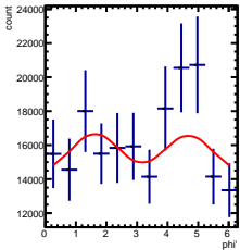
Corrected Yields 0/5 < y < 1/5, 2.5/4.5 < \cos(\theta^*) < 3.5/4.5
