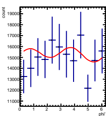
Corrected Yields 2/5 < y < 3/5 , 0.5/4.5 < \cos(\theta^*) < 1.5/4.5
