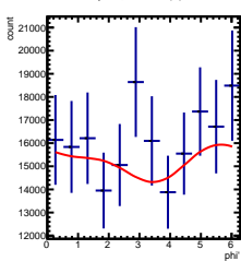
Corrected Yields -3/5 < y < -2/5 , 3.5/4.5 < \cos(\theta^*) < 4.5/4.5
