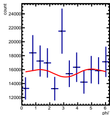
Corrected Yields 1/5 < y < 2/5, -3.5/4.5 < \cos(\theta^*) < -2.5/4.5
