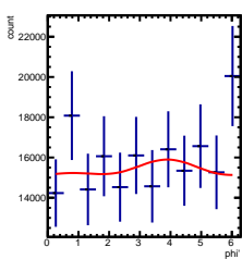
Corrected Yields -2/5 < y < -1/5 , -4.5/4.5 < \cos(\theta^*) < -3.5/4.5
