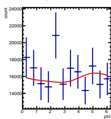
Corrected Yields -1/5 < y < 0/5 , 3.5/4.5 < \cos(\theta^*) < 4.5/4.5
