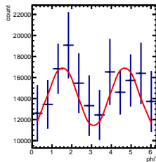
Corrected Yields 3/5 < y < 4/5, -0.5/4.5 < \cos(\theta^*) < 0.5/4.5
