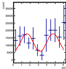
Corrected Yields 4/5 < y < 5/5, -0.5/4.5 < \cos(\theta^*) < 0.5/4.5
