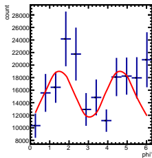
Corrected Yields -4/5 < y < -3/5, -0.5/4.5 < \cos(\theta^*) < 0.5/4.5
