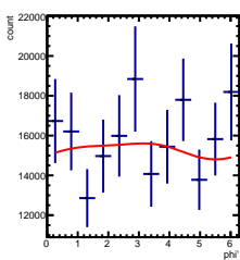
Corrected Yields 2/5 < y < 3/5 , 3.5/4.5 < \cos(\theta^*) < 4.5/4.5
