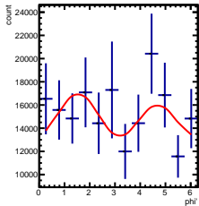
Corrected Yields 3/5 < y < 4/5, 2.5/4.5 < \cos(\theta^*) < 3.5/4.5
