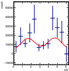
Corrected Yields 4/5 < y < 5/5, -2.5/4.5 < \cos(\theta^*) < -1.5/4.5
