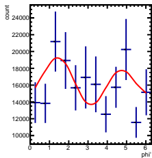
Corrected Yields -4/5 < y < -3/5, -3.5/4.5 < \cos(\theta^*) < -2.5/4.5
