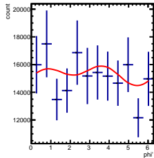
Corrected Yields 2/5 < y < 3/5, 1.5/4.5 < \cos(\theta^*) < 2.5/4.5
