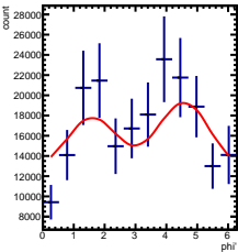
Corrected Yields -4/5 < y < -3/5, 2.5/4.5 < \cos(\theta^*) < 3.5/4.5
