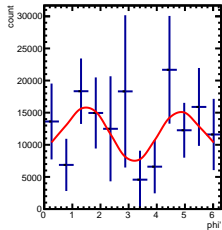
Corrected Yields 4/5 < y < 5/5, 2.5/4.5 < \cos(\theta^*) < 3.5/4.5
