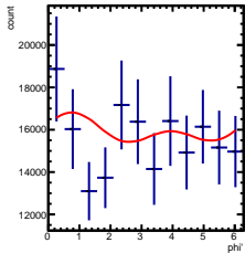
Corrected Yields -2/5 < y < -1/5, 2.5/4.5 < \cos(\theta^*) < 3.5/4.5
