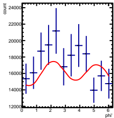
Corrected Yields -3/5 < \gamma < -2/5, -1.5/4.5 < \cos(\theta^*) < -0.5/4.5
