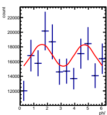
Corrected Yields 0/5 < y < 1/5 , 0.5/4.5 < \cos(\theta^*) < 1.5/4.5
