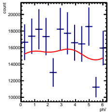
Corrected Yields 2/5 < y < 3/5, 2.5/4.5 < \cos(\theta^*) < 3.5/4.5
