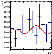
Corrected Yields -2/5 < y < -1/5, -2.5/4.5 < \cos(\theta^*) < -1.5/4.5
