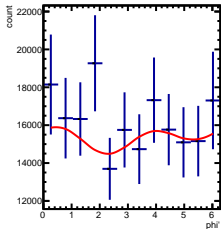
Corrected Yields 2/5 < y < 3/5, -2.5/4.5 < \cos(\theta^*) < -1.5/4.5
