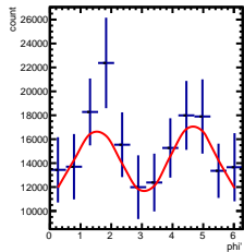
Corrected Yields 3/5 < \gamma < 4/5, -1.5/4.5 < \cos(\theta^*) < -0.5/4.5
