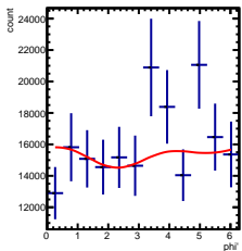
Corrected Yields 2/5 < y < 3/5, -3.5/4.5 < \cos(\theta^*) < -2.5/4.5
