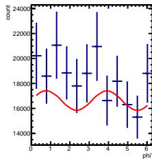
Corrected Yields -2/5 < y < -1/5, -0.5/4.5 < \cos(\theta^*) < 0.5/4.5
