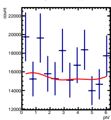
Corrected Yields -2/5 < y < -1/5 , 3.5/4.5 < \cos(\theta^*) < 4.5/4.5
