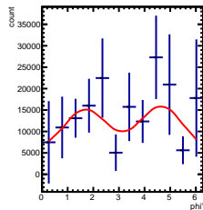
Corrected Yields 4/5 < y < 5/5, -3.5/4.5 < \cos(\theta^*) < -2.5/4.5
