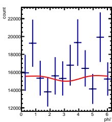
Corrected Yields 1/5 < y < 2/5 , -4.5/4.5 < \cos(\theta^*) < -3.5/4.5
