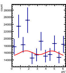
Corrected Yields 1/5 < y < 2/5 , 0.5/4.5 < \cos(\theta^*) < 1.5/4.5
