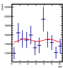
Corrected Yields 0/5 < y < 1/5 , 3.5/4.5 < \cos(\theta^*) < 4.5/4.5
