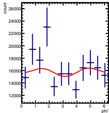
Corrected Yields 1/5 < y < 2/5, -2.5/4.5 < \cos(\theta^*) < -1.5/4.5
