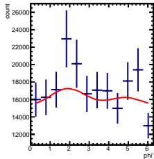
Corrected Yields -1/5 < y < 0/5, -2.5/4.5 < \cos(\theta^*) < -1.5/4.5
