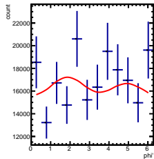
Corrected Yields -1/5 < \gamma < 0/5, -1.5/4.5 < \cos(\theta^*) < -0.5/4.5
