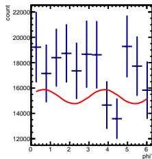
Corrected Yields 2/5 < y < 3/5, -0.5/4.5 < \cos(\theta^*) < 0.5/4.5
