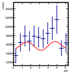
Corrected Yields 0/5 < y < 1/5, -3.5/4.5 < \cos(\theta^*) < -2.5/4.5
