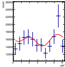
Corrected Yields -3/5 < y < -2/5, 1.5/4.5 < \cos(\theta^*) < 2.5/4.5
