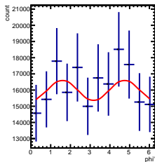
Corrected Yields 1/5 < y < 2/5, -0.5/4.5 < \cos(\theta^*) < 0.5/4.5
