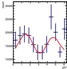
Corrected Yields -4/5 < y < -3/5, -2.5/4.5 < \cos(\theta^*) < -1.5/4.5
