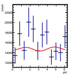
Corrected Yields 0/5 < y < 1/5 , -4.5/4.5 < \cos(\theta^*) < -3.5/4.5
