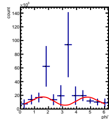
Corrected Yields 4/5 < y < 5/5 , 0.5/4.5 < \cos(\theta^*) < 1.5/4.5
