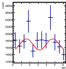
Corrected Yields 0/5 < y < 1/5, -0.5/4.5 < \cos(\theta^*) < 0.5/4.5
