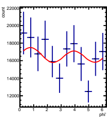
Corrected Yields -2/5 < y < -1/5 , 0.5/4.5 < \cos(\theta^*) < 1.5/4.5
