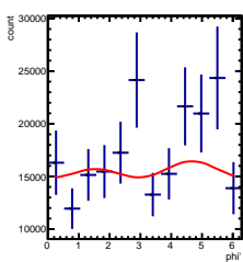
Corrected Yields 3/5 < y < 4/5 , -4.5/4.5 < \cos(\theta^*) < -3.5/4.5
