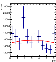
Corrected Yields 1/5 < y < 2/5 , 3.5/4.5 < \cos(\theta^*) < 4.5/4.5
