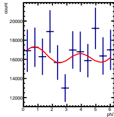
Corrected Yields -2/5 < y < -1/5, 1.5/4.5 < \cos(\theta^*) < 2.5/4.5
