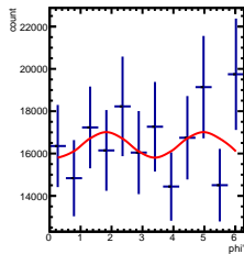
Corrected Yields -1/5 < y < 0/5, -0.5/4.5 < \cos(\theta^*) < 0.5/4.5
