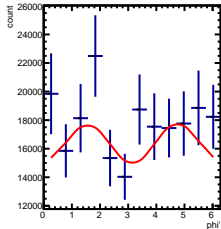
Corrected Yields 0/5 < y < 1/5, -2.5/4.5 < \cos(\theta^*) < -1.5/4.5
