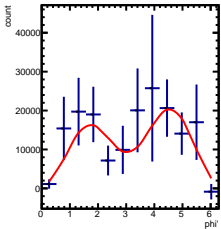
Corrected Yields -5/5 < y < -4/5, 1.5/4.5 < \cos(\theta^*) < 2.5/4.5
