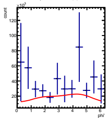
Corrected Yields -5/5 < y < -4/5 , 3.5/4.5 < \cos(\theta^*) < 4.5/4.5
