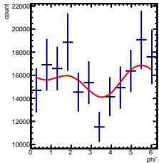
Corrected Yields -3/5 < y < -2/5, 2.5/4.5 < \cos(\theta^*) < 3.5/4.5
