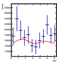
Corrected Yields 3/5 < y < 4/5 , 3.5/4.5 < \cos(\theta^*) < 4.5/4.5
