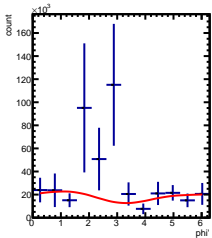
Corrected Yields -5/5 < y < -4/5 , -4.5/4.5 < \cos(\theta^*) < -3.5/4.5
