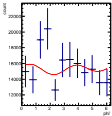
Corrected Yields 2/5 < \gamma < 3/5, -1.5/4.5 < \cos(\theta^*) < -0.5/4.5
