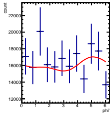
Corrected Yields -1/5 < y < 0/5, 2.5/4.5 < \cos(\theta^*) < 3.5/4.5
