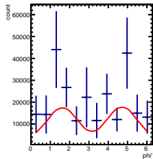
Corrected Yields 4/5 < \gamma < 5/5, -1.5/4.5 < \cos(\theta^*) < -0.5/4.5
