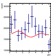
Corrected Yields -4/5 < y < -3/5 , -4.5/4.5 < \cos(\theta^*) < -3.5/4.5
