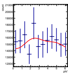
Corrected Yields -3/5 < y < -2/5 , -4.5/4.5 < \cos(\theta^*) < -3.5/4.5
