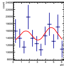
Corrected Yields 3/5 < y < 4/5, -3.5/4.5 < \cos(\theta^*) < -2.5/4.5
