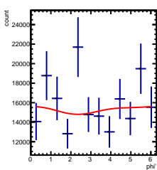
Corrected Yields 2/5 < y < 3/5 , -4.5/4.5 < \cos(\theta^*) < -3.5/4.5
