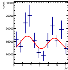
Corrected Yields 3/5 < y < 4/5, 1.5/4.5 < \cos(\theta^*) < 2.5/4.5
