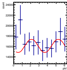
Corrected Yields -3/5 < y < -2/5, -0.5/4.5 < \cos(\theta^*) < 0.5/4.5
