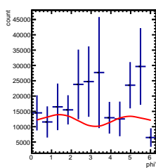
Corrected Yields 4/5 < y < 5/5 , 3.5/4.5 < \cos(\theta^*) < 4.5/4.5
