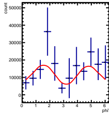
Corrected Yields 4/5 < y < 5/5, 1.5/4.5 < \cos(\theta^*) < 2.5/4.5
