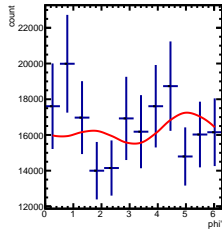
Corrected Yields -1/5 < y < 0/5, 1.5/4.5 < \cos(\theta^*) < 2.5/4.5
