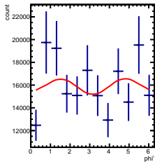
Corrected Yields 1/5 < \gamma < 2/5, -1.5/4.5 < \cos(\theta^*) < -0.5/4.5
