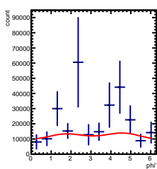
Corrected Yields 4/5 < y < 5/5 , -4.5/4.5 < \cos(\theta^*) < -3.5/4.5
