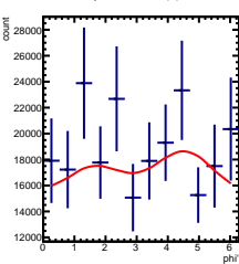
Corrected Yields -4/5 < y < -3/5 , 3.5/4.5 < \cos(\theta^*) < 4.5/4.5
