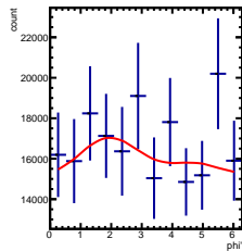
Corrected Yields -1/5 < y < 0/5, -3.5/4.5 < \cos(\theta^*) < -2.5/4.5
