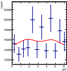
Corrected Yields 1/5 < y < 2/5, 2.5/4.5 < \cos(\theta^*) < 3.5/4.5
