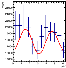
Corrected Yields -4/5 < \gamma < -3/5, -1.5/4.5 < \cos(\theta^*) < -0.5/4.5
