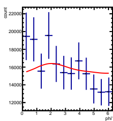
Corrected Yields -1/5 < y < 0/5 , -4.5/4.5 < \cos(\theta^*) < -3.5/4.5
