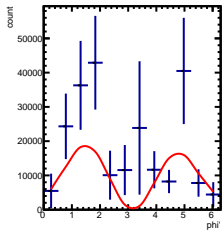
Corrected Yields -5/5 < \gamma < -4/5, -1.5/4.5 < \cos(\theta^*) < -0.5/4.5
