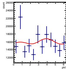
Corrected Yields -2/5 < y < -1/5, -3.5/4.5 < \cos(\theta^*) < -2.5/4.5
