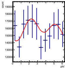
Corrected Yields -3/5 < y < -2/5, -2.5/4.5 < \cos(\theta^*) < -1.5/4.5
