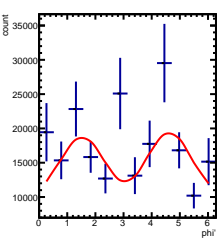
Corrected Yields -4/5 < y < -3/5 , 0.5/4.5 < \cos(\theta^*) < 1.5/4.5
