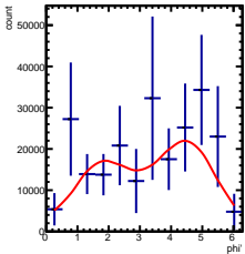
Corrected Yields -5/5 < y < -4/5, 2.5/4.5 < \cos(\theta^*) < 3.5/4.5
