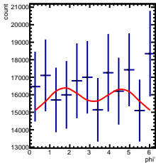
Corrected Yields 1/5 < y < 2/5, 1.5/4.5 < \cos(\theta^*) < 2.5/4.5
