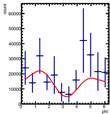
Corrected Yields -5/5 < y < -4/5, -3.5/4.5 < \cos(\theta^*) < -2.5/4.5
