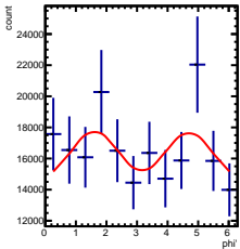
Corrected Yields 0/5 < y < 1/5, 1.5/4.5 < \cos(\theta^*) < 2.5/4.5
