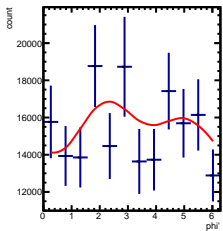
Corrected Yields -3/5 < y < -2/5, -3.5/4.5 < \cos(\theta^*) < -2.5/4.5
