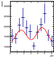
Corrected Yields -4/5 < y < -3/5, 1.5/4.5 < \cos(\theta^*) < 2.5/4.5
