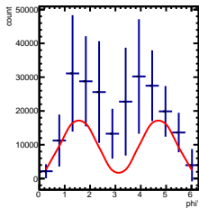
Corrected Yields -5/5 < y < -4/5, -0.5/4.5 < \cos(\theta^*) < 0.5/4.5
