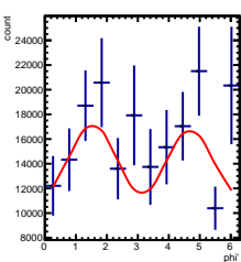
Corrected Yields 3/5 < y < 4/5 , 0.5/4.5 < \cos(\theta^*) < 1.5/4.5
