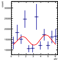
Corrected Yields 3/5 < y < 4/5, -2.5/4.5 < \cos(\theta^*) < -1.5/4.5
