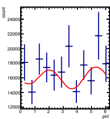
Corrected Yields -3/5 < y < -2/5 , 0.5/4.5 < \cos(\theta^*) < 1.5/4.5
