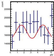
Corrected Yields 0/5 < \gamma < 1/5, -1.5/4.5 < \cos(\theta^*) < -0.5/4.5
