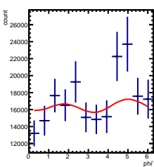
Corrected Yields -1/5 < y < 0/5 , 0.5/4.5 < \cos(\theta^*) < 1.5/4.5
