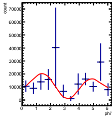
Corrected Yields -5/5 < y < -4/5, -2.5/4.5 < \cos(\theta^*) < -1.5/4.5
