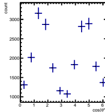
Raw Yields 3/5 < y < 4/5, 0.5/4.5 < \cos(\theta^*) < 1.5/4.5
