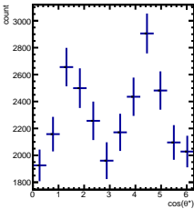
Raw Yields -4/5 < y < -3/5 , 3.5/4.5 < \cos(\theta^*) < 4.5/4.5
