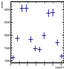
Raw Yields -4/5 < y < -3/5, 0.5/4.5 < \cos(\theta^*) < 1.5/4.5
