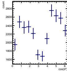
Raw Yields 3/5 < y < 4/5 , 3.5/4.5 < \cos(\theta^*) < 4.5/4.5
