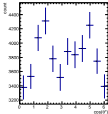
Raw Yields 2/5 < y < 3/5 , -3.5/4.5 < \cos(\theta^*) < -2.5/4.5
