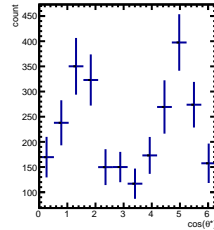
Raw Yields 4/5 < y < 5/5 , 3.5/4.5 < \cos(\theta^*) < 4.5/4.5
