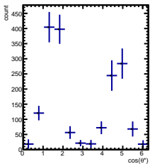
Raw Yields -6/5 < y < -4/5, -1.5/4.5 < \cos(\theta^*) < -0.5/4.5
