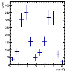
Raw Yields -5/5 < y < -4/5 , 2.5/4.5 < \cos(\theta^*) < 3.5/4.5
