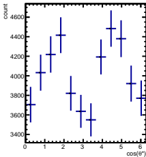
Raw Yields 2/5 < y < 3/5, 1.5/4.5 < \cos(\theta^*) < 2.5/4.5
