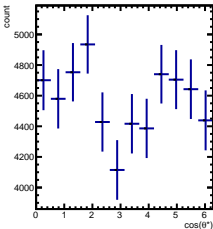
Raw Yields 1/5 < y < 2/5, 0.5/4.5 < \cos(\theta^*) < 1.5/4.5
