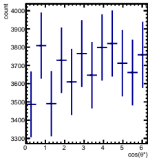
Raw Yields 0/5 < y < 1/5, -4.5/4.5 < \cos(\theta^*) < -3.5/4.5
