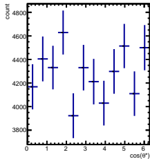
Raw Yields 0/5 < y < 1/5 , -2.5/4.5 < \cos(\theta^*) < -1.5/4.5
