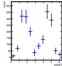
Raw Yields 4/5 < y < 5/5 , -3.5/4.5 < \cos(\theta^*) < -2.5/4.5
