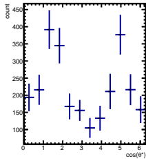
Raw Yields -6/5 < y < -4/5, -4.5/4.5 < \cos(\theta^*) < -3.5/4.5
