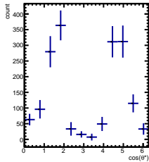
Raw Yields -6/5 < y < -4/5 , -2.5/4.5 < \cos(\theta^*) < -1.5/4.5
