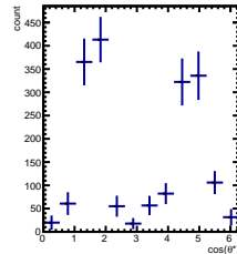
Raw Yields 4/5 < y < 5/5, 0.5/4.5 < \cos(\theta^*) < 1.5/4.5
