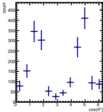
Raw Yields -6/5 < y < -4/5 , -3.5/4.5 < \cos(\theta^*) < -2.5/4.5
