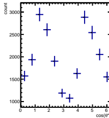
Raw Yields 3/5 < y < 4/5, 1.5/4.5 < \cos(\theta^*) < 2.5/4.5
