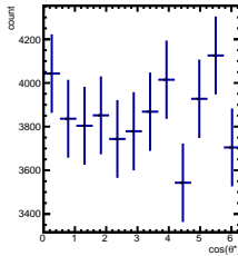
Raw Yields -1/5 < y < 0/5 , 3.5/4.5 < \cos(\theta^*) < 4.5/4.5
