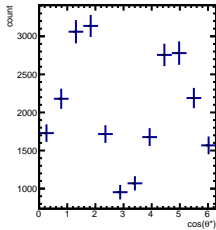
Raw Yields -4/5 < y < -3/5 , -2.5/4.5 < \cos(\theta^*) < -1.5/4.5
