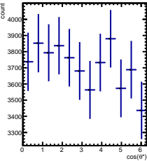
Raw Yields 0/5 < y < 1/5 , 3.5/4.5 < \cos(\theta^*) < 4.5/4.5
