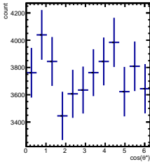
Raw Yields 2/5 < y < 3/5 , 3.5/4.5 < \cos(\theta^*) < 4.5/4.5
