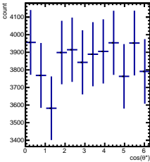
Raw Yields 1/5 < y < 2/5 , 3.5/4.5 < \cos(\theta^*) < 4.5/4.5
