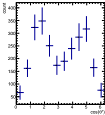
Raw Yields -5/5 < y < -4/5 , 3.5/4.5 < \cos(\theta^*) < 4.5/4.5
