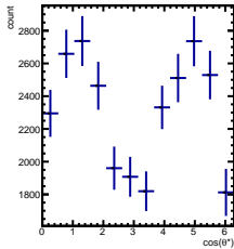
Raw Yields -4/5 < y < -3/5, -4.5/4.5 < \cos(\theta^*) < -3.5/4.5
