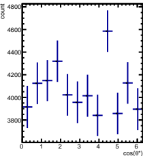
Raw Yields 0/5 < y < 1/5 , 2.5/4.5 < \cos(\theta^*) < 3.5/4.5
