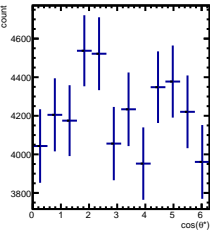
Raw Yields 0/5 < y < 1/5, 1.5/4.5 < \cos(\theta^*) < 2.5/4.5
