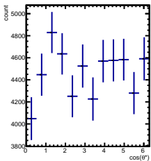
Raw Yields 0/5 < y < 1/5, -1.5/4.5 < \cos(\theta^*) < -0.5/4.5
