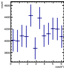
Raw Yields 1/5 < y < 2/5 , 2.5/4.5 < \cos(\theta^*) < 3.5/4.5
