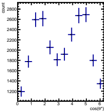
Raw Yields -4/5 < y < -3/5 , 2.5/4.5 < \cos(\theta^*) < 3.5/4.5
