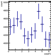
Raw Yields 1/5 < y < 2/5, 1.5/4.5 < \cos(\theta^*) < 2.5/4.5
