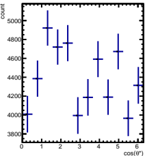
Raw Yields 0/5 < y < 1/5, 0.5/4.5 < \cos(\theta^*) < 1.5/4.5
