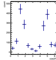
Raw Yields 4/5 < y < 5/5, 1.5/4.5 < \cos(\theta^*) < 2.5/4.5
