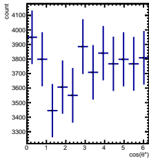
Raw Yields 1/5 < y < 2/5, -4.5/4.5 < \cos(\theta^*) < -3.5/4.5
