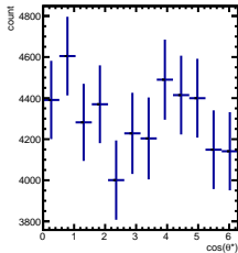
Raw Yields 1/5 < y < 2/5 , -2.5/4.5 < \cos(\theta^*) < -1.5/4.5
