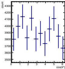
Raw Yields -3/5 < y < -2/5 , 3.5/4.5 < \cos(\theta^*) < 4.5/4.5
