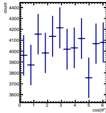
Raw Yields -2/5 < y < -1/5 , 3.5/4.5 < \cos(\theta^*) < 4.5/4.5
