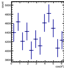
Raw Yields -2/5 < y < -1/5 , -3.5/4.5 < \cos(\theta^*) < -2.5/4.5
