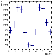
Raw Yields -4/5 < y < -3/5 , -3.5/4.5 < \cos(\theta^*) < -2.5/4.5
