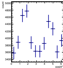
Raw Yields 2/5 < y < 3/5, 0.5/4.5 < \cos(\theta^*) < 1.5/4.5
