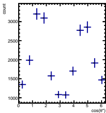
Raw Yields -4/5 < y < -3/5, -1.5/4.5 < \cos(\theta^*) < -0.5/4.5
