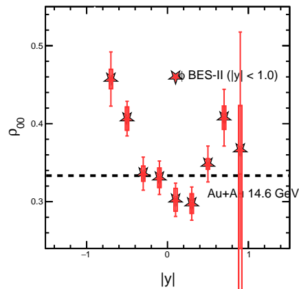
1.00 <math>p_T < 2.00 </math> GeV/c, Cent (0-10)
