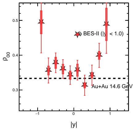
2.00 <math>p_T < 5.00 </math> GeV/c, Cent (10-40)
