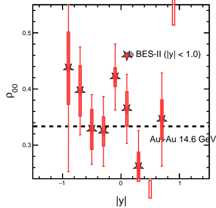
2.00 <math>p_T < 5.00 </math> GeV/c, Cent (0-10)
