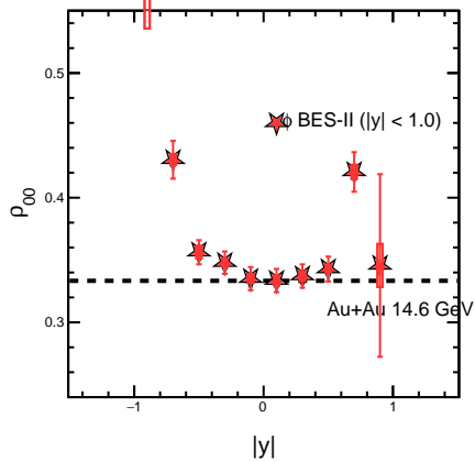
1.00 <math>p_T < 2.00 </math> GeV/c, Cent (10-40)
