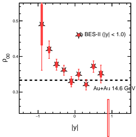
2.00 <math>p_T < 5.00 </math> GeV/c, Cent (40-80)
