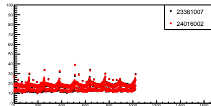
g_ranStdDev_27_1
