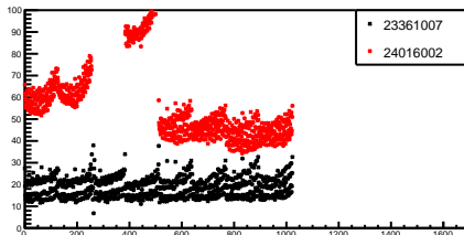
g_totStdDev_25_0
