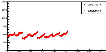
g_pedestals_5_0
