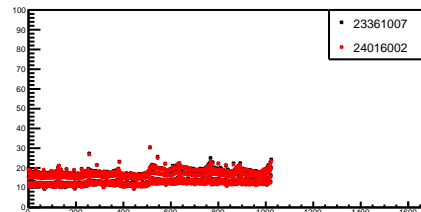
g_ranStdDev_15_2
