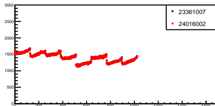
g_pedestals_11_0
