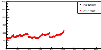
g_pedestals_17_1
