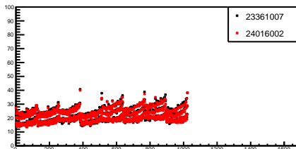
g_totStdDev_11_0
