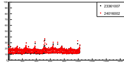
g_ranStdDev_33_0
