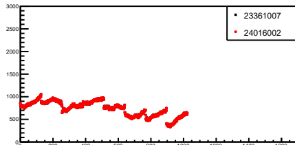
g_pedestals_10_1
