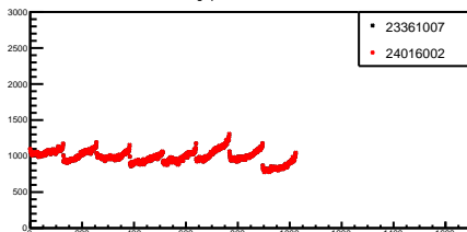
g_pedestals_23_1
