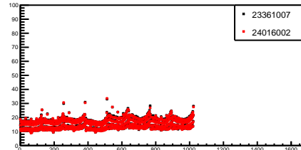
g_ranStdDev_17_1
