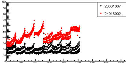
g_totStdDev_33_1
