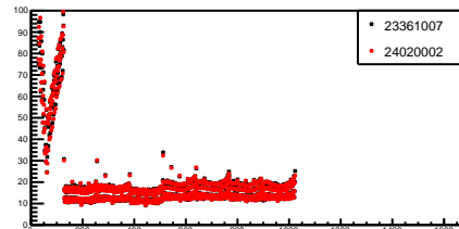
g_randStdDev_27_2
