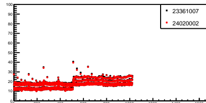
g_randStdDev_26_2
