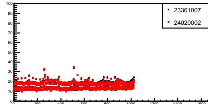
g_randStdDev_25_2
