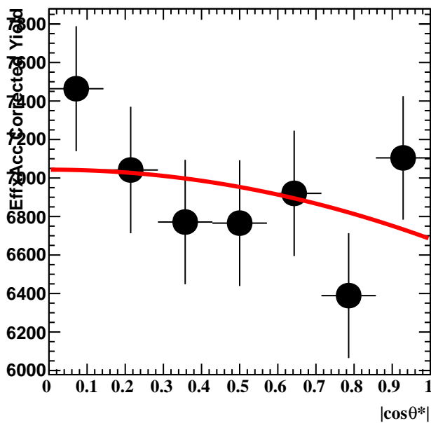
3.0 < p_T < 4.2 GeV/c, Cent 20-60
