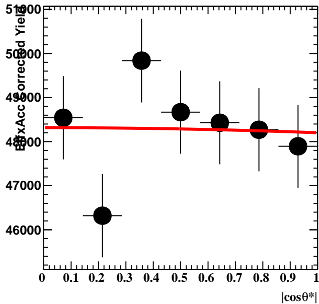
2.4 < p_T < 3.0 GeV/c, Cent 20-60
