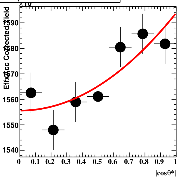
1.2 < p_T < 1.8 GeV/c, Cent 20-60
